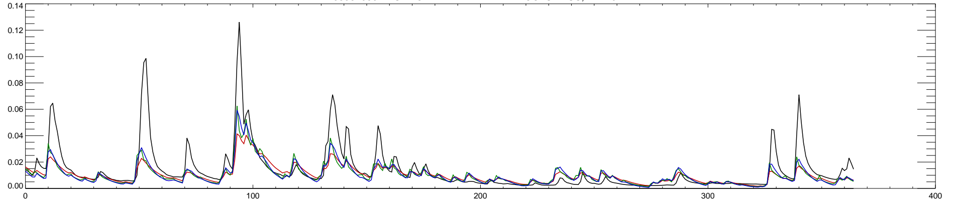
03364000 EAST FORK WHITE RIVER AT COLUMBUS, IN : 2015
