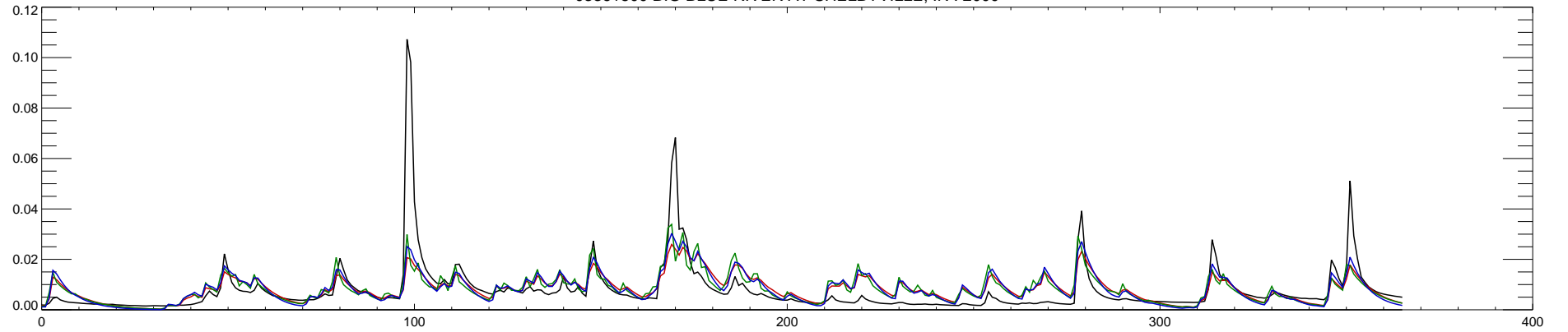
03361500 BIG BLUE RIVER AT SHELBYVILLE, IN : 2001
