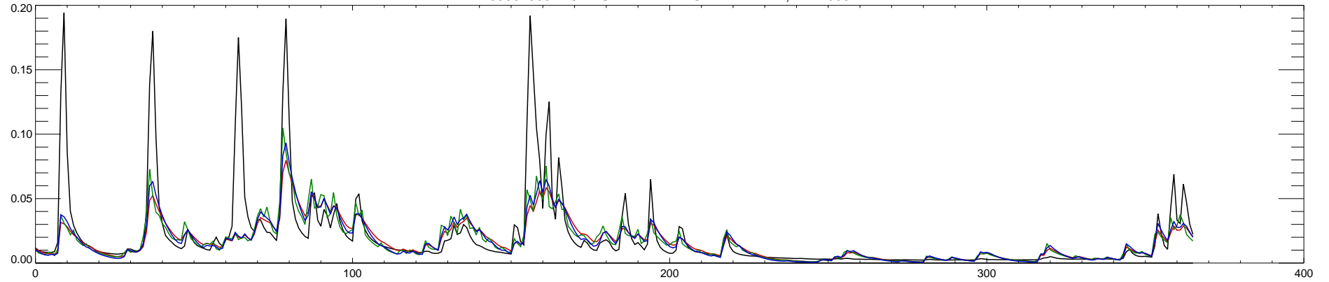
03361500 BIG BLUE RIVER AT SHELBYVILLE, IN : 2009
