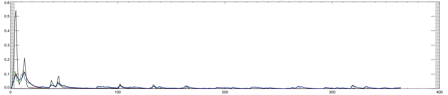
03346000 NORTH FORK EMBARRAS RIVER NEAR OBLONG, IL : 2006
