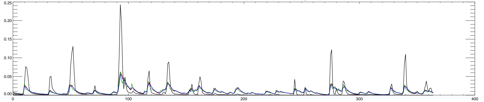
03346000 NORTH FORK EMBARRAS RIVER NEAR OBLONG, IL : 2015
