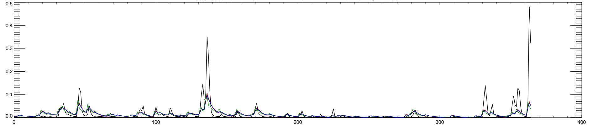
03346000 NORTH FORK EMBARRAS RIVER NEAR OBLONG, IL : 1991
