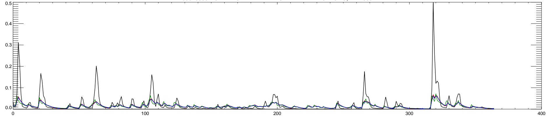
03346000 NORTH FORK EMBARRAS RIVER NEAR OBLONG, IL : 1994
