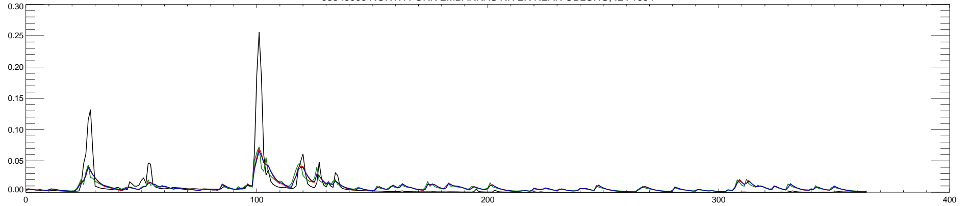
03346000 NORTH FORK EMBARRAS RIVER NEAR OBLONG, IL : 1995
