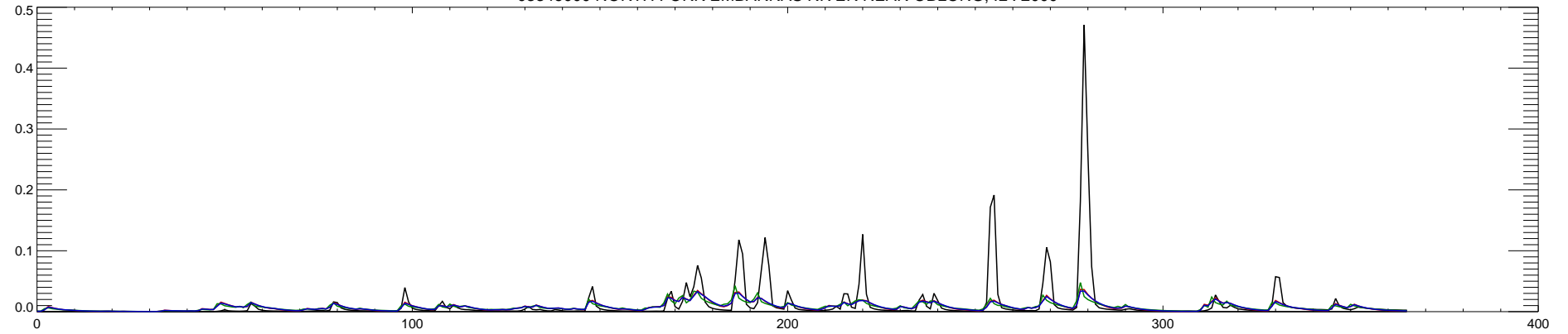
03346000 NORTH FORK EMBARRAS RIVER NEAR OBLONG, IL : 2001
