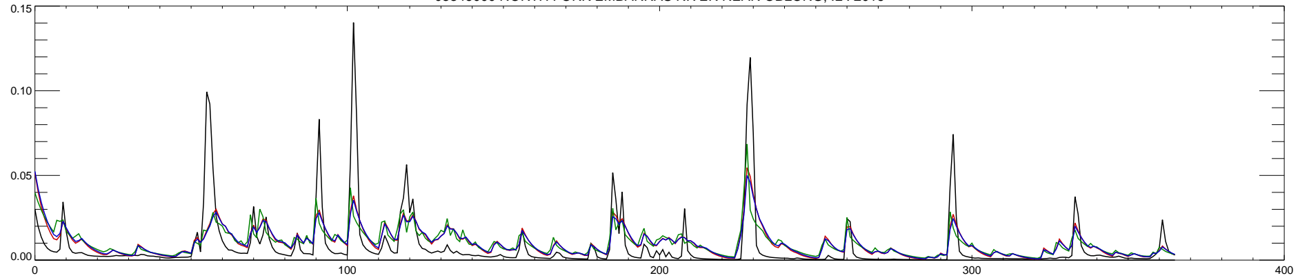
03346000 NORTH FORK EMBARRAS RIVER NEAR OBLONG, IL : 2016
