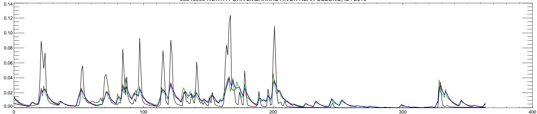
03346000 NORTH FORK EMBARRAS RIVER NEAR OBLONG, IL : 2010
