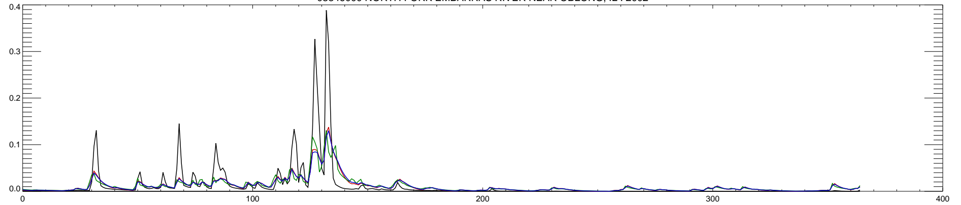
03346000 NORTH FORK EMBARRAS RIVER NEAR OBLONG, IL : 2003
