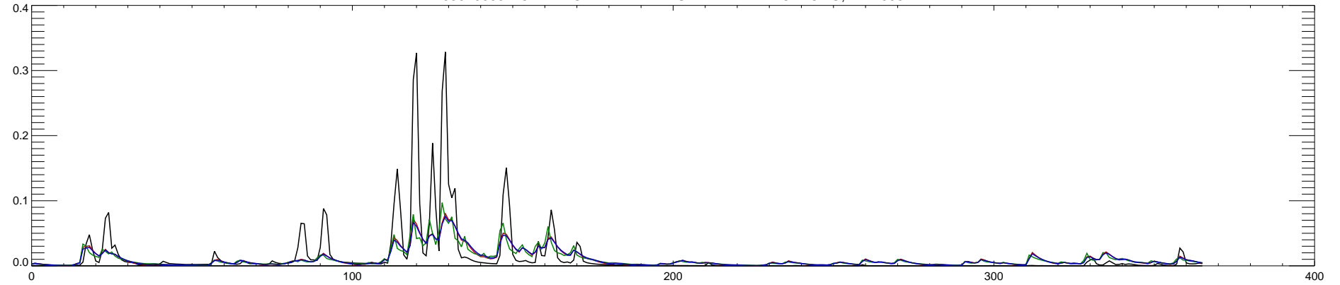
03346000 NORTH FORK EMBARRAS RIVER NEAR OBLONG, IL : 1997
