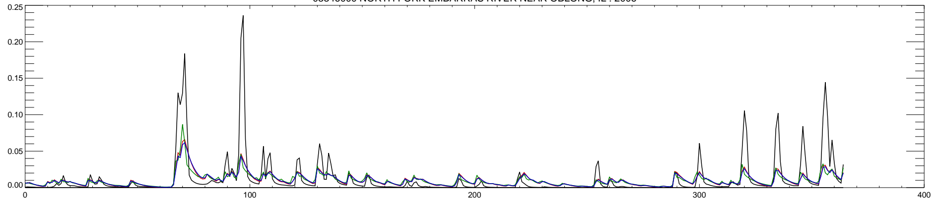
03346000 NORTH FORK EMBARRAS RIVER NEAR OBLONG, IL : 2007
