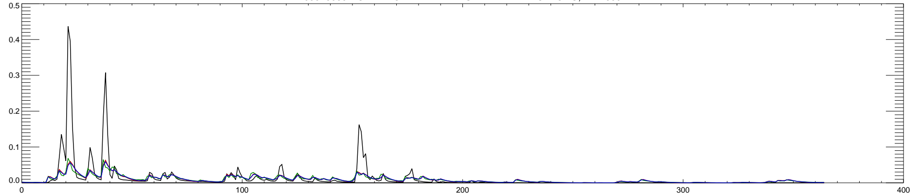
03346000 NORTH FORK EMBARRAS RIVER NEAR OBLONG, IL : 2000
