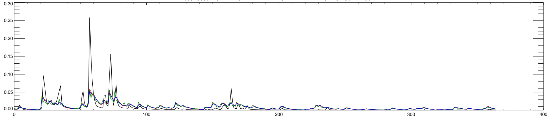
03346000 NORTH FORK EMBARRAS RIVER NEAR OBLONG, IL : 1998
