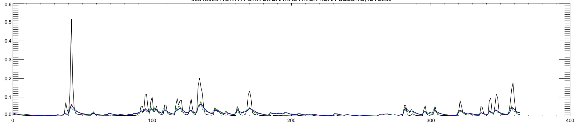
03346000 NORTH FORK EMBARRAS RIVER NEAR OBLONG, IL : 2010
