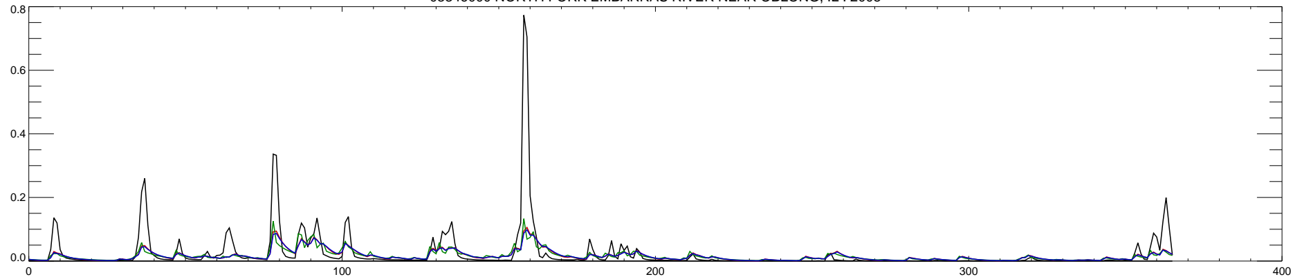
03346000 NORTH FORK EMBARRAS RIVER NEAR OBLONG, IL : 2009
