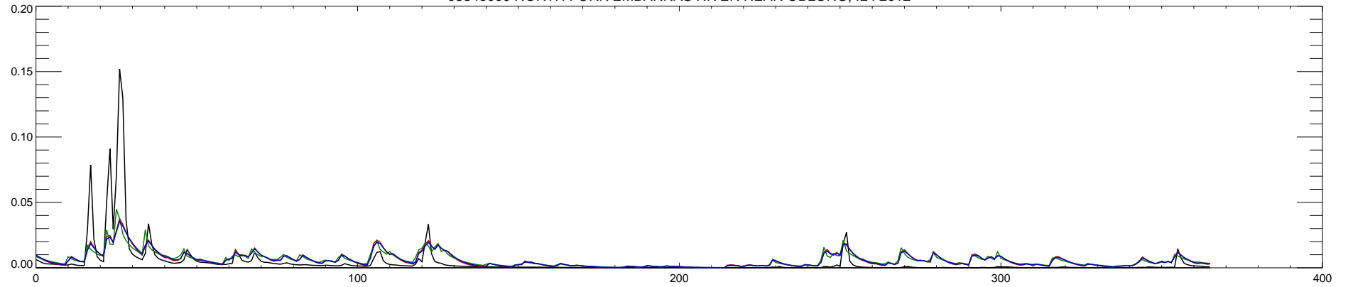
03346000 NORTH FORK EMBARRAS RIVER NEAR OBLONG, IL : 2013
