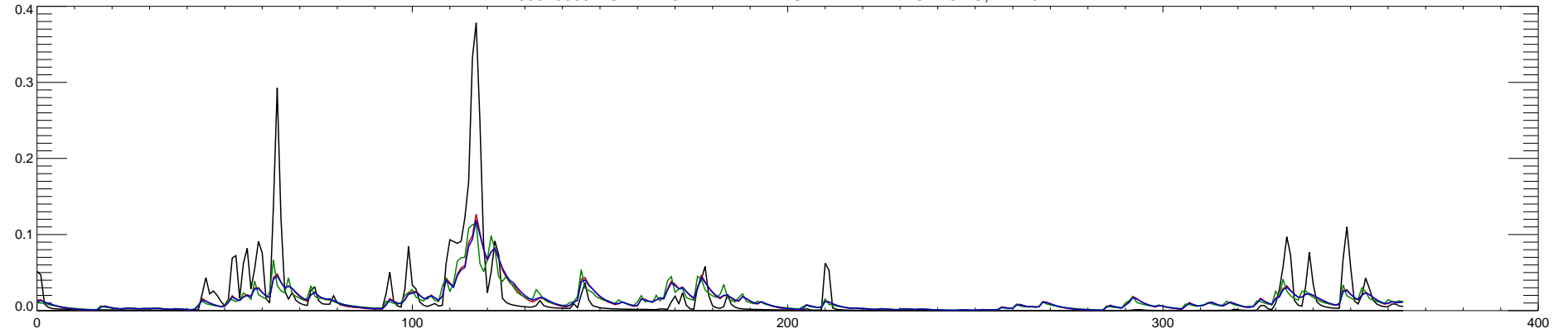
03346000 NORTH FORK EMBARRAS RIVER NEAR OBLONG, IL : 2012
