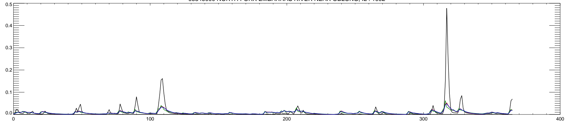
03346000 NORTH FORK EMBARRAS RIVER NEAR OBLONG, IL : 1992
