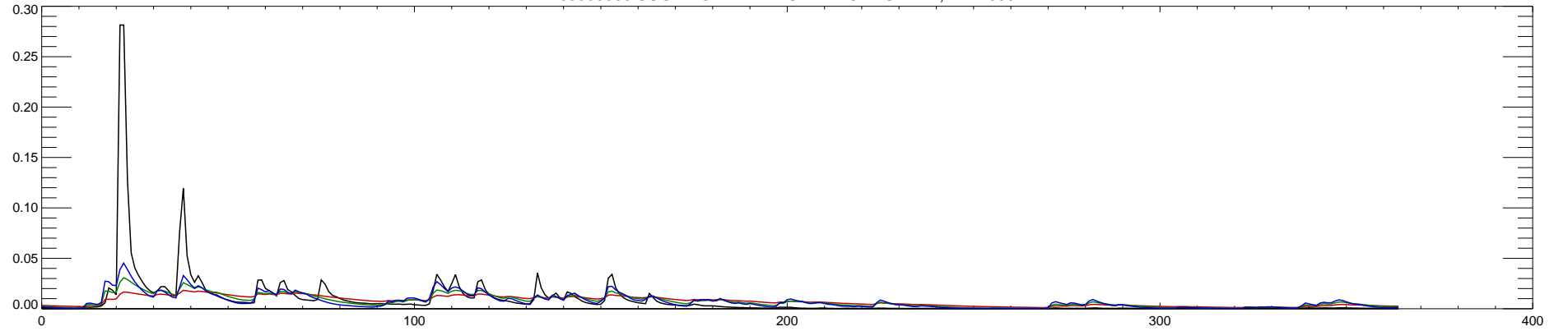
03339500 SUGAR CREEK AT CRAWFORDSVILLE, IN : 2000
