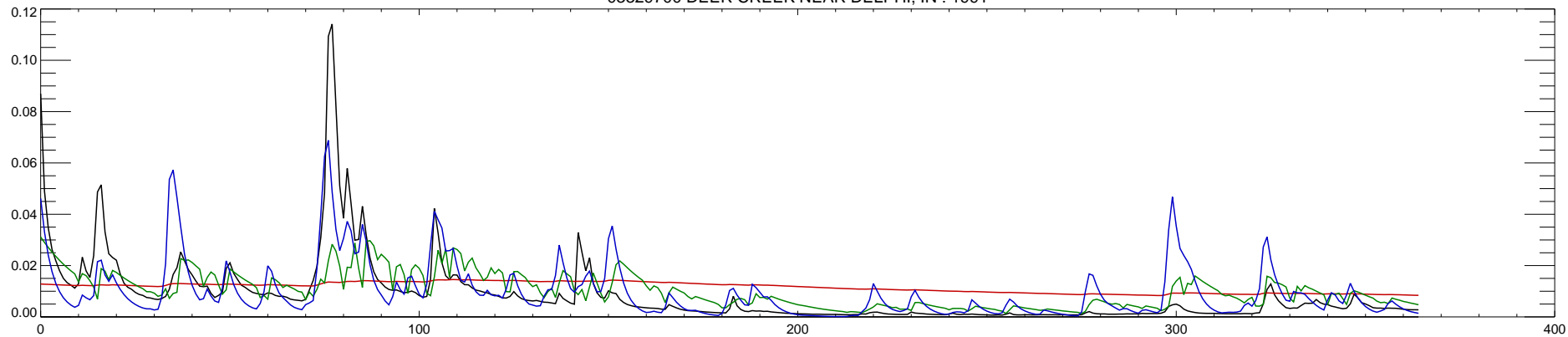
03329700 DEER CREEK NEAR DELPHI, IN : 1992
