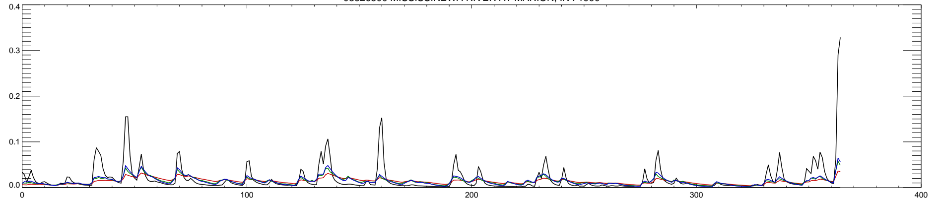
03326500 MISSISSINEWA RIVER AT MARION, IN : 1991
