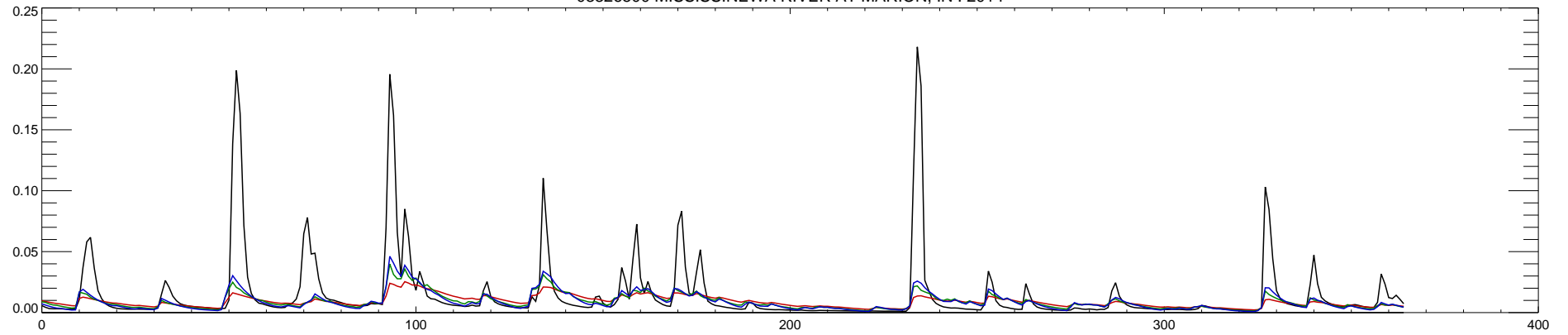
03326500 MISSISSINEWA RIVER AT MARION, IN : 2015
