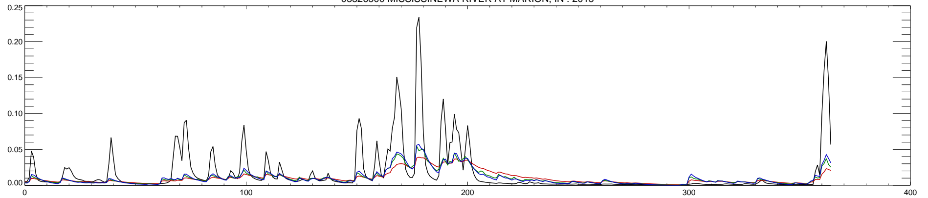
03326500 MISSISSINEWA RIVER AT MARION, IN : 2016
