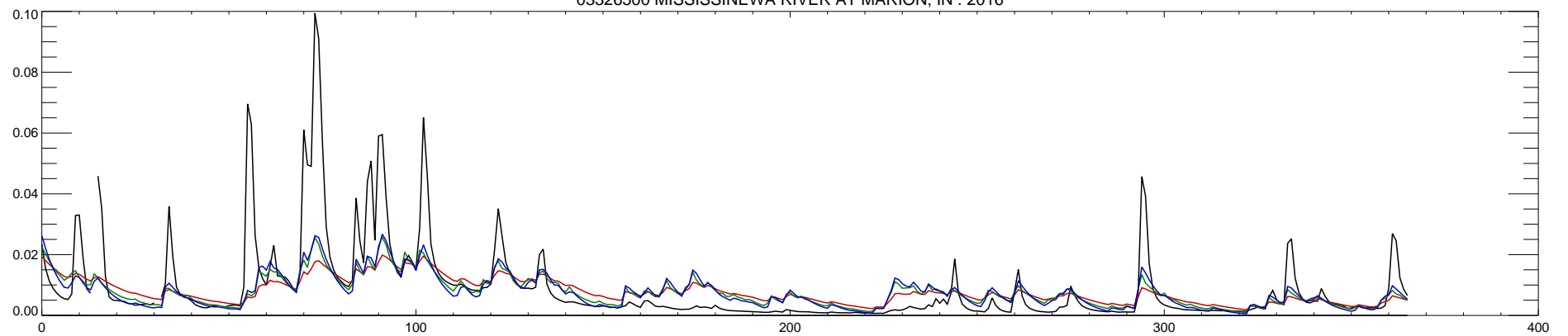
03326500 MISSISSINEWA RIVER AT MARION, IN : 2016
