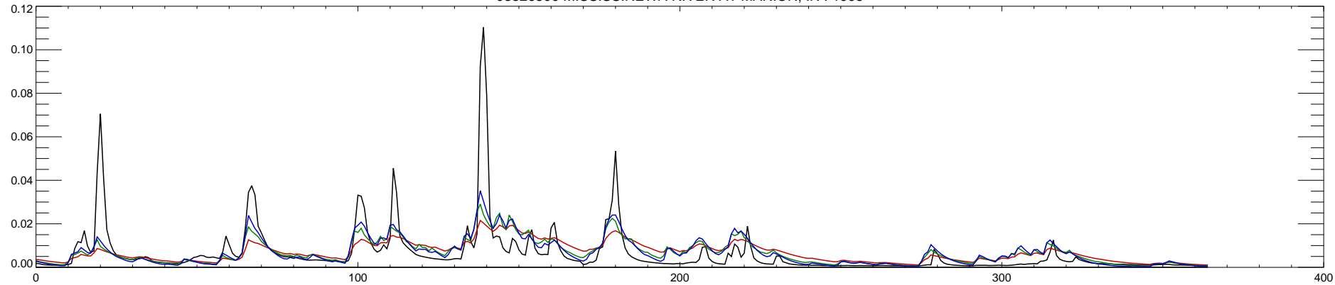
03326500 MISSISSINEWA RIVER AT MARION, IN : 1995
