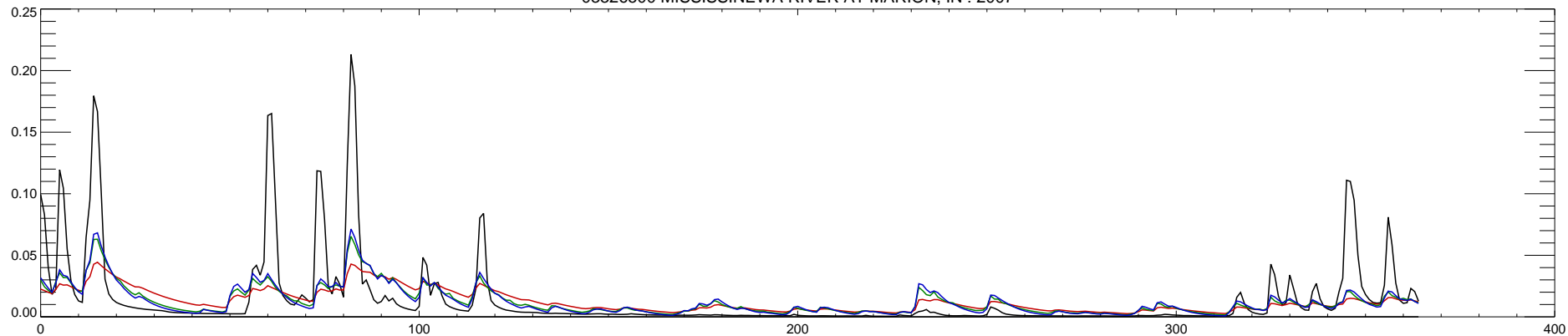
03326500 MISSISSINEWA RIVER AT MARION, IN : 2007
