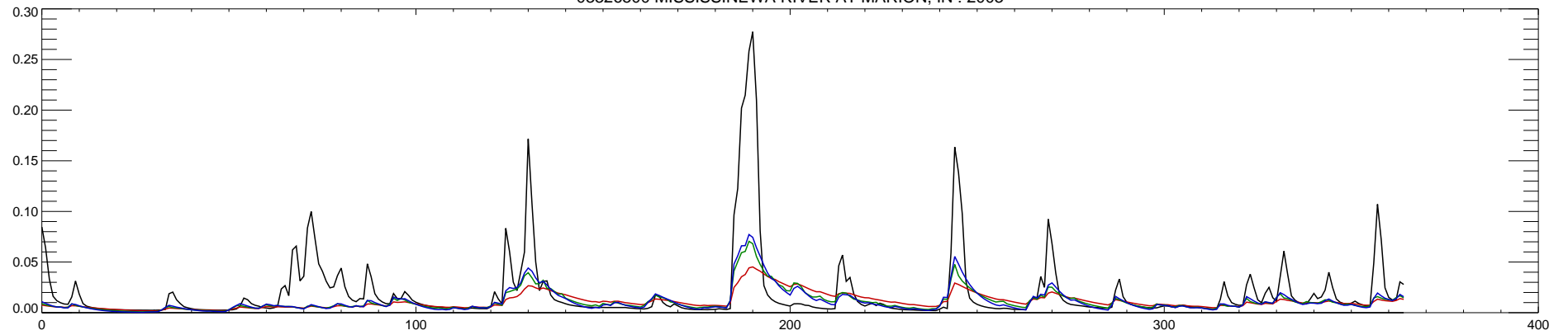
03326500 MISSISSINEWA RIVER AT MARION, IN : 2004
