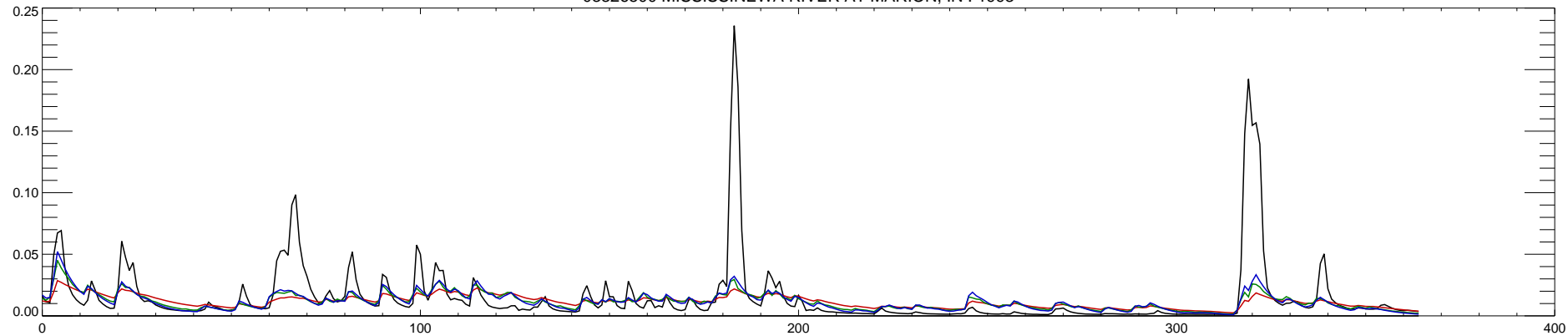
03326500 MISSISSINEWA RIVER AT MARION, IN : 1994
