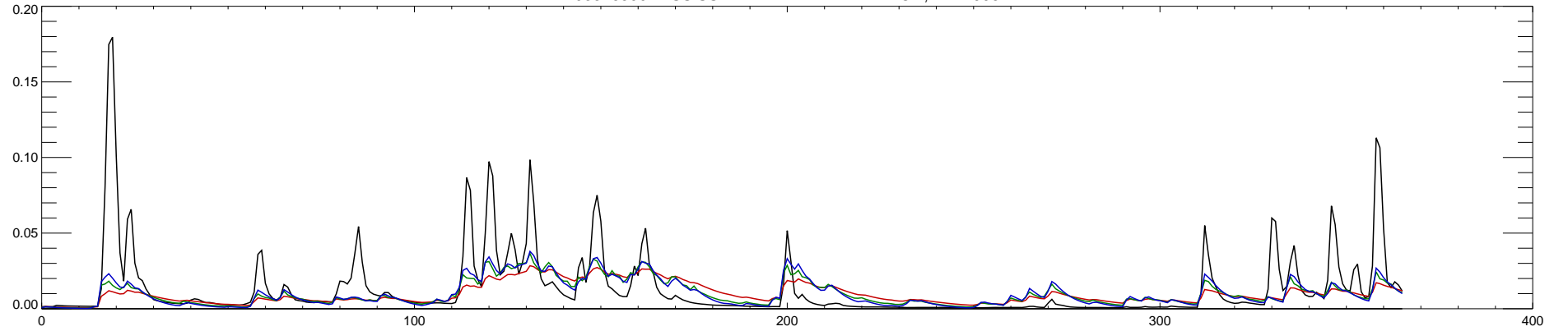
03326500 MISSISSINEWA RIVER AT MARION, IN : 1997
