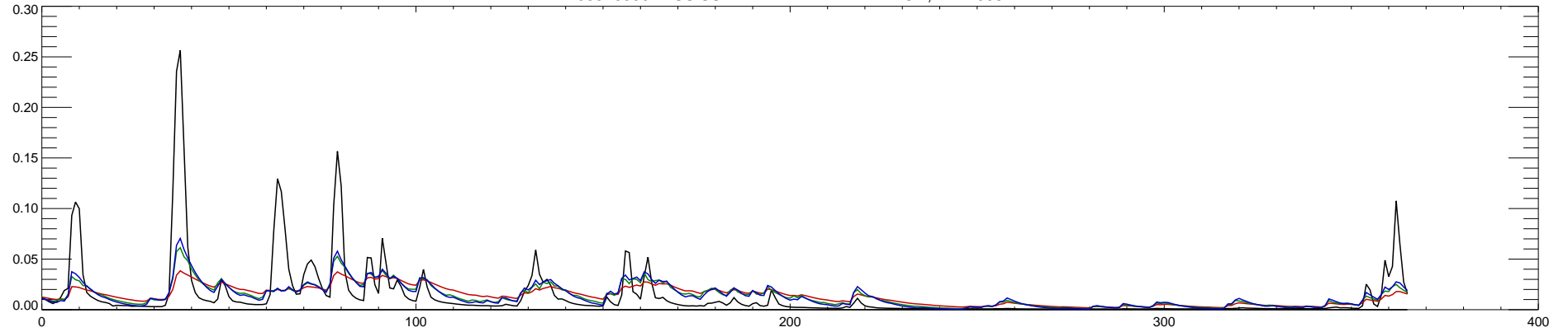
03326500 MISSISSINEWA RIVER AT MARION, IN : 2009
