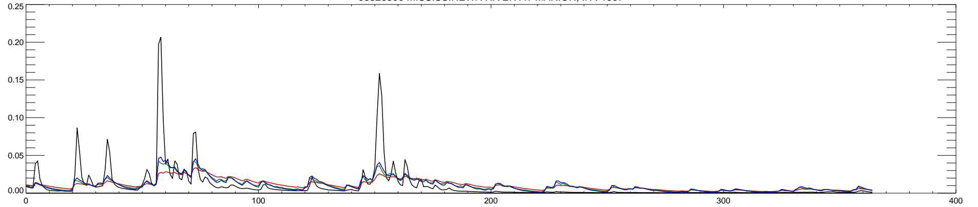
03326500 MISSISSINEWA RIVER AT MARION, IN : 1998
