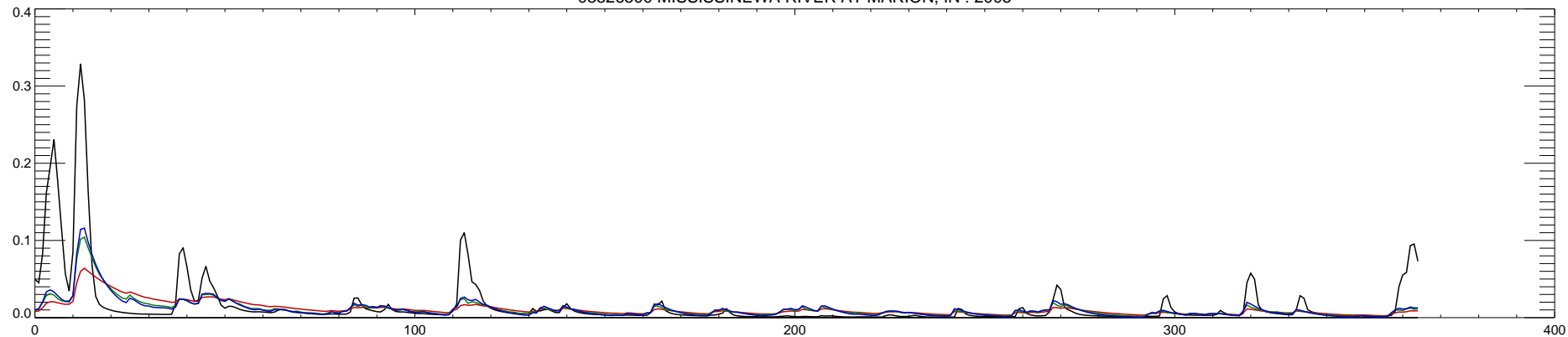
03326500 MISSISSINEWA RIVER AT MARION, IN : 2006
