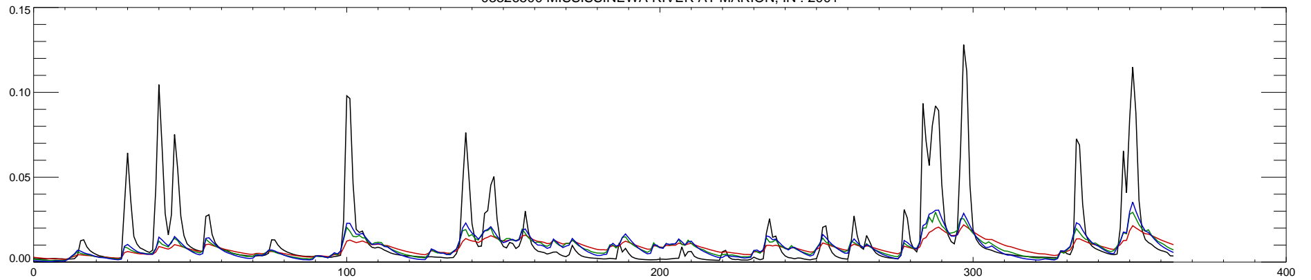
03326500 MISSISSINEWA RIVER AT MARION, IN : 2001
