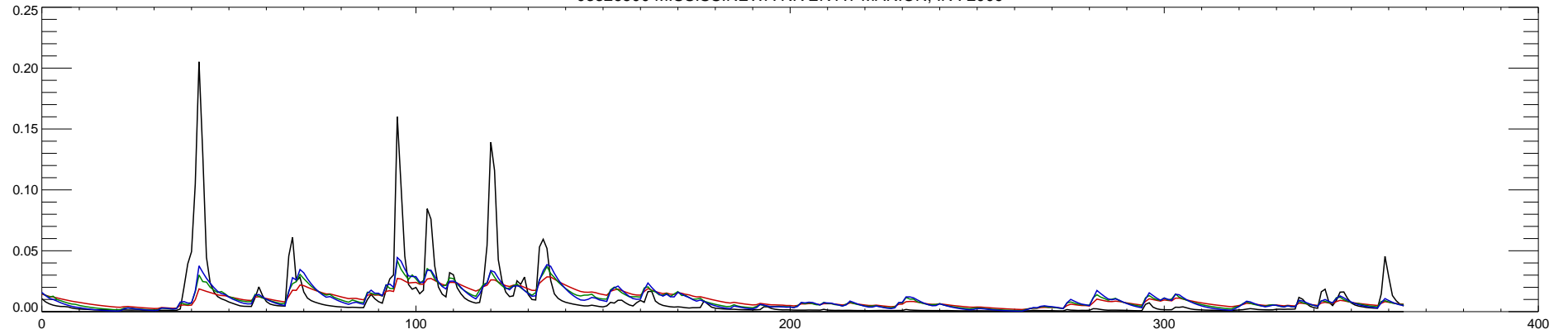
03326500 MISSISSINEWA RIVER AT MARION, IN : 2010
