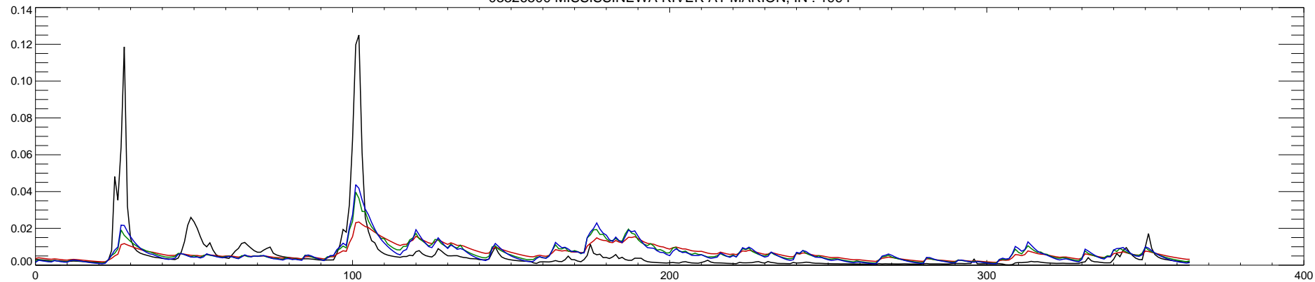
03326500 MISSISSINEWA RIVER AT MARION, IN : 1995
