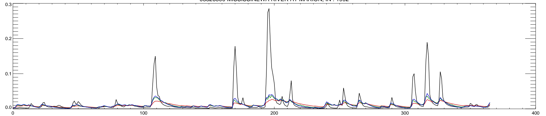
03326500 MISSISSINEWA RIVER AT MARION, IN : 1992
