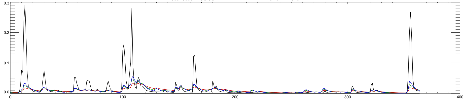
03326500 MISSISSINEWA RIVER AT MARION, IN : 2013
