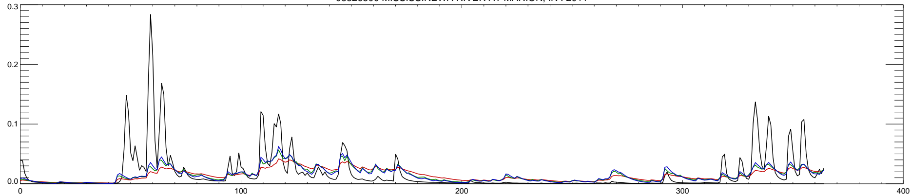
03326500 MISSISSINEWA RIVER AT MARION, IN : 2012
