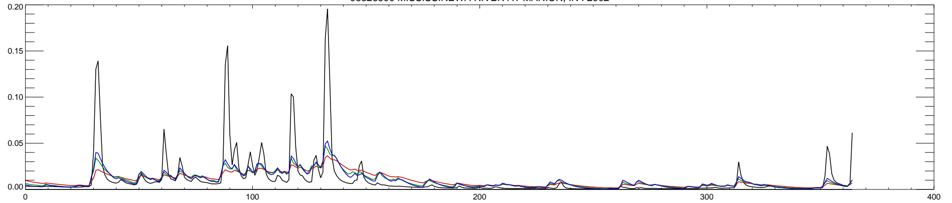
03326500 MISSISSINEWA RIVER AT MARION, IN : 2003
