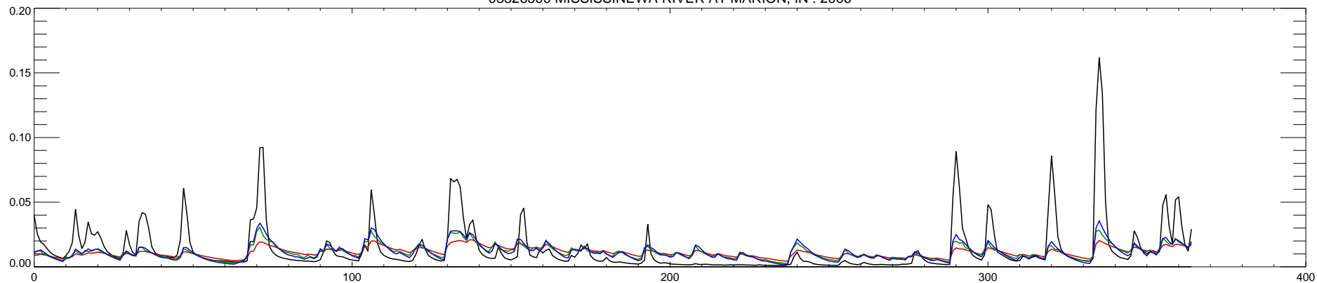
03326500 MISSISSINEWA RIVER AT MARION, IN : 2007
