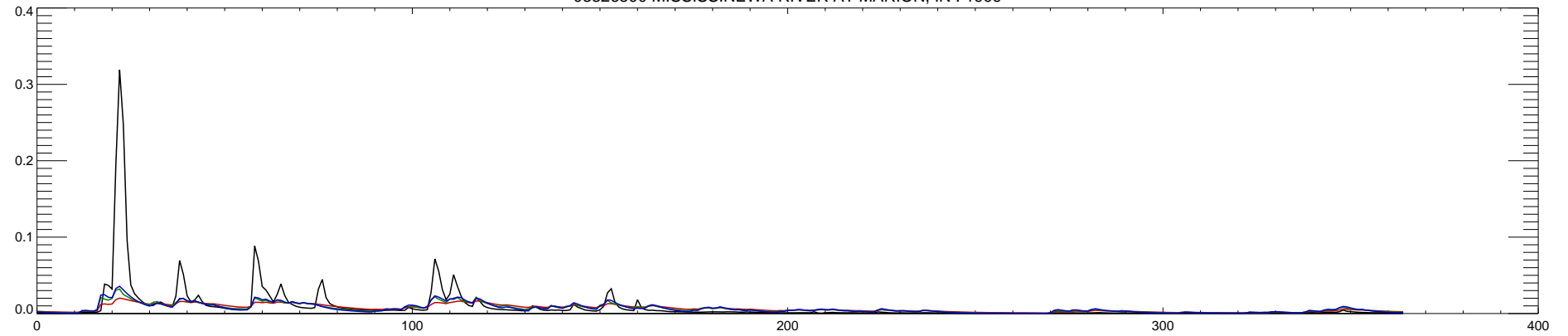
03326500 MISSISSINEWA RIVER AT MARION, IN : 2000
