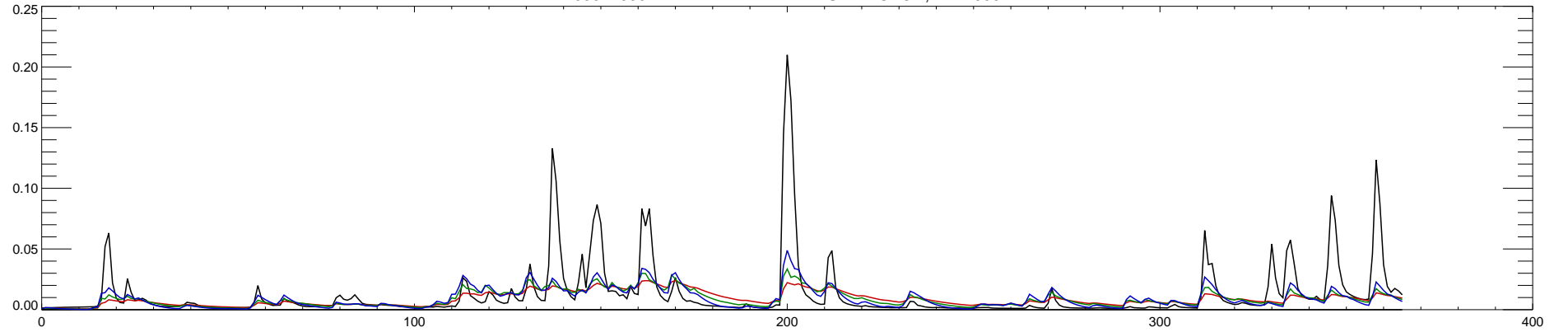
03324000 LITTLE RIVER NEAR HUNTINGTON, IN : 1997
