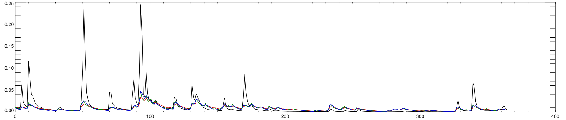
03272000 TWIN CREEK NEAR GERMANTOWN OH : 2015
