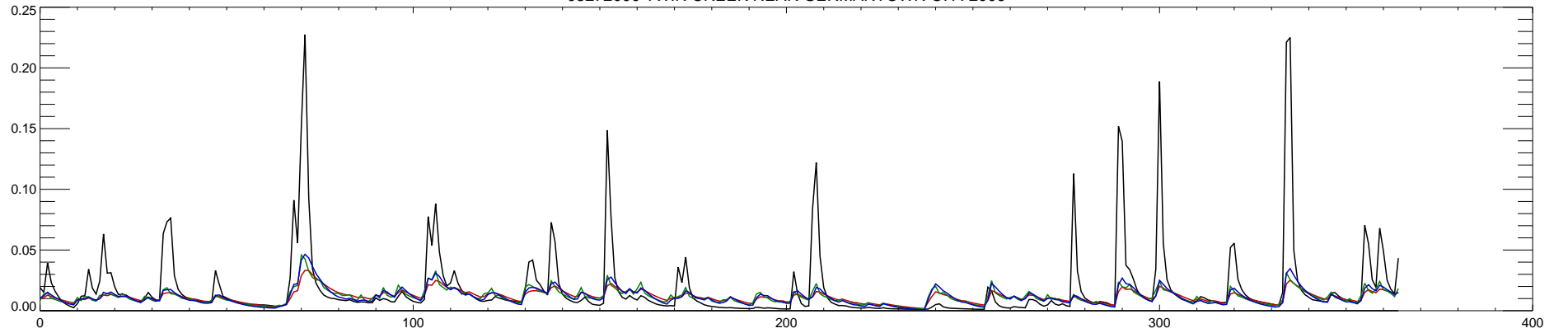
03272000 TWIN CREEK NEAR GERMANTOWN OH : 2007
