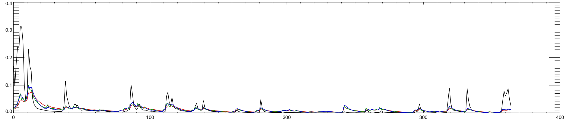
03272000 TWIN CREEK NEAR GERMANTOWN OH : 2006
