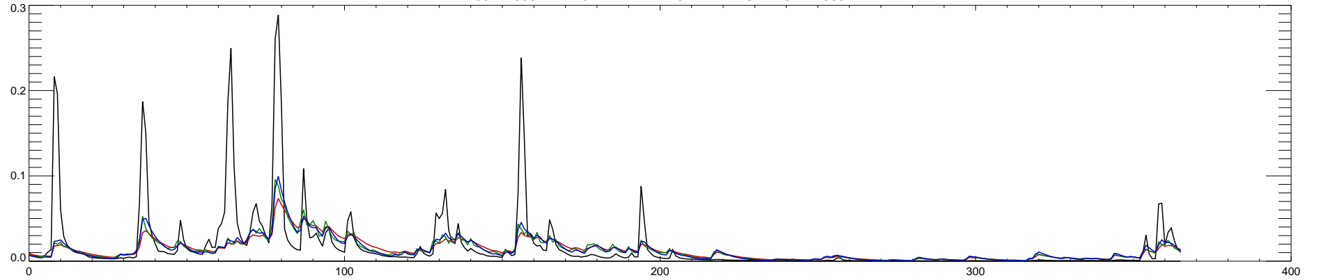
03272000 TWIN CREEK NEAR GERMANTOWN OH : 2009
