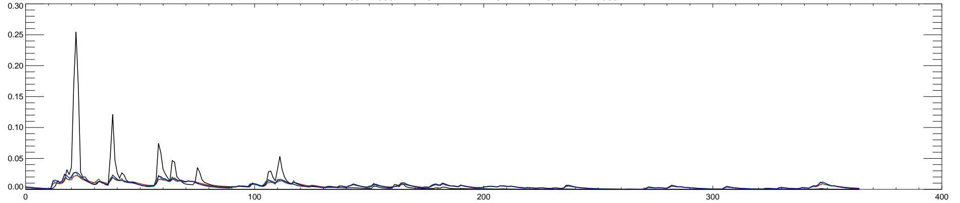
03272000 TWIN CREEK NEAR GERMANTOWN OH : 2000
