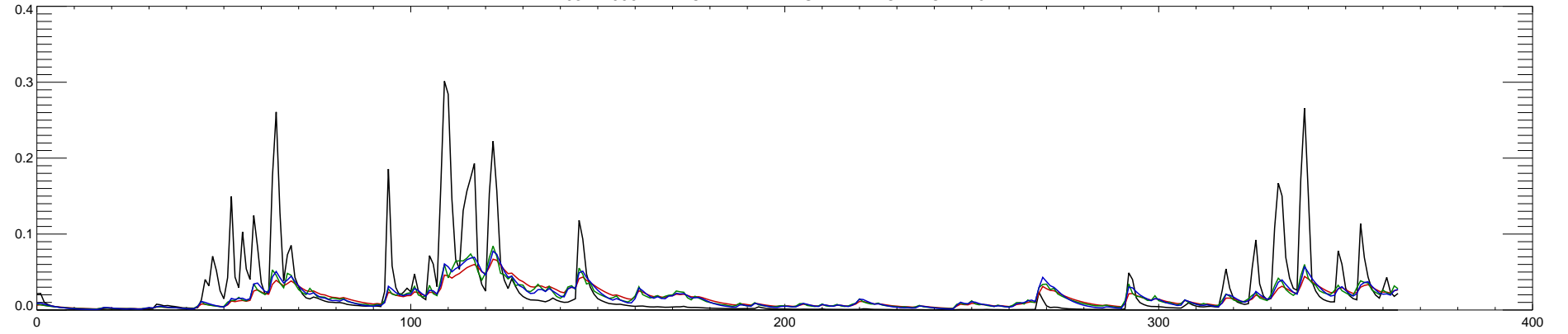
03272000 TWIN CREEK NEAR GERMANTOWN OH : 2012
