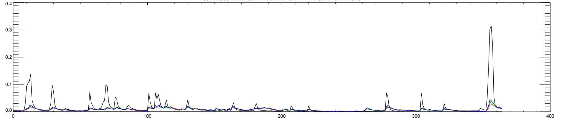
03272000 TWIN CREEK NEAR GERMANTOWN OH : 2013
