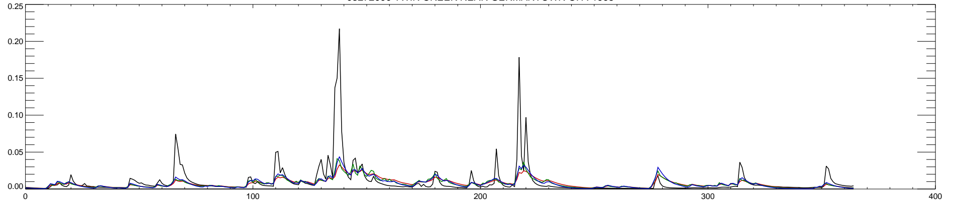
03272000 TWIN CREEK NEAR GERMANTOWN OH : 1995
