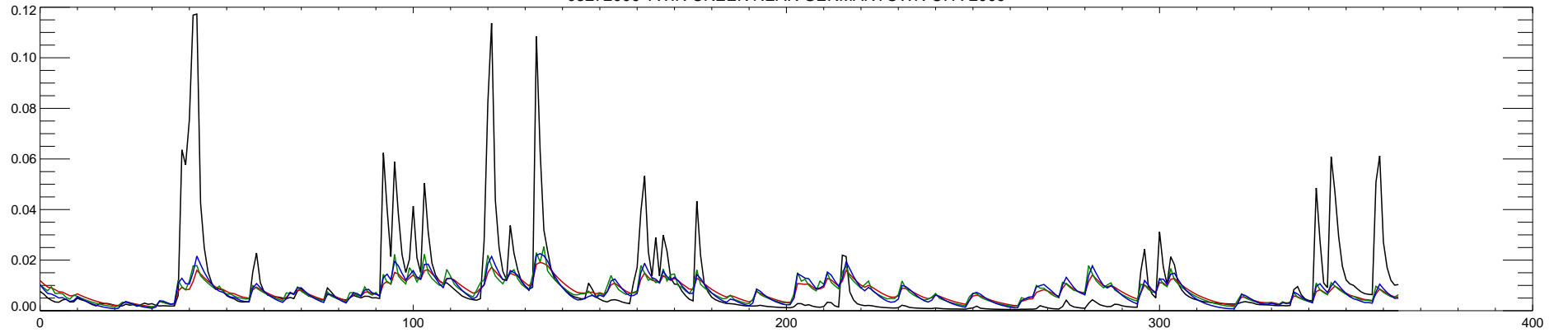
03272000 TWIN CREEK NEAR GERMANTOWN OH : 2010
