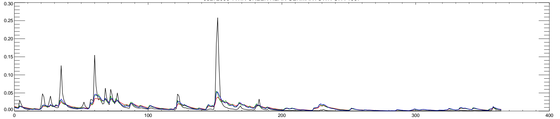
03272000 TWIN CREEK NEAR GERMANTOWN OH : 1998
