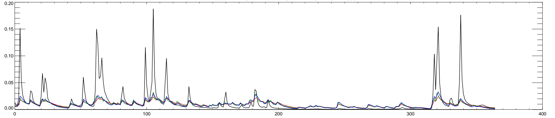
03272000 TWIN CREEK NEAR GERMANTOWN OH : 1994
