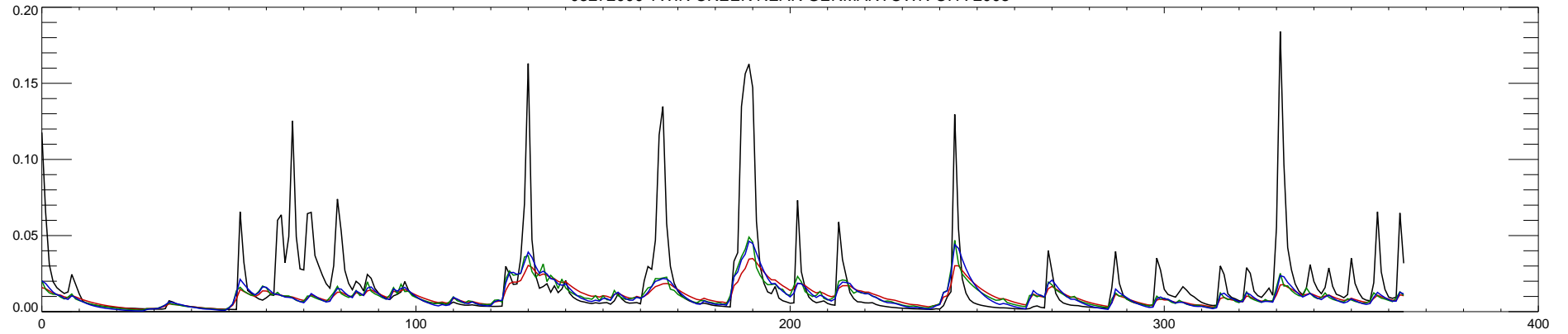
03272000 TWIN CREEK NEAR GERMANTOWN OH : 2004
