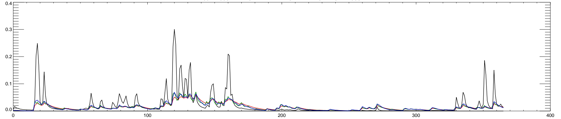
03272000 TWIN CREEK NEAR GERMANTOWN OH : 1997
