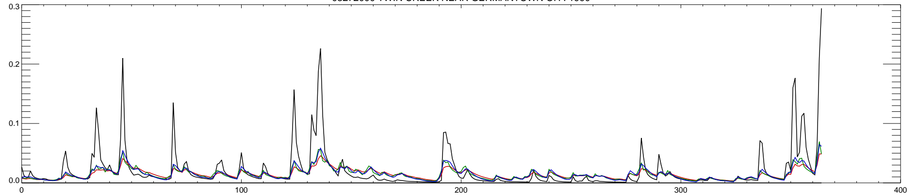
03272000 TWIN CREEK NEAR GERMANTOWN OH : 1991
