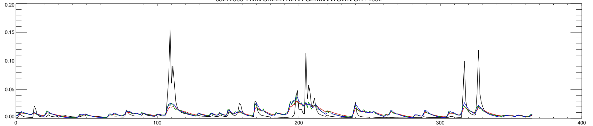
03272000 TWIN CREEK NEAR GERMANTOWN OH : 1992
