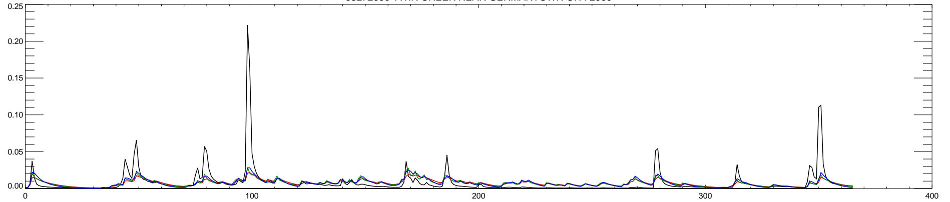
03272000 TWIN CREEK NEAR GERMANTOWN OH : 2001
