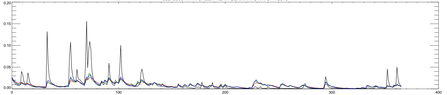
03272000 TWIN CREEK NEAR GERMANTOWN OH : 2016
