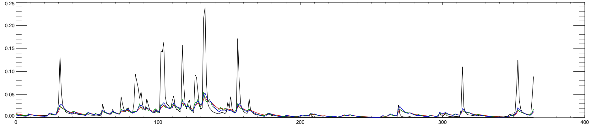
03272000 TWIN CREEK NEAR GERMANTOWN OH : 2003
