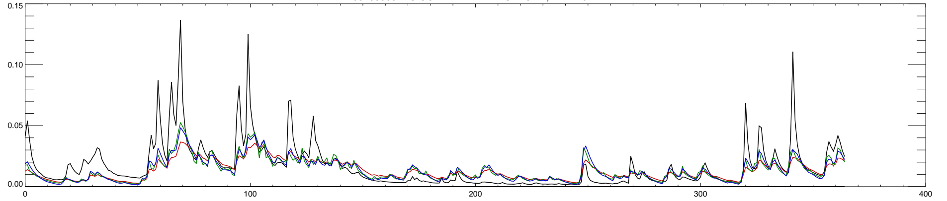
03198500 BIG COAL RIVER AT ASHFORD, WV : 2012
