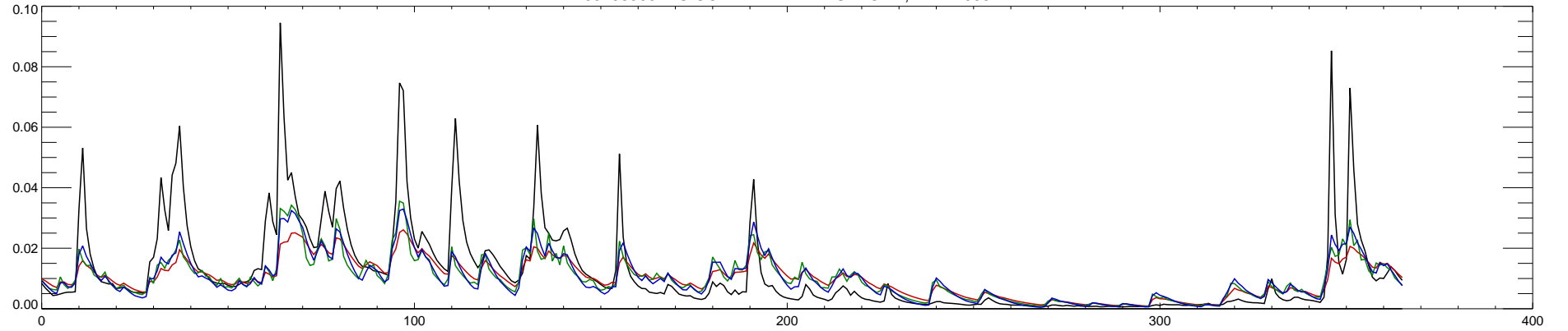
03198500 BIG COAL RIVER AT ASHFORD, WV : 2009
