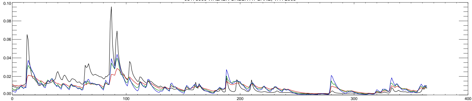
03173000 WALKER CREEK AT BANE, VA : 2006
