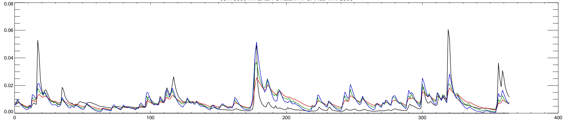
03173000 WALKER CREEK AT BANE, VA : 2007
