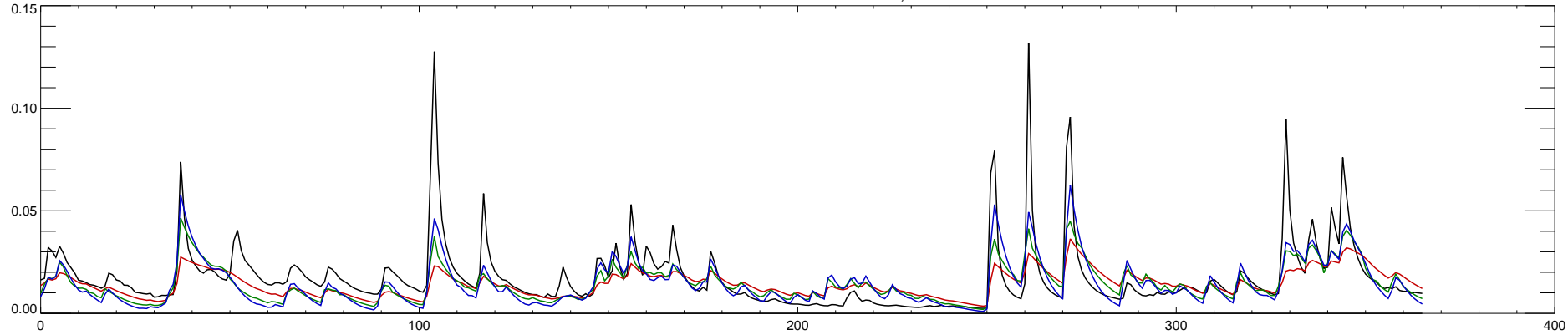
03173000 WALKER CREEK AT BANE, VA : 2004
