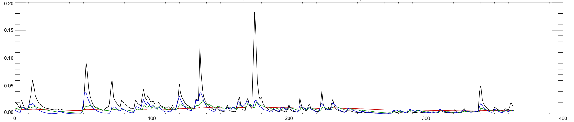
03106000 CONNOQUENESSING CREEK NEAR ZELIENOPLE, PA : 2015
