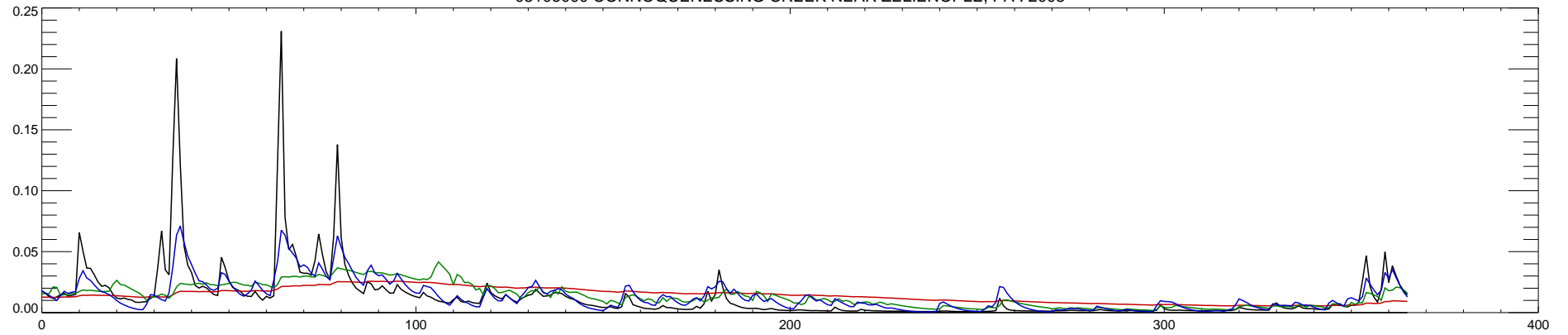
03106000 CONNOQUENESSING CREEK NEAR ZELIENOPLE, PA : 2009
