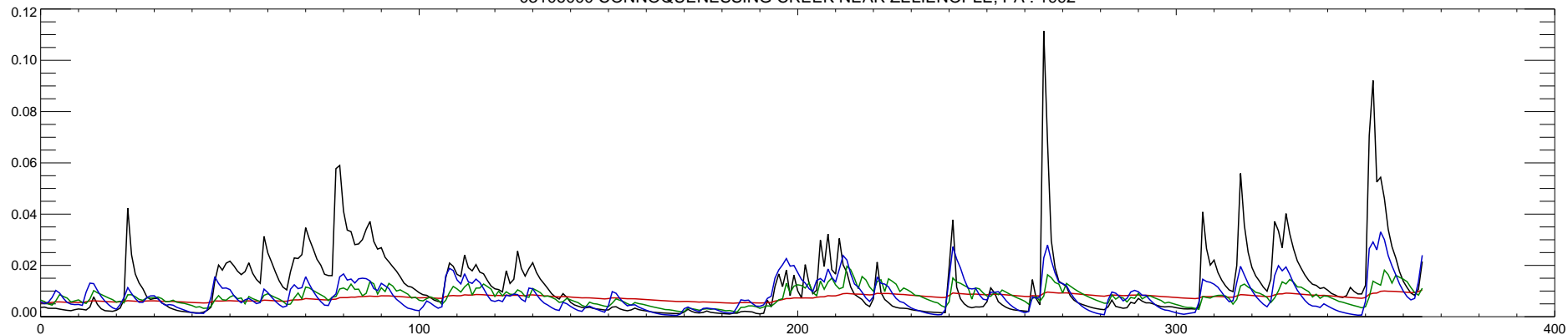
03106000 CONNOQUENESSING CREEK NEAR ZELIENOPLE, PA : 1992
