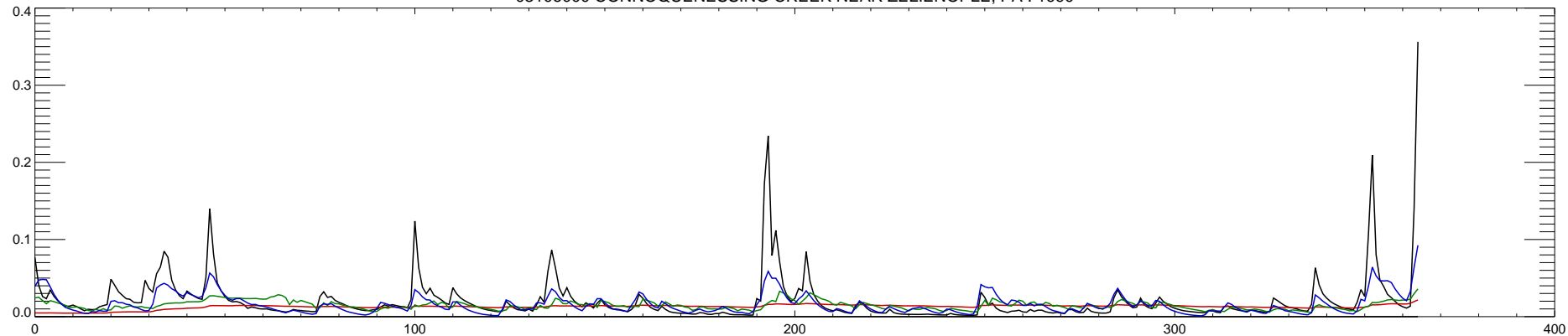
03106000 CONNOQUENESSING CREEK NEAR ZELIENOPLE, PA : 1991
