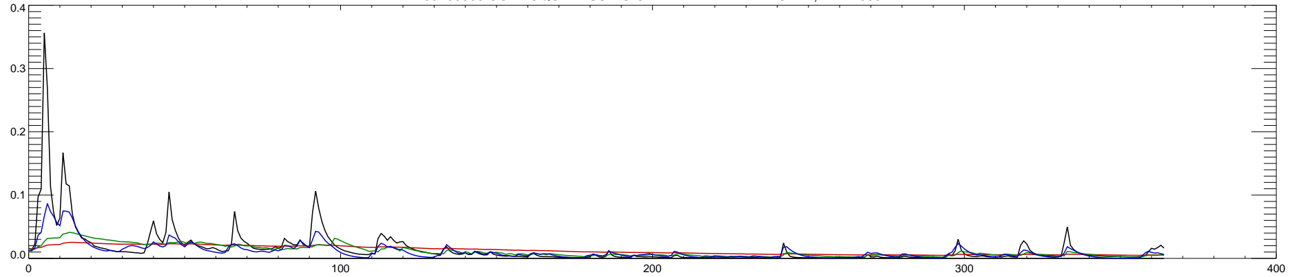
03106000 CONNOQUENESSING CREEK NEAR ZELIENOPLE, PA : 2006
