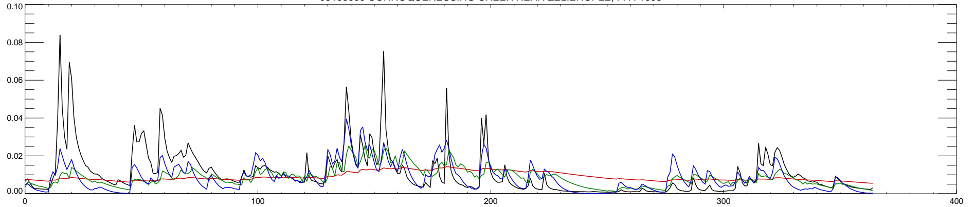
03106000 CONNOQUENESSING CREEK NEAR ZELIENOPLE, PA : 1995
