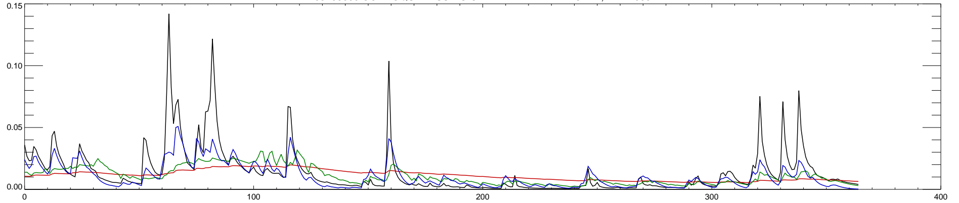
03106000 CONNOQUENESSING CREEK NEAR ZELIENOPLE, PA : 1994
