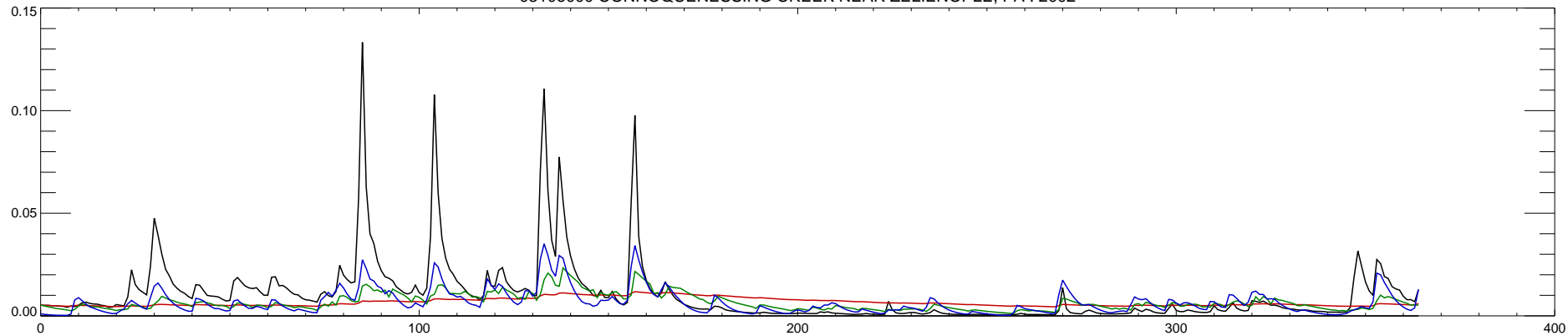
03106000 CONNOQUENESSING CREEK NEAR ZELIENOPLE, PA : 2003
