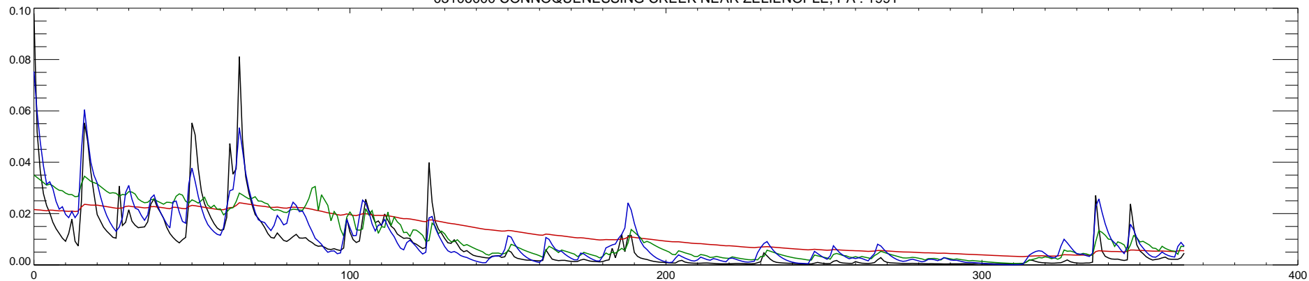
03106000 CONNOQUENESSING CREEK NEAR ZELIENOPLE, PA : 1992
