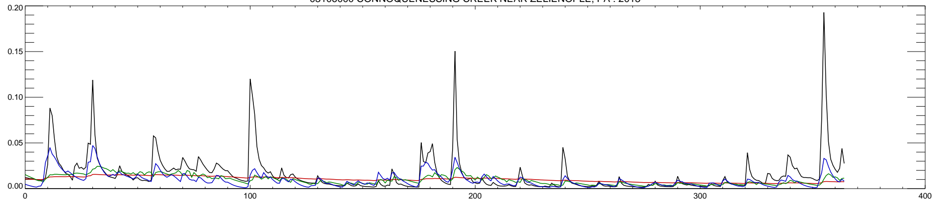
03106000 CONNOQUENESSING CREEK NEAR ZELIENOPLE, PA : 2013
