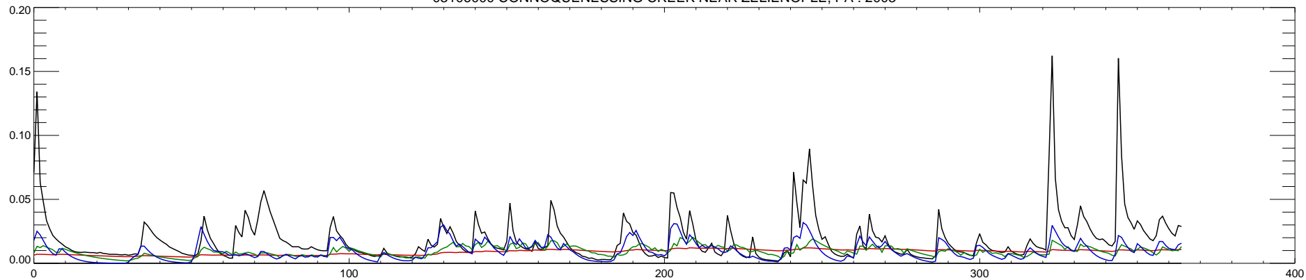
03106000 CONNOQUENESSING CREEK NEAR ZELIENOPLE, PA : 2004
