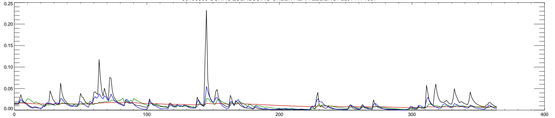
03106000 CONNOQUENESSING CREEK NEAR ZELIENOPLE, PA : 1998
