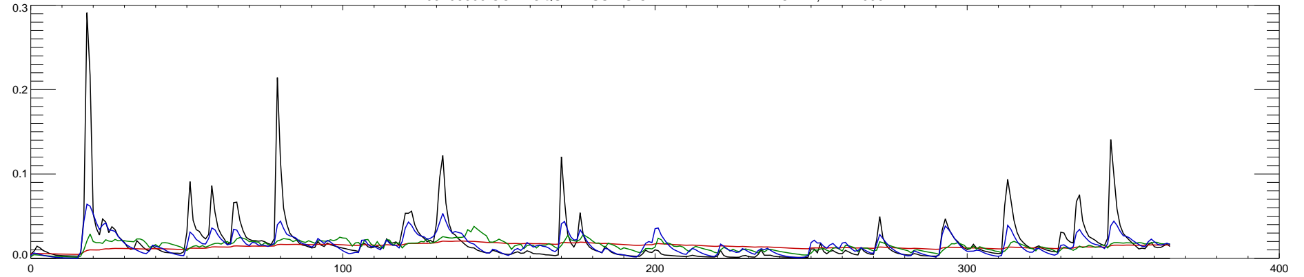
03106000 CONNOQUENESSING CREEK NEAR ZELIENOPLE, PA : 1997
