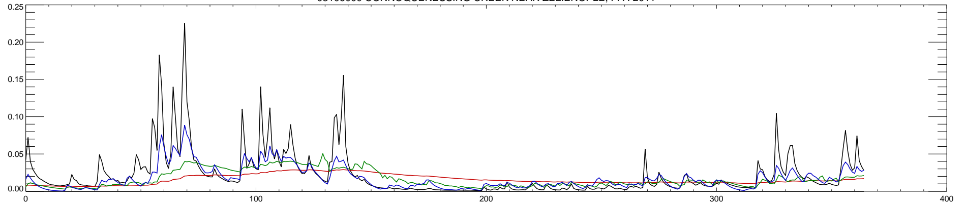
03106000 CONNOQUENESSING CREEK NEAR ZELIENOPLE, PA : 2012
