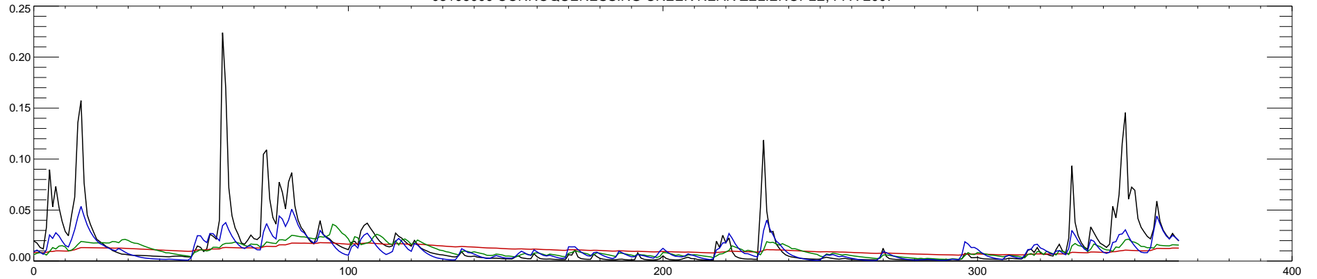
03106000 CONNOQUENESSING CREEK NEAR ZELIENOPLE, PA : 2007
