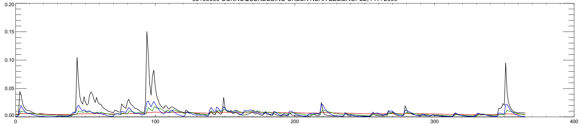
03106000 CONNOQUENESSING CREEK NEAR ZELIENOPLE, PA : 2001
