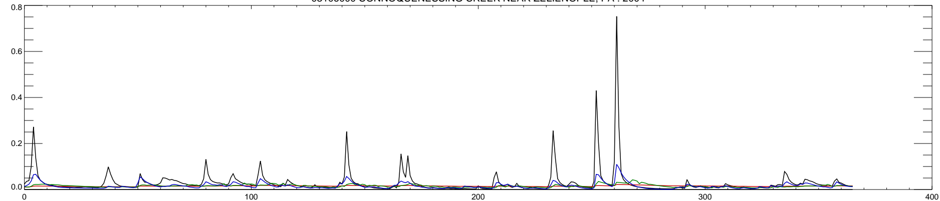
03106000 CONNOQUENESSING CREEK NEAR ZELIENOPLE, PA : 2004
