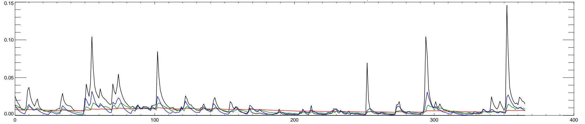
03106000 CONNOQUENESSING CREEK NEAR ZELIENOPLE, PA : 2016
