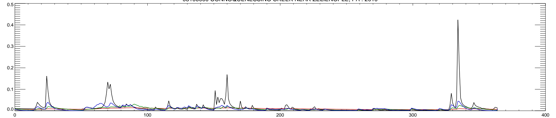
03106000 CONNOQUENESSING CREEK NEAR ZELIENOPLE, PA : 2010
