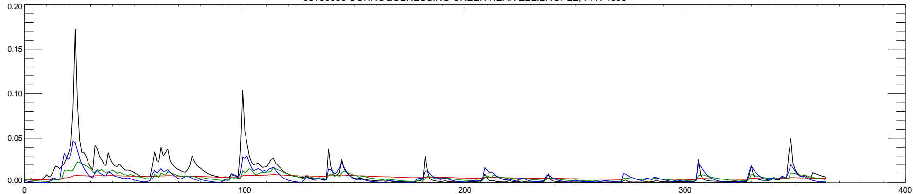
03106000 CONNOQUENESSING CREEK NEAR ZELIENOPLE, PA : 2000
