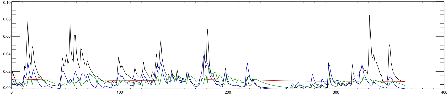
03079000 CASSELMAN RIVER AT MARKLETON, PA : 1995
