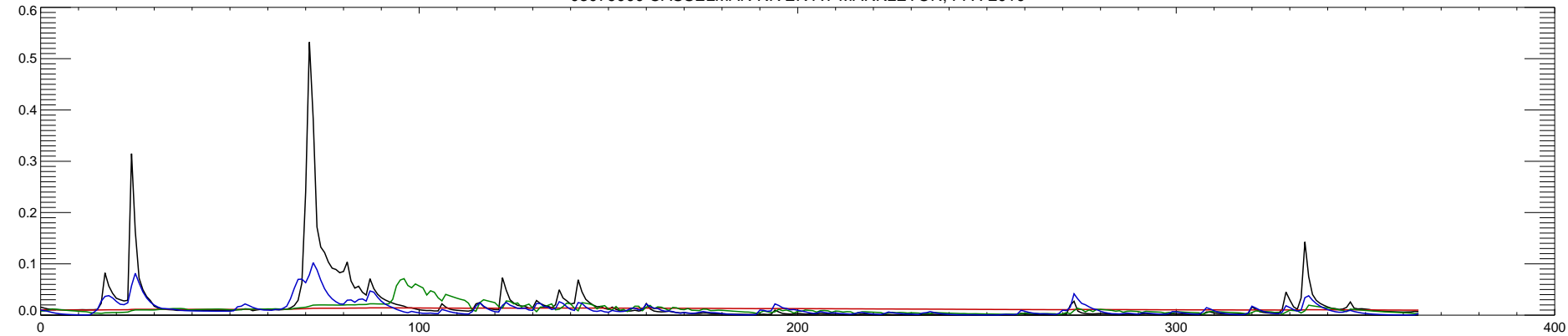
03079000 CASSELMAN RIVER AT MARKLETON, PA : 2010
