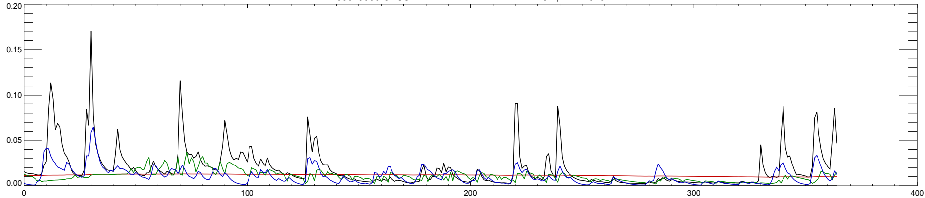
03079000 CASSELMAN RIVER AT MARKLETON, PA : 2013
