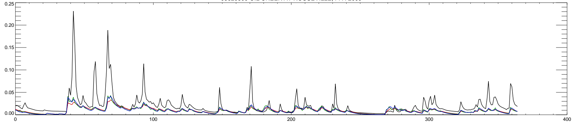
03020500 OIL CREEK AT ROUSEVILLE, PA : 2010
