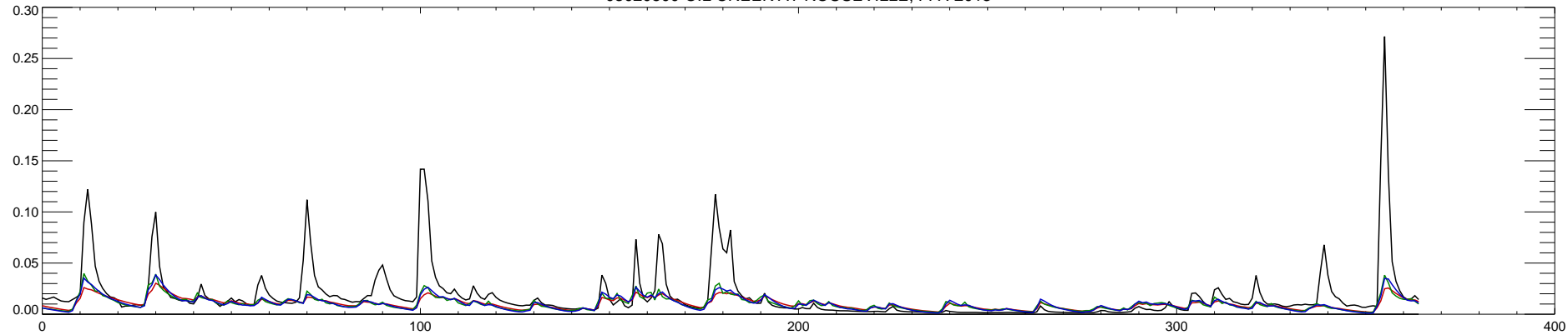
03020500 OIL CREEK AT ROUSEVILLE, PA : 2013
