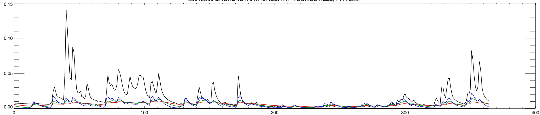
03015500 BROKENSTRAW CREEK AT YOUNGSVILLE, PA : 2001
