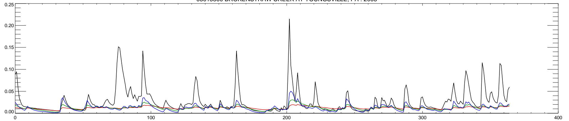
03015500 BROKENSTRAW CREEK AT YOUNGSVILLE, PA : 2004
