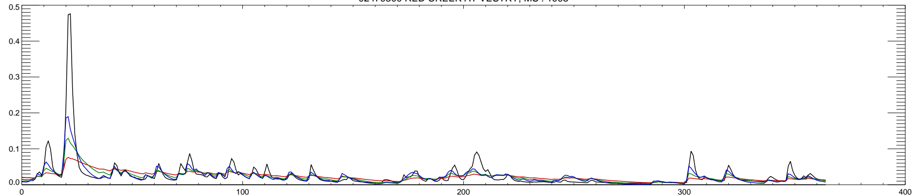
02479300 RED CREEK AT VESTRY, MS : 1994
