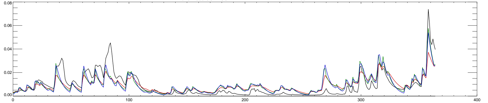
02371500 CONECUH RIVER AT BRANTLEY AL : 2003
