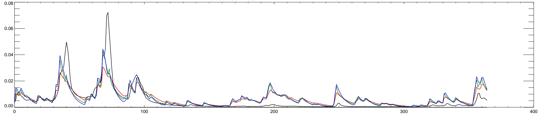
02371500 CONECUH RIVER AT BRANTLEY AL : 2012
