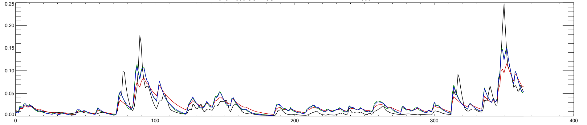
02371500 CONECUH RIVER AT BRANTLEY AL : 2010
