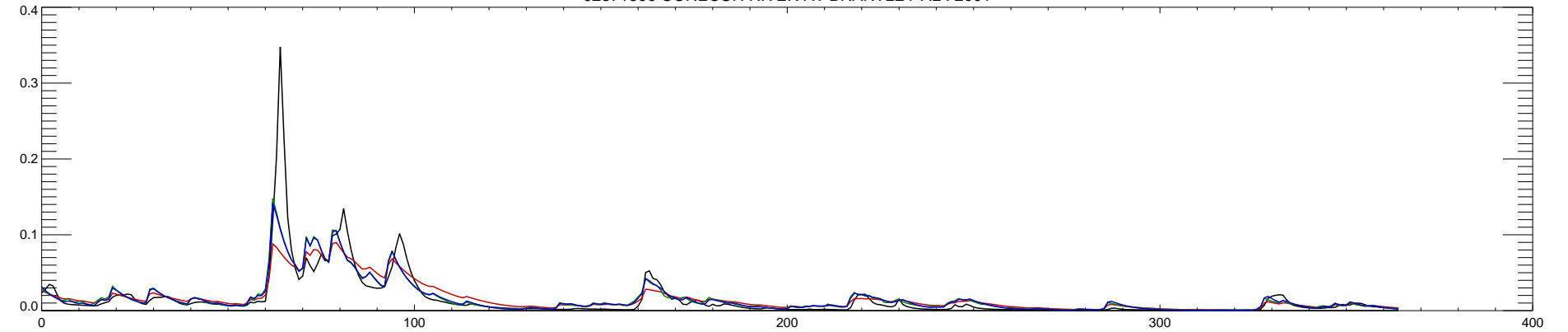
02371500 CONECUH RIVER AT BRANTLEY AL : 2001
