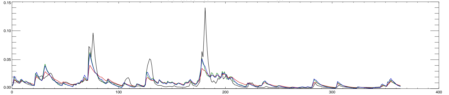
02371500 CONECUH RIVER AT BRANTLEY AL : 2000
