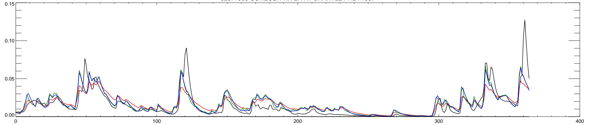
02371500 CONECUH RIVER AT BRANTLEY AL : 1998
