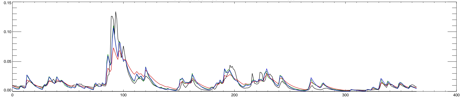
02371500 CONECUH RIVER AT BRANTLEY AL : 2006
