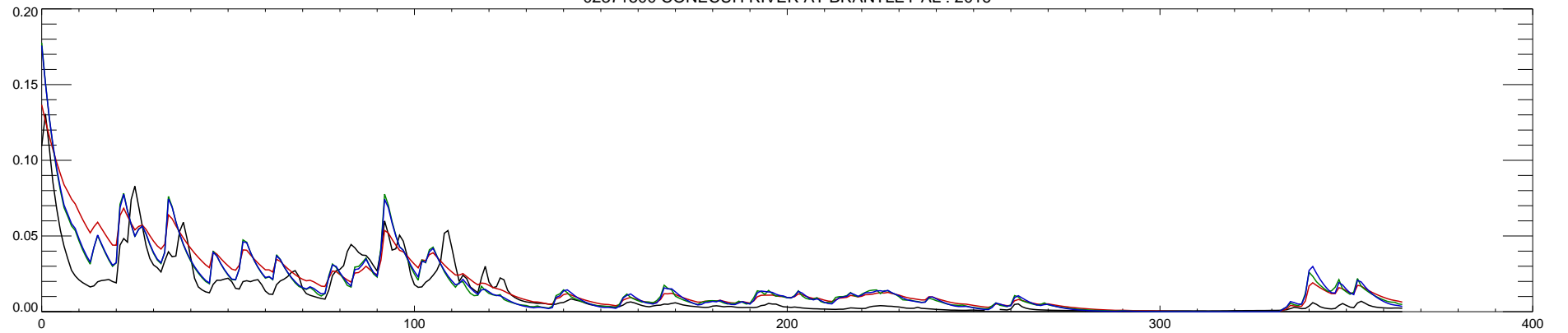
02371500 CONECUH RIVER AT BRANTLEY AL : 2016
