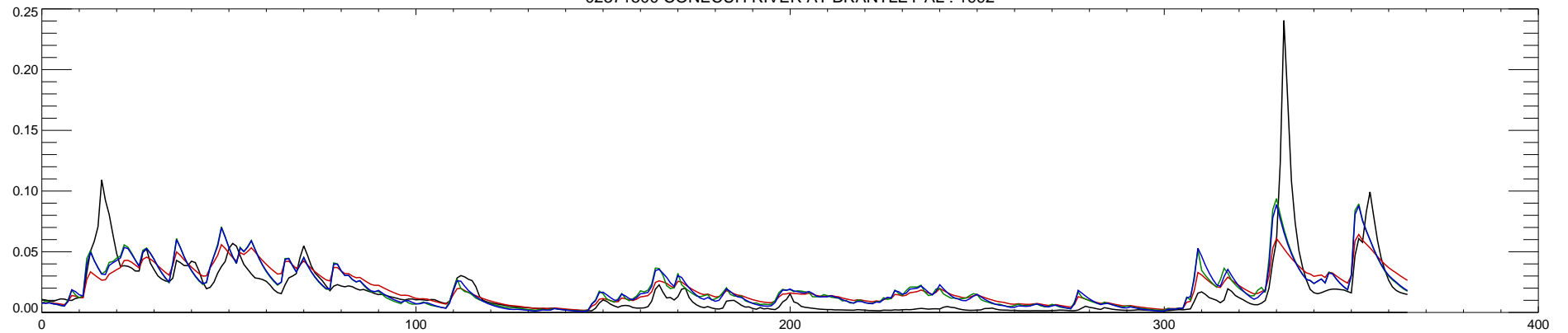
02371500 CONECUH RIVER AT BRANTLEY AL : 1992
