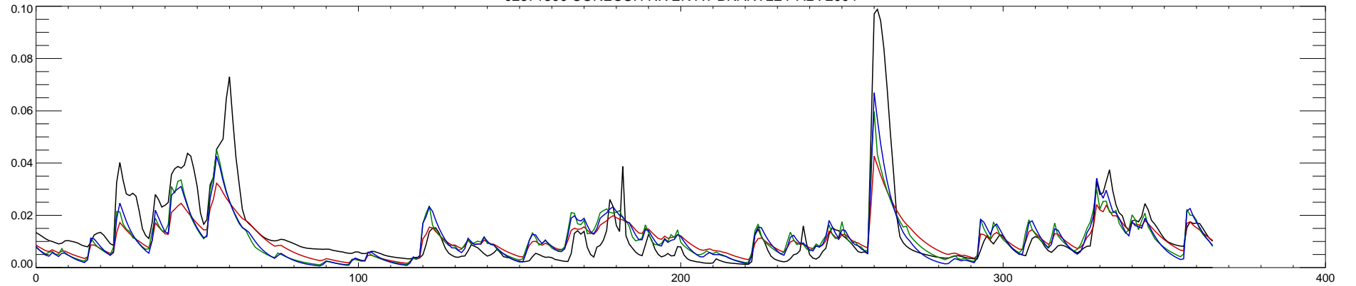
02371500 CONECUH RIVER AT BRANTLEY AL : 2004
