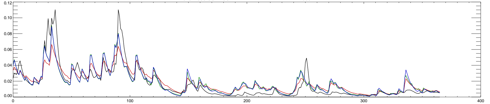
02371500 CONECUH RIVER AT BRANTLEY AL : 1997
