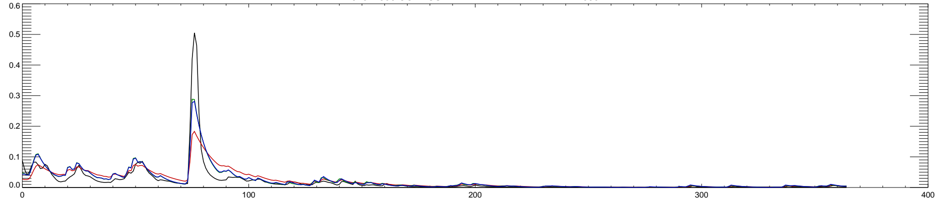
02371500 CONECUH RIVER AT BRANTLEY AL : 1991
