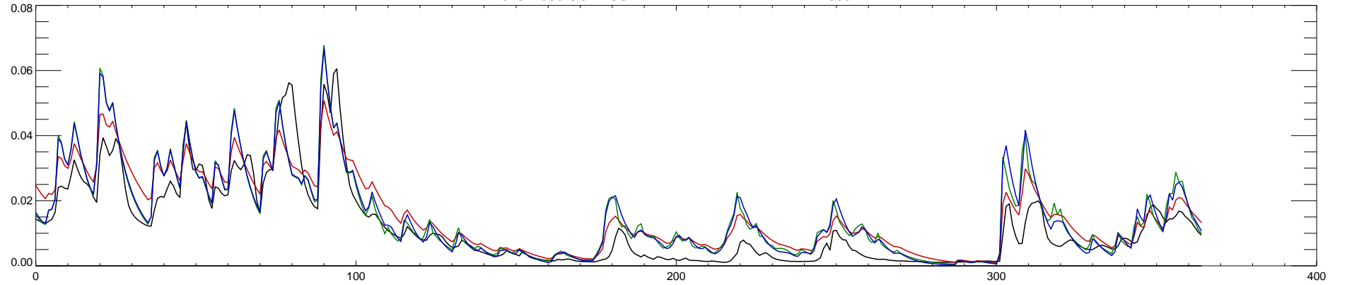
02371500 CONECUH RIVER AT BRANTLEY AL : 1994
