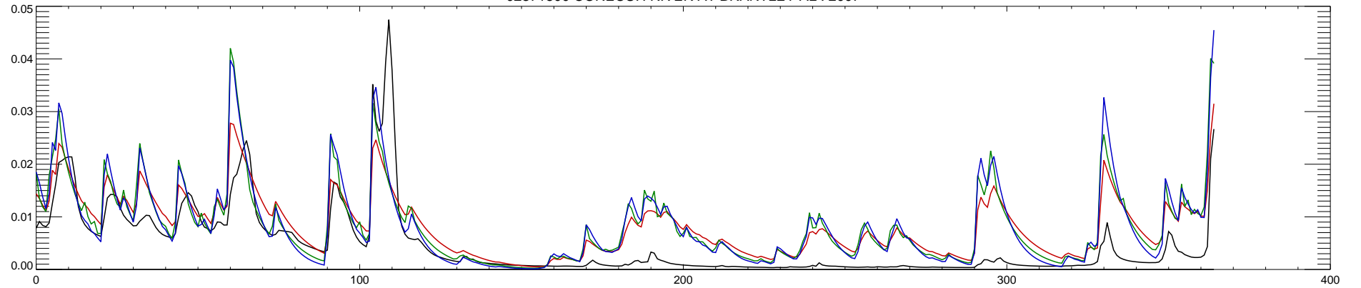
02371500 CONECUH RIVER AT BRANTLEY AL : 2007
