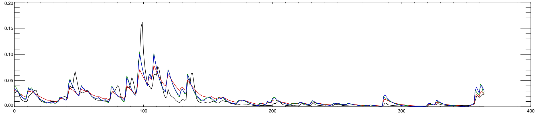
02371500 CONECUH RIVER AT BRANTLEY AL : 2015
