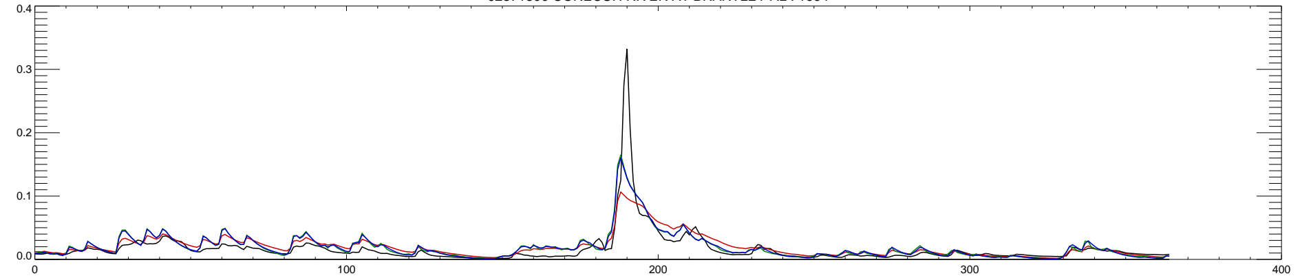
02371500 CONECUH RIVER AT BRANTLEY AL : 1995
