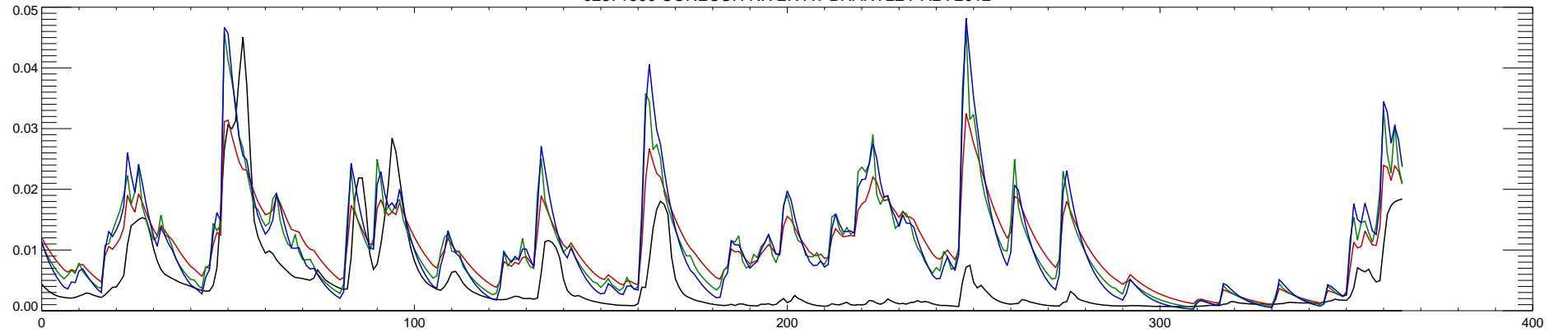
02371500 CONECUH RIVER AT BRANTLEY AL : 2013
