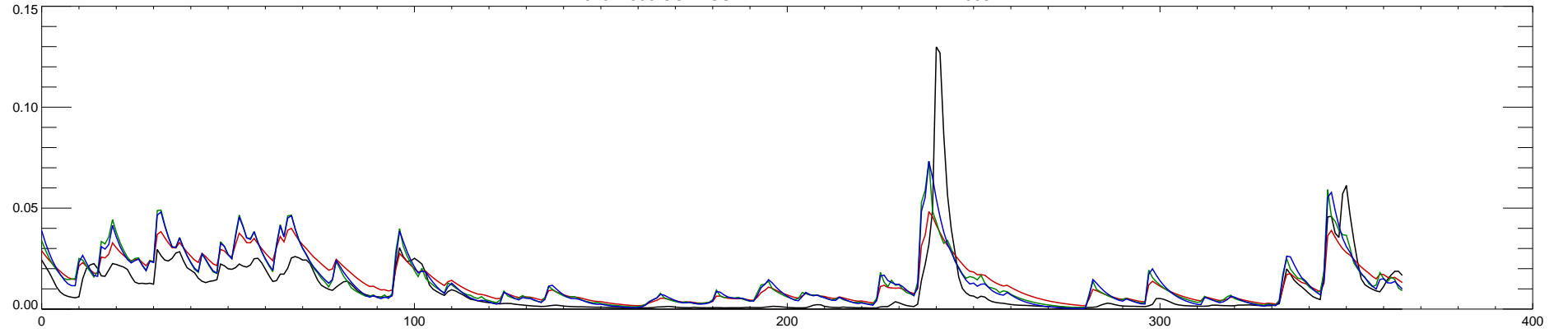
02371500 CONECUH RIVER AT BRANTLEY AL : 2009
