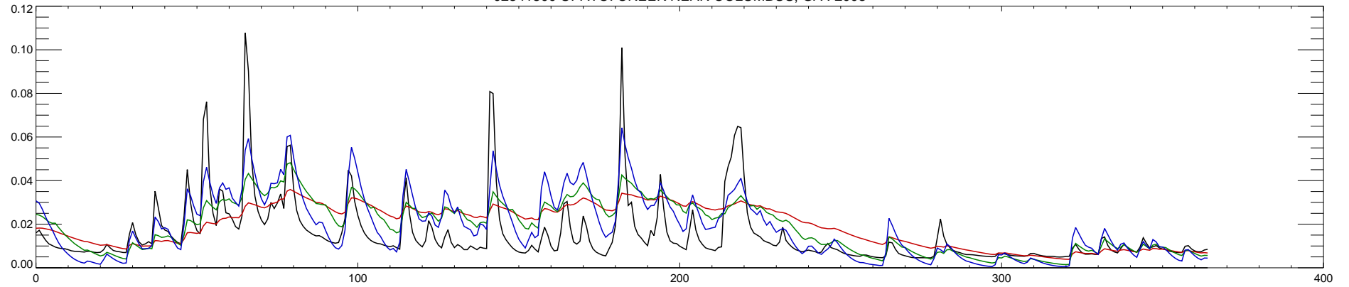
02341800 UPATOI CREEK NEAR COLUMBUS, GA : 2004
