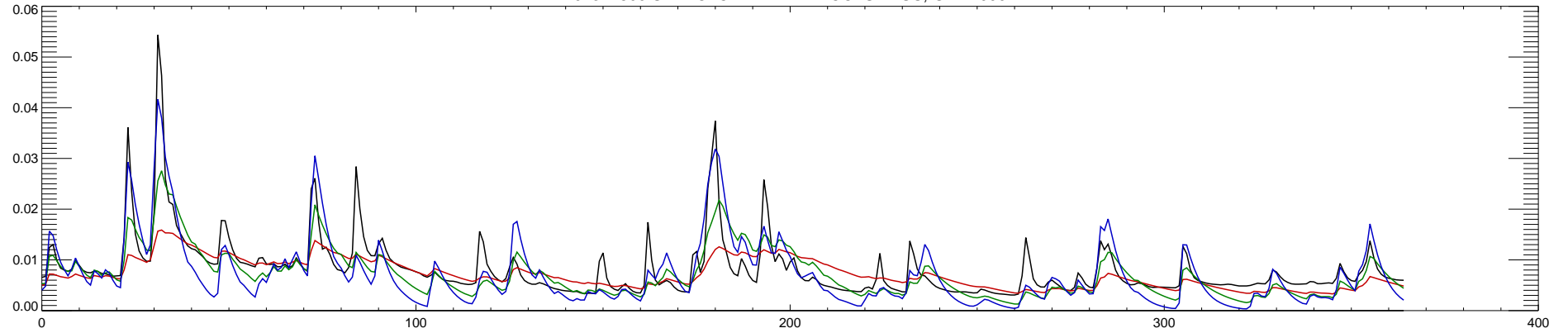
02341800 UPATOI CREEK NEAR COLUMBUS, GA : 2000
