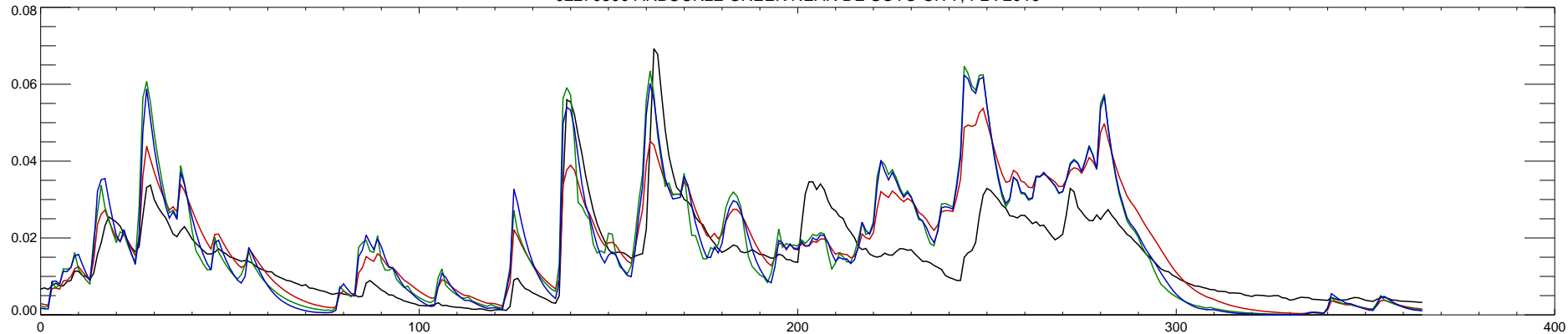
02270500 ARBUCKLE CREEK NEAR DE SOTO CITY, FL : 2016
