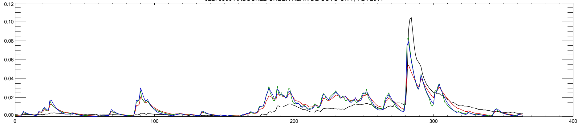
02270500 ARBUCKLE CREEK NEAR DE SOTO CITY, FL : 2012
