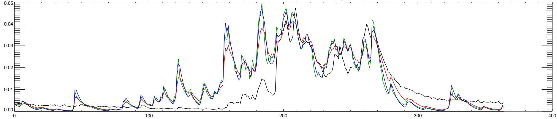
02270500 ARBUCKLE CREEK NEAR DE SOTO CITY, FL : 2013
