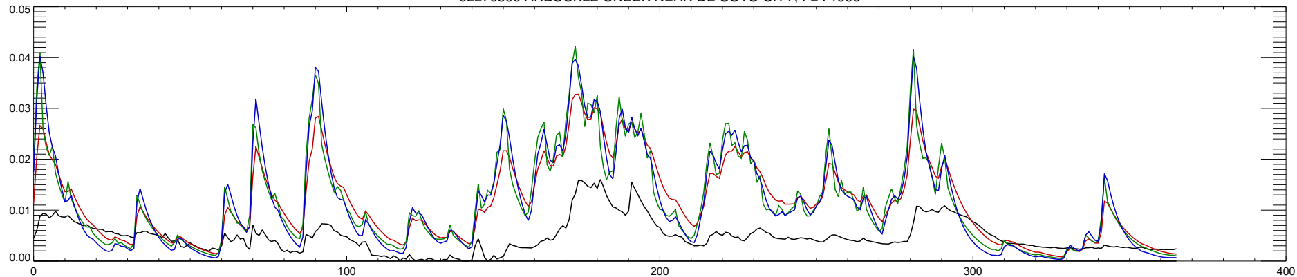
02270500 ARBUCKLE CREEK NEAR DE SOTO CITY, FL : 1997
