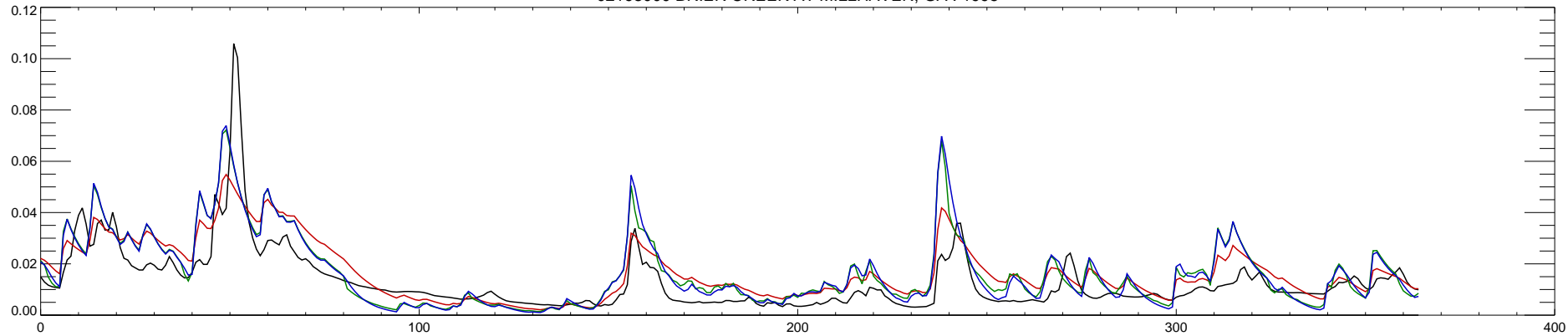
02198000 BRIER CREEK AT MILLHAVEN, GA : 1995
