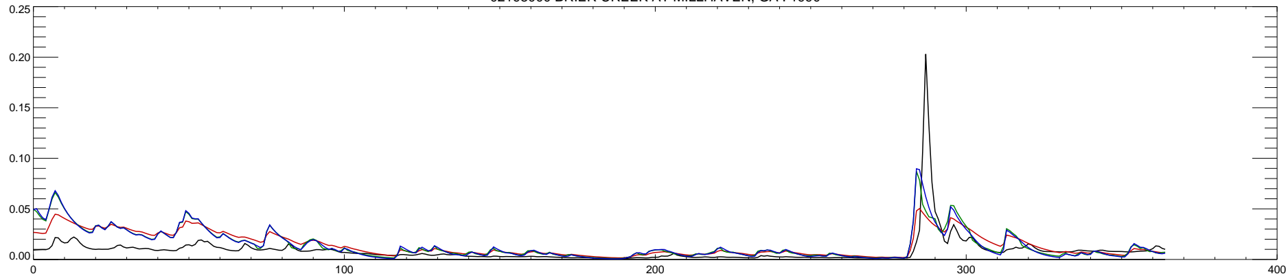
02198000 BRIER CREEK AT MILLHAVEN, GA : 1991
