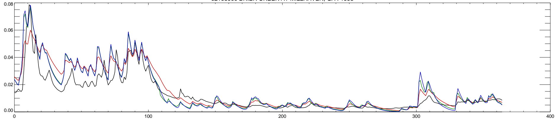
02198000 BRIER CREEK AT MILLHAVEN, GA : 1994
