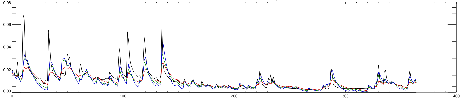
02061500 BIG OTTER RIVER NEAR EVINGTON, VA : 2015
