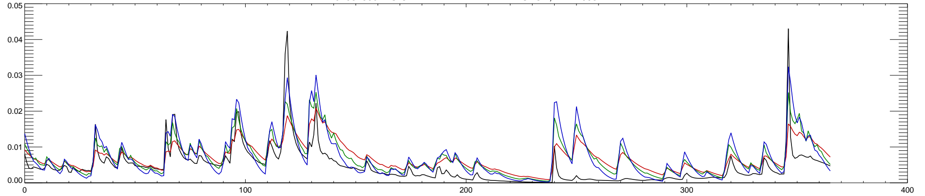
02061500 BIG OTTER RIVER NEAR EVINGTON, VA : 2009
