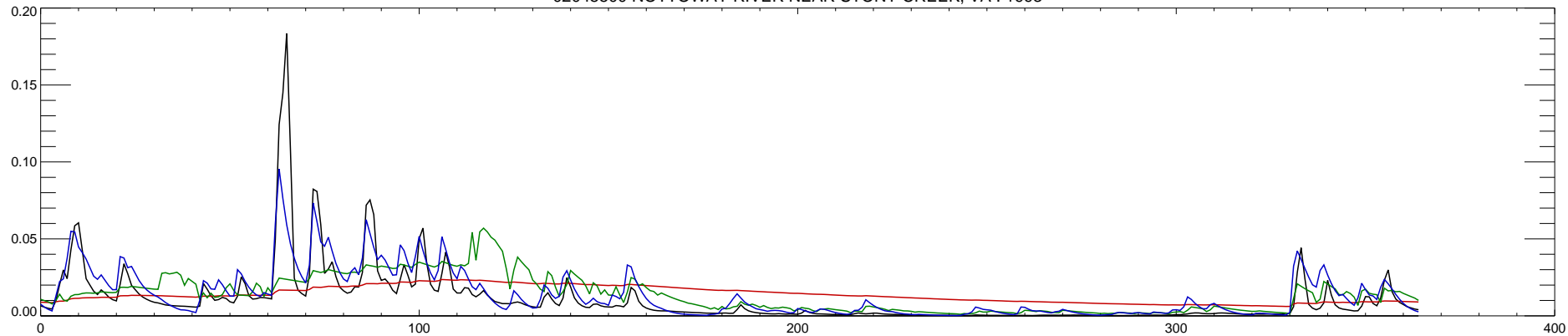
02045500 NOTTOWAY RIVER NEAR STONY CREEK, VA : 1994
