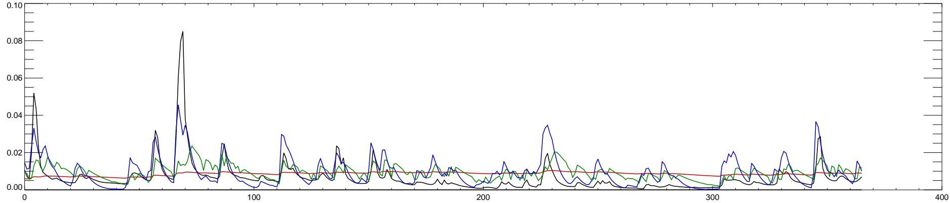
02045500 NOTTOWAY RIVER NEAR STONY CREEK, VA : 1992
