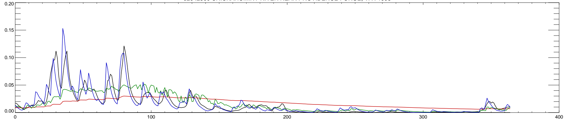
02042500 CHICKAHOMINY RIVER NEAR PROVIDENCE FORGE, VA : 1998
