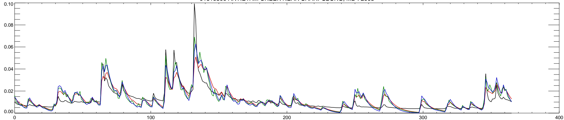
01619500 ANTIETAM CREEK NEAR SHARPSBURG, MD : 2009
