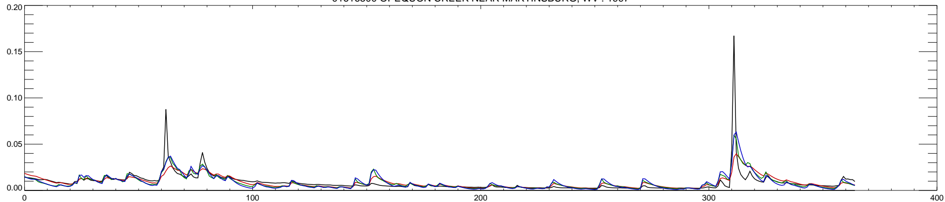
01616500 OPEQUON CREEK NEAR MARTINSBURG, WV : 1998
