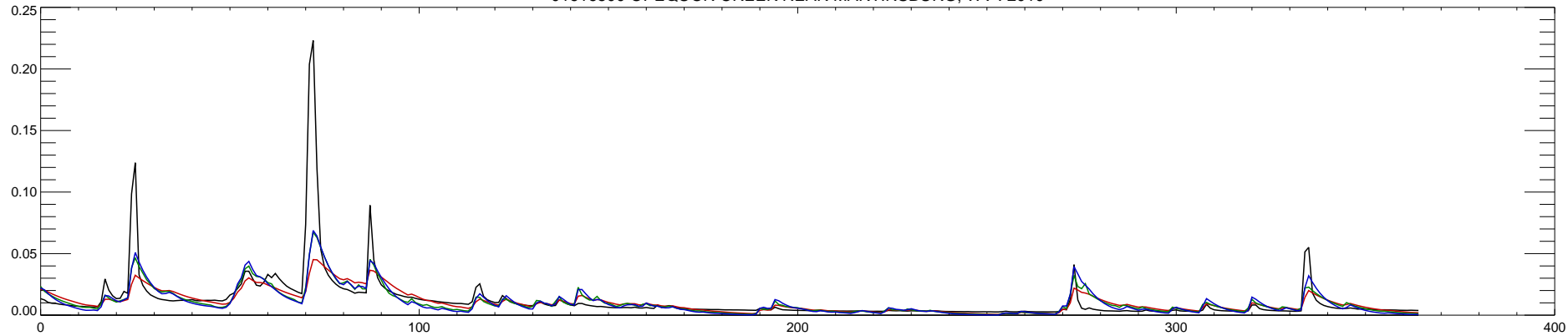
01616500 OPEQUON CREEK NEAR MARTINSBURG, WV : 2010
