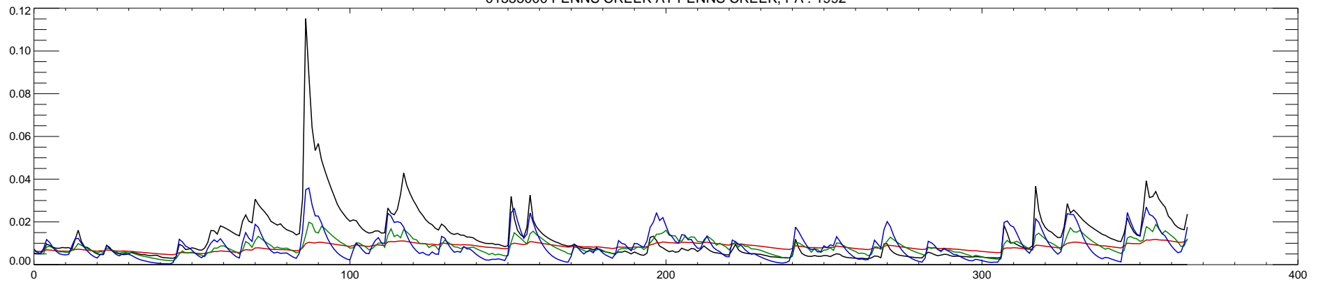
01555000 PENNS CREEK AT PENNS CREEK, PA : 1992
