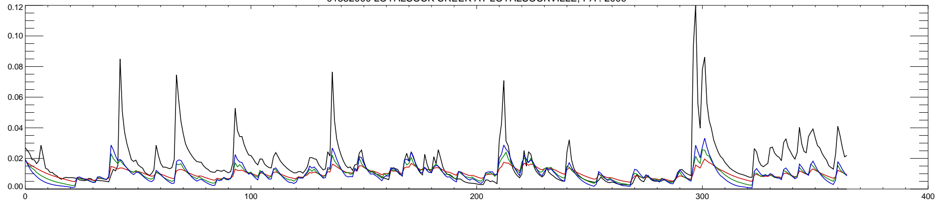
01552000 LOYALSOCK CREEK AT LOYALSOCKVILLE, PA : 2010
