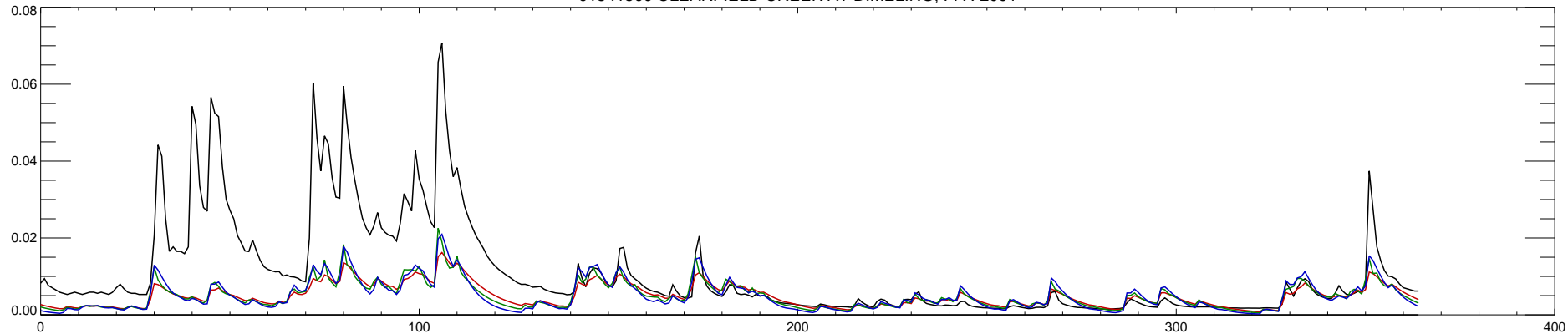
01541500 CLEARFIELD CREEK AT DIMELING, PA : 2001
