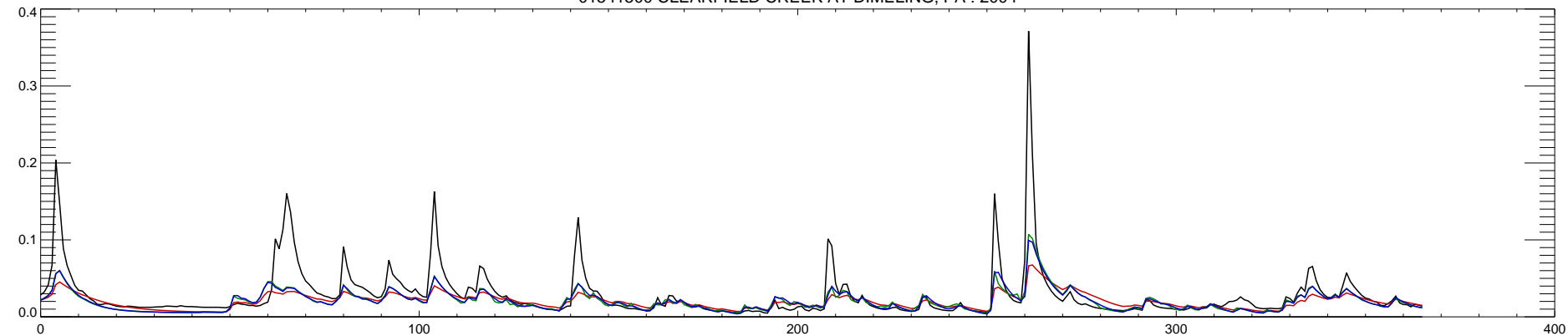
01541500 CLEARFIELD CREEK AT DIMELING, PA : 2004
