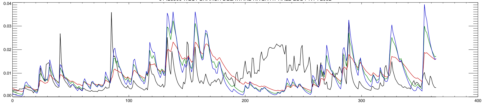
01426500 WEST BRANCH DELAWARE RIVER AT HALE EDDY NY : 2003
