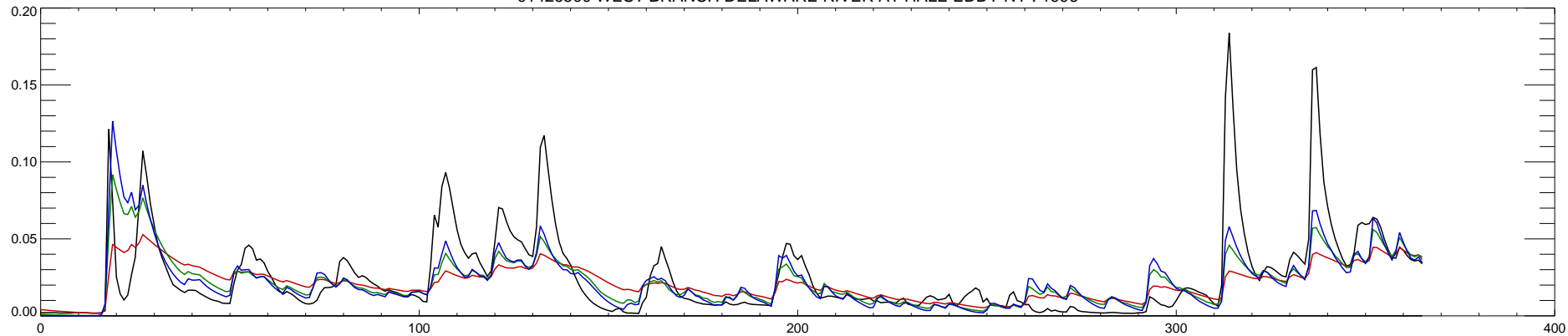
01426500 WEST BRANCH DELAWARE RIVER AT HALE EDDY NY : 1997
