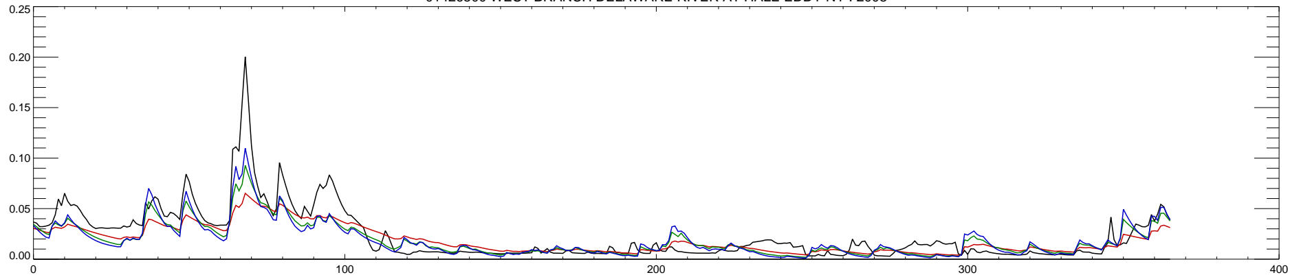
01426500 WEST BRANCH DELAWARE RIVER AT HALE EDDY NY : 2009
