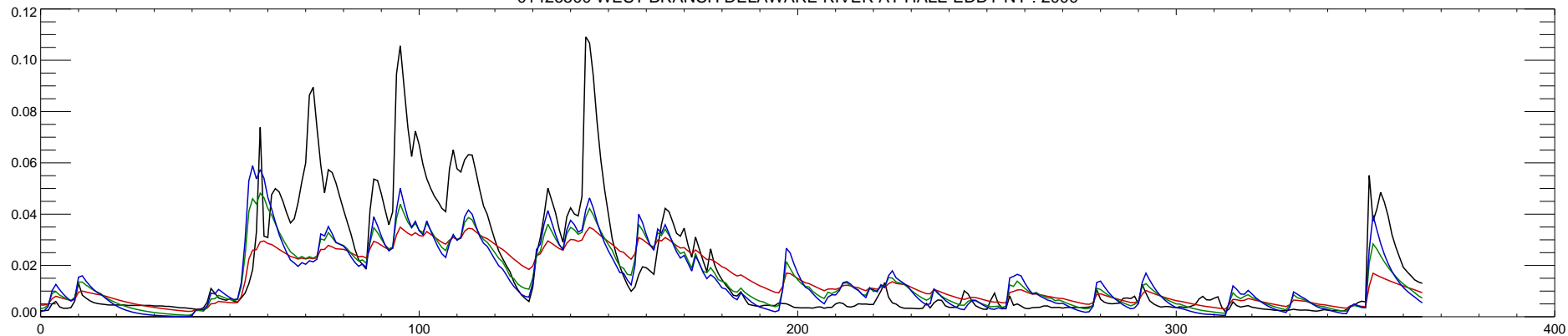
01426500 WEST BRANCH DELAWARE RIVER AT HALE EDDY NY : 2001
