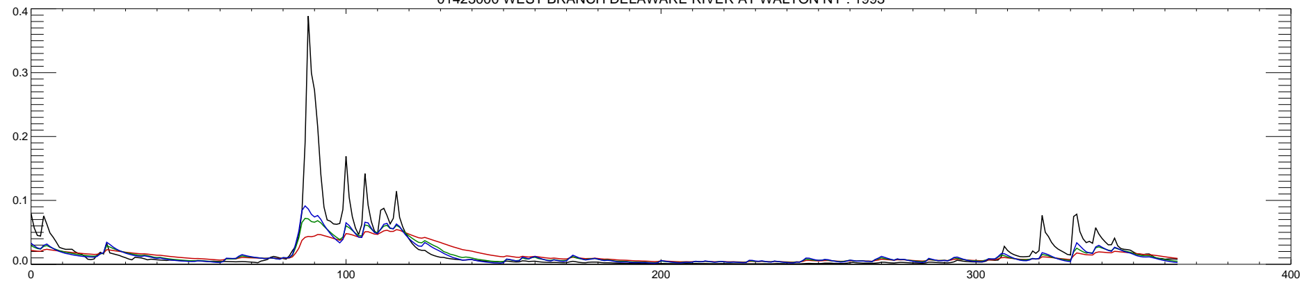
01423000 WEST BRANCH DELAWARE RIVER AT WALTON NY : 1994
