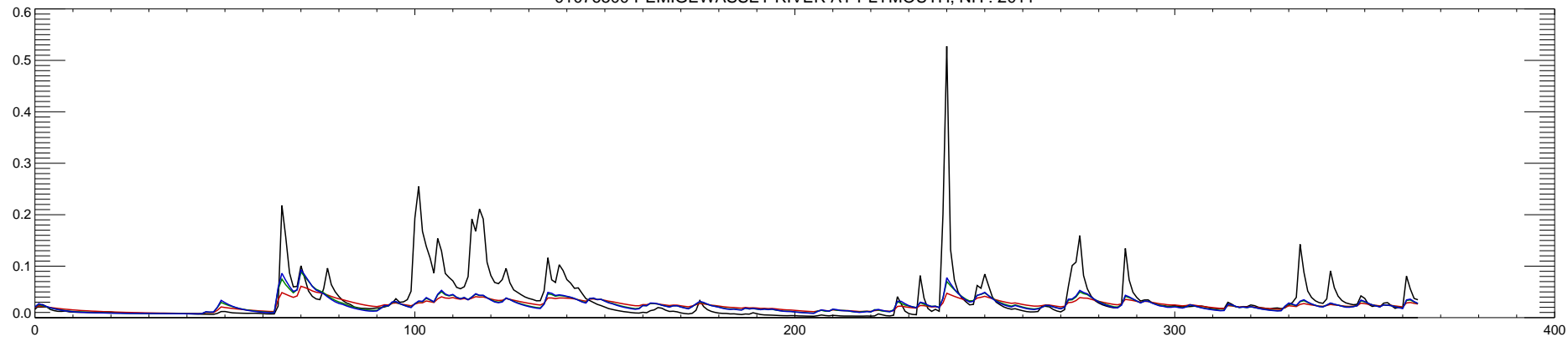
01076500 PEMIGEWASSET RIVER AT PLYMOUTH, NH : 2012
