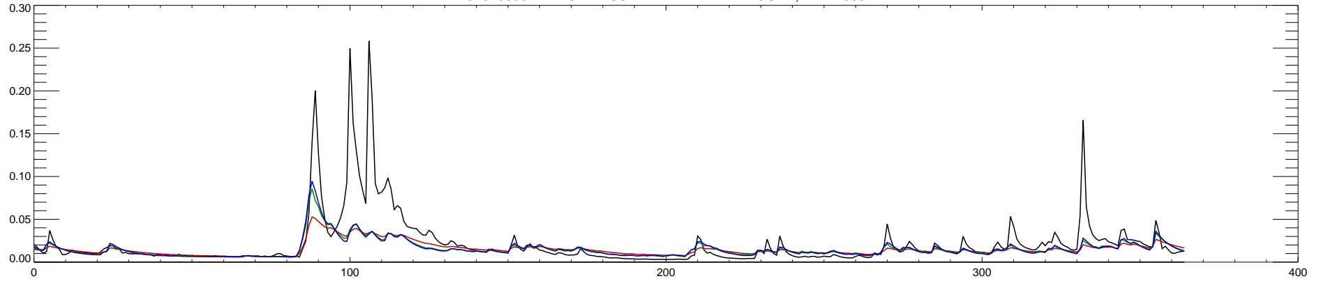
01076500 PEMIGEWASSET RIVER AT PLYMOUTH, NH : 1994
