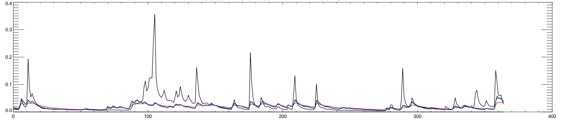
01076500 PEMIGEWASSET RIVER AT PLYMOUTH, NH : 2015
