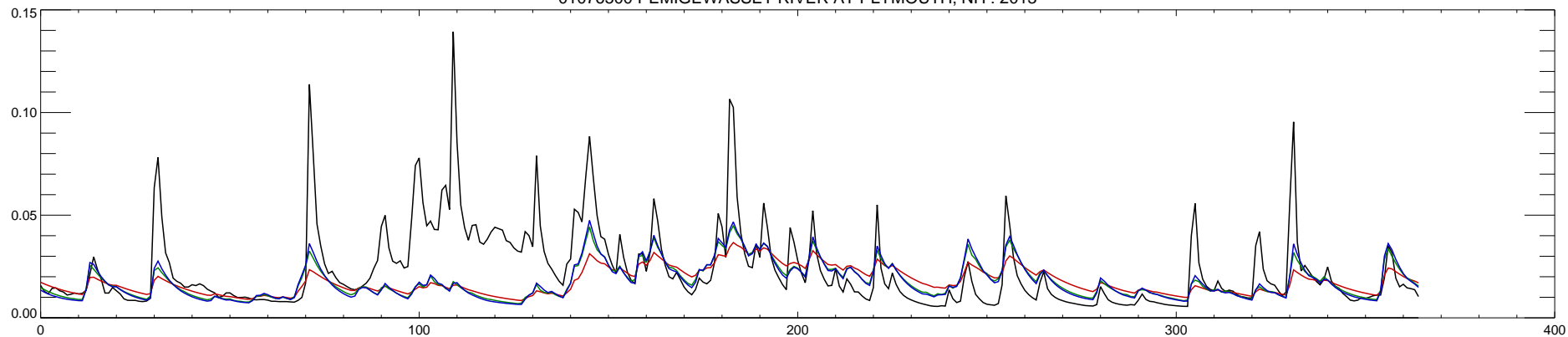
01076500 PEMIGEWASSET RIVER AT PLYMOUTH, NH : 2013
