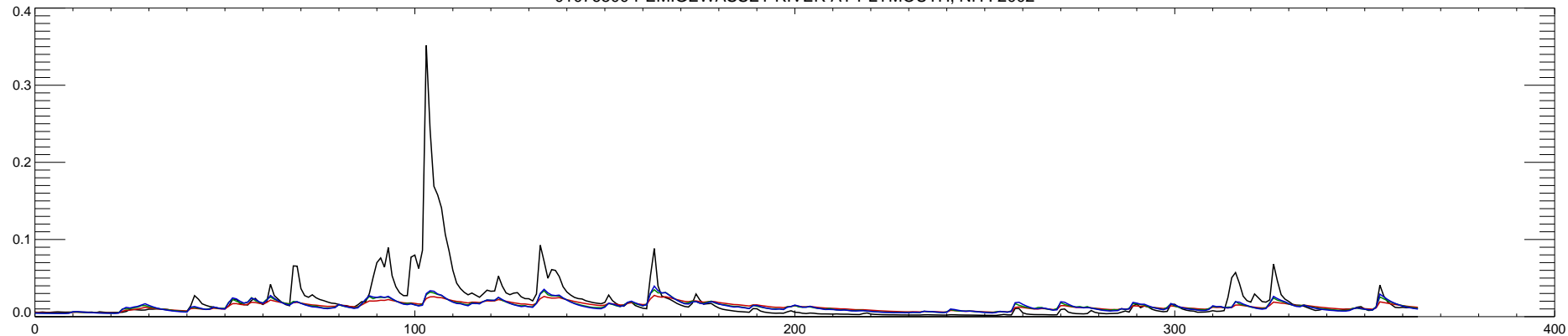
01076500 PEMIGEWASSET RIVER AT PLYMOUTH, NH : 2003
