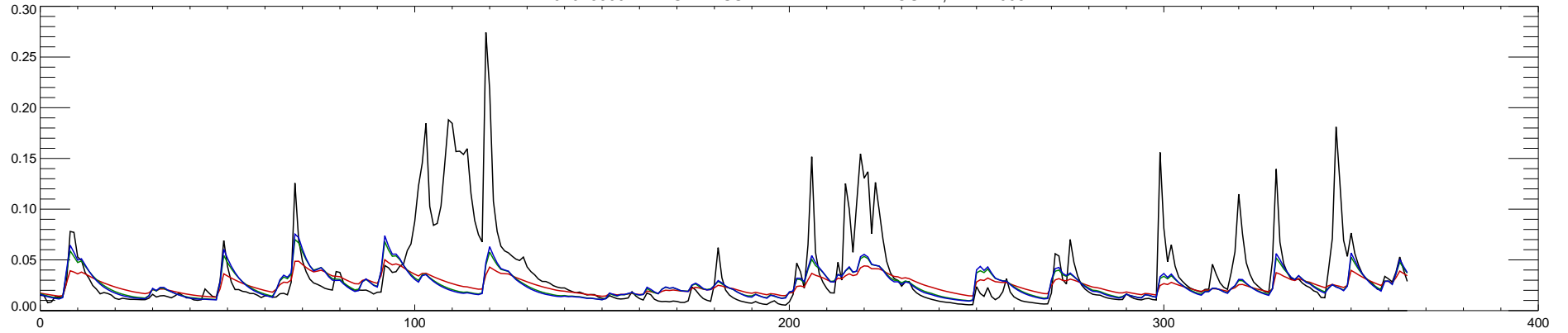
01076500 PEMIGEWASSET RIVER AT PLYMOUTH, NH : 2009
