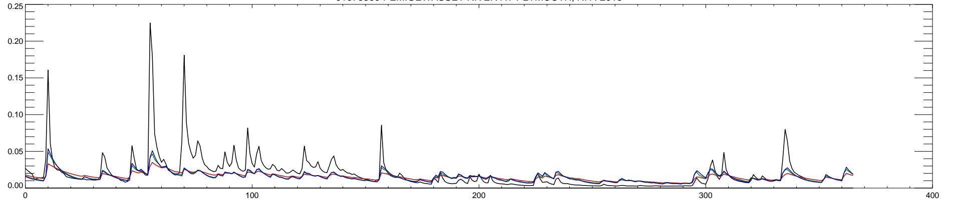
01076500 PEMIGEWASSET RIVER AT PLYMOUTH, NH : 2016
