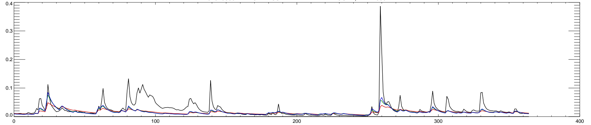
01076500 PEMIGEWASSET RIVER AT PLYMOUTH, NH : 2000
