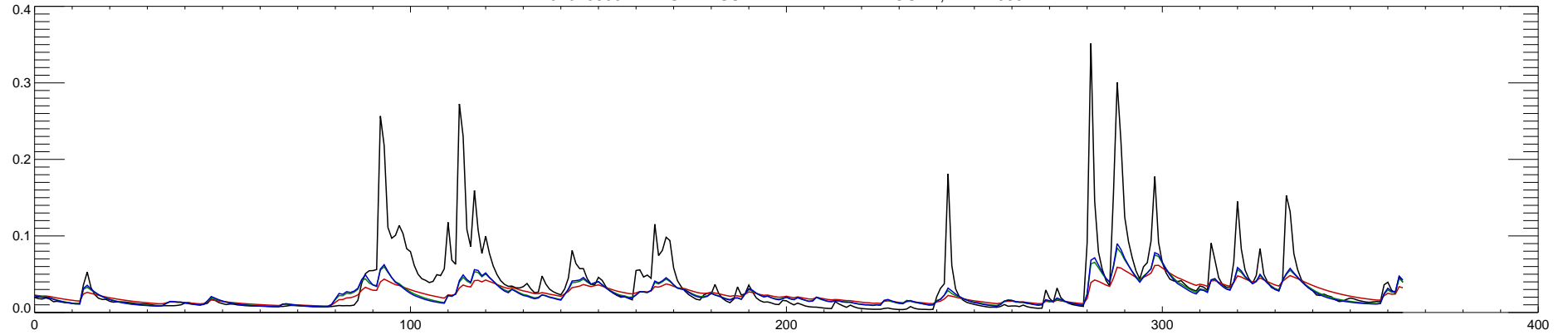
01076500 PEMIGEWASSET RIVER AT PLYMOUTH, NH : 2006
