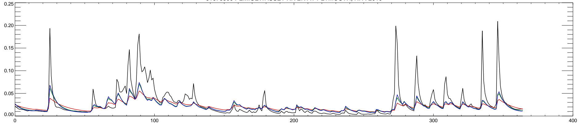
01076500 PEMIGEWASSET RIVER AT PLYMOUTH, NH : 2010
