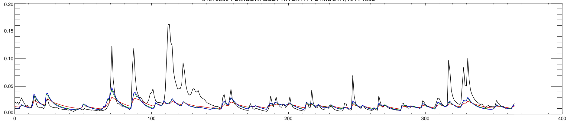
01076500 PEMIGEWASSET RIVER AT PLYMOUTH, NH : 1992
