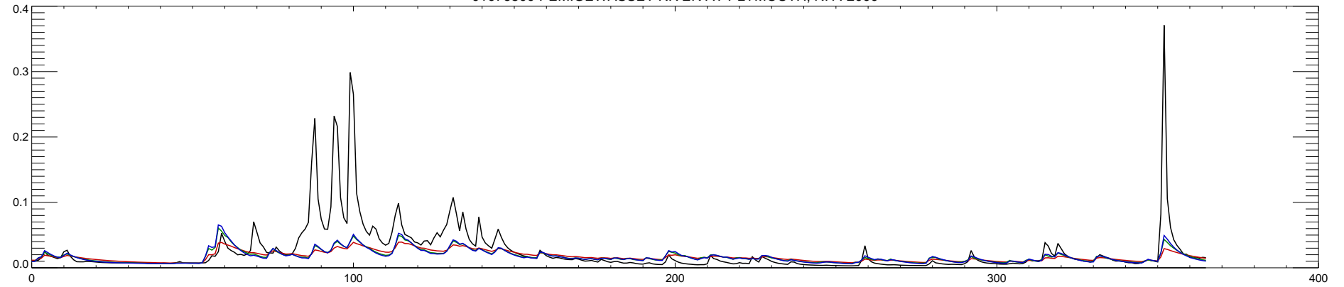
01076500 PEMIGEWASSET RIVER AT PLYMOUTH, NH : 2001
