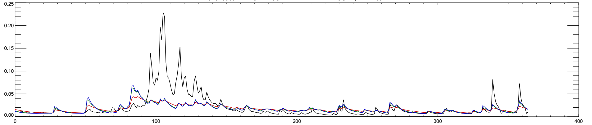
01076500 PEMIGEWASSET RIVER AT PLYMOUTH, NH : 1995
