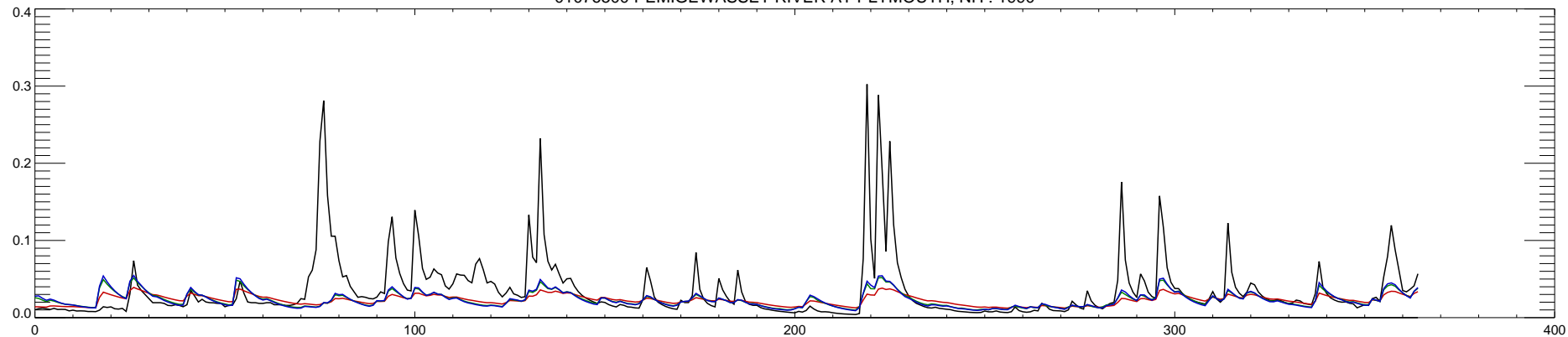
01076500 PEMIGEWASSET RIVER AT PLYMOUTH, NH : 1991
