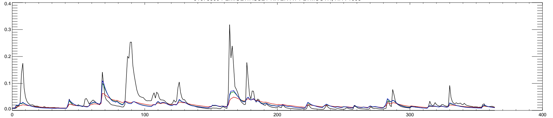
01076500 PEMIGEWASSET RIVER AT PLYMOUTH, NH : 1998
