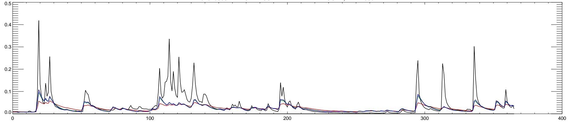
01076500 PEMIGEWASSET RIVER AT PLYMOUTH, NH : 1997
