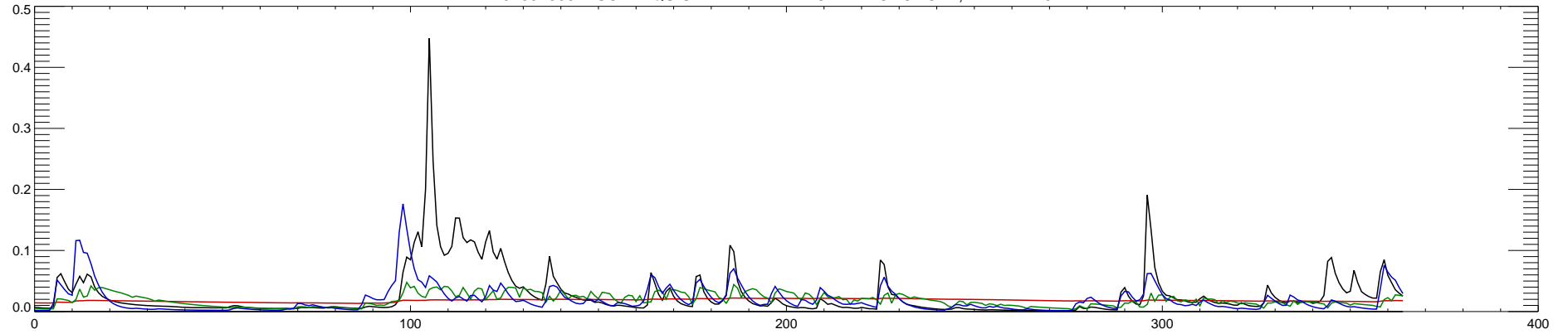
01031500 PISCATAQUIS RIVER NEAR DOVER-FOXCROFT, MAINE : 2015
