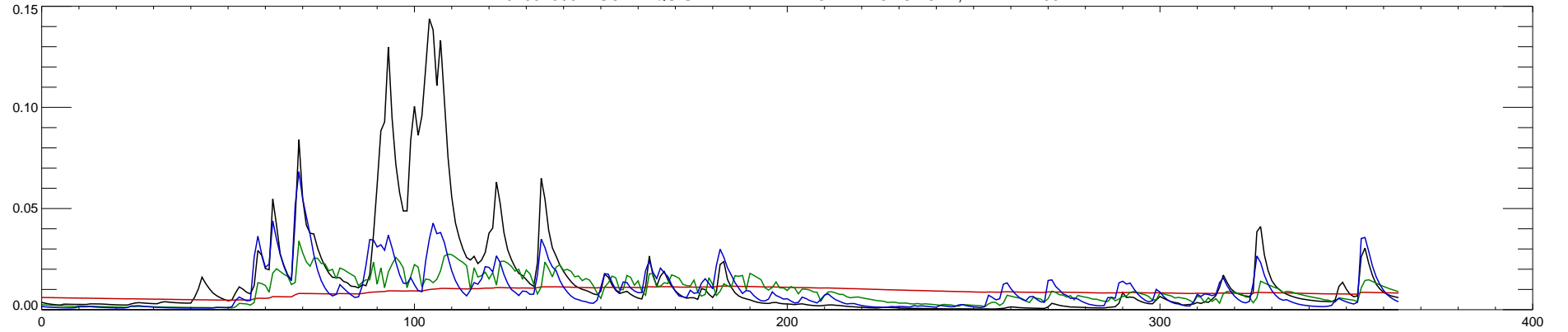
01031500 PISCATAQUIS RIVER NEAR DOVER-FOXCROFT, MAINE : 2003
