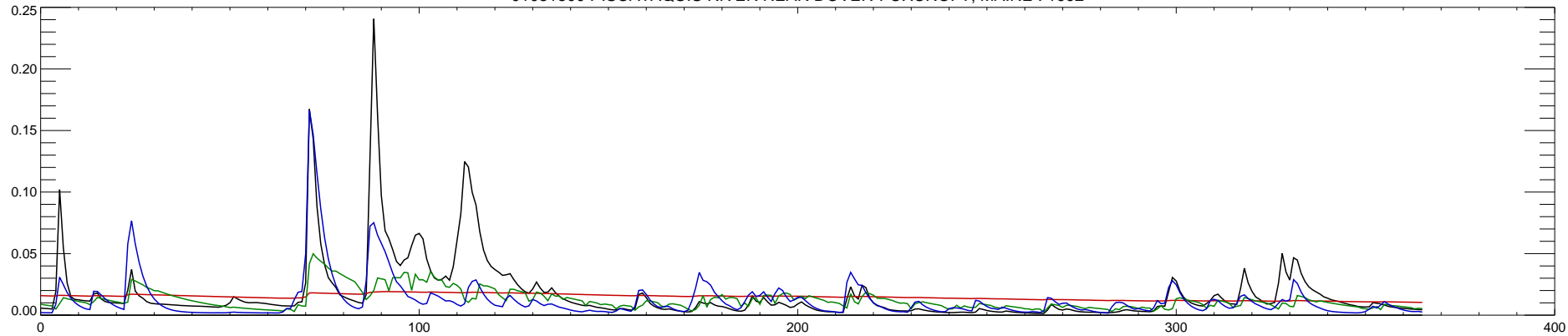
01031500 PISCATAQUIS RIVER NEAR DOVER-FOXCROFT, MAINE : 1992
