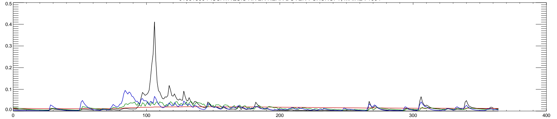
01031500 PISCATAQUIS RIVER NEAR DOVER-FOXCROFT, MAINE : 1995
