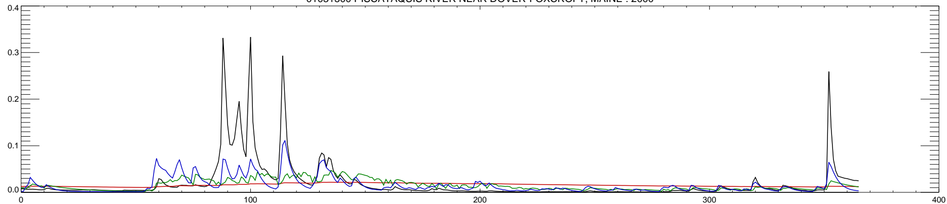
01031500 PISCATAQUIS RIVER NEAR DOVER-FOXCROFT, MAINE : 2001
