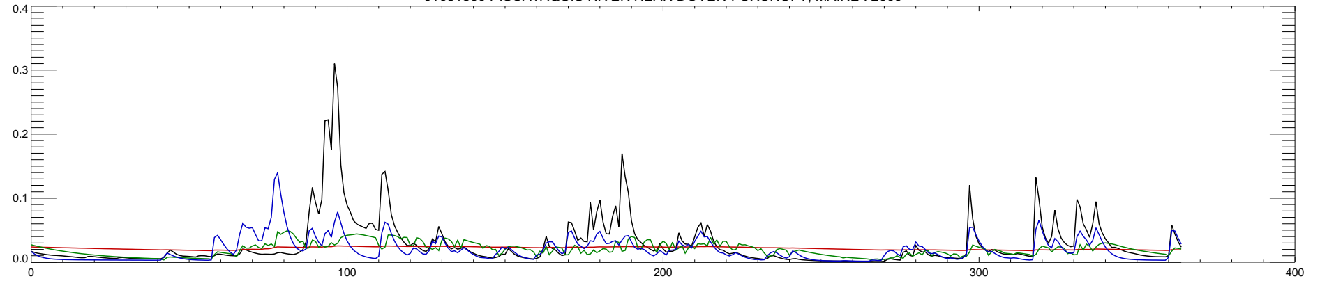
01031500 PISCATAQUIS RIVER NEAR DOVER-FOXCROFT, MAINE : 2010
