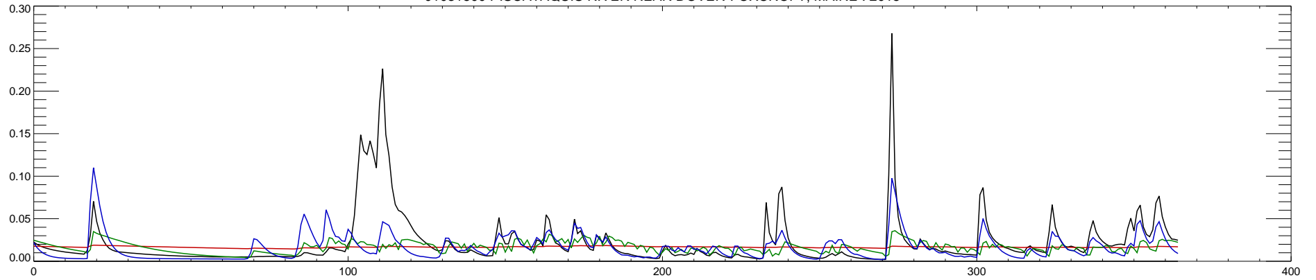
01031500 PISCATAQUIS RIVER NEAR DOVER-FOXCROFT, MAINE : 2016
