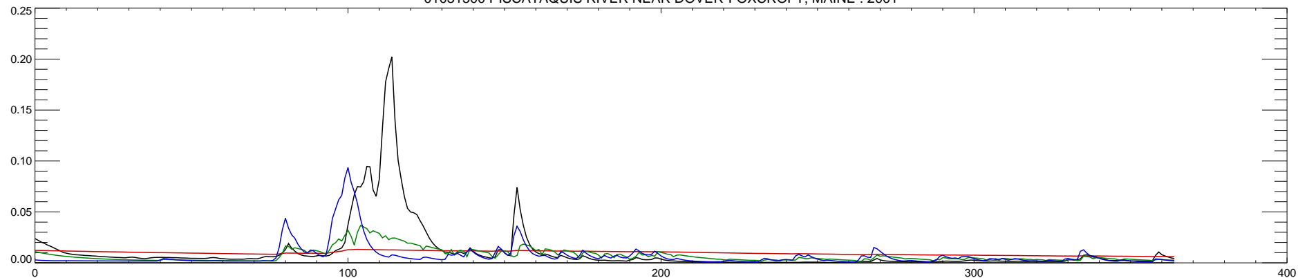
01031500 PISCATAQUIS RIVER NEAR DOVER-FOXCROFT, MAINE : 2001
