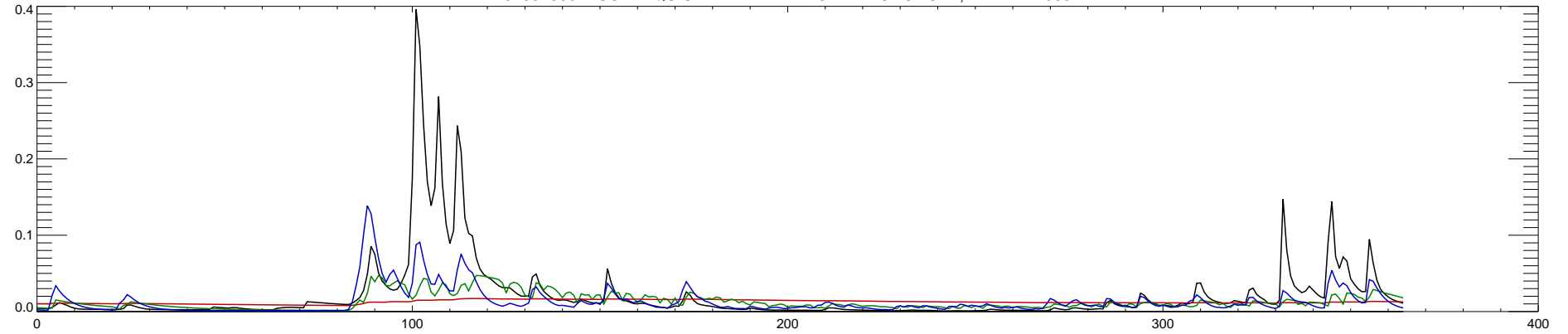
01031500 PISCATAQUIS RIVER NEAR DOVER-FOXCROFT, MAINE : 1994
