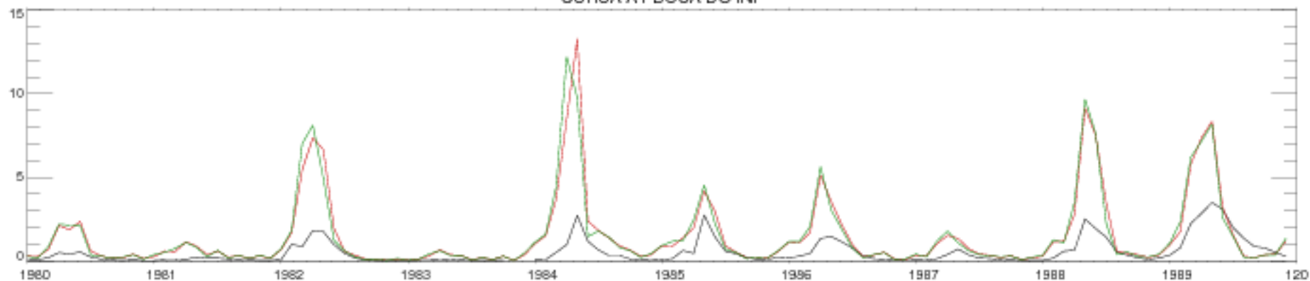
CURVA AT BOCA DO INF
