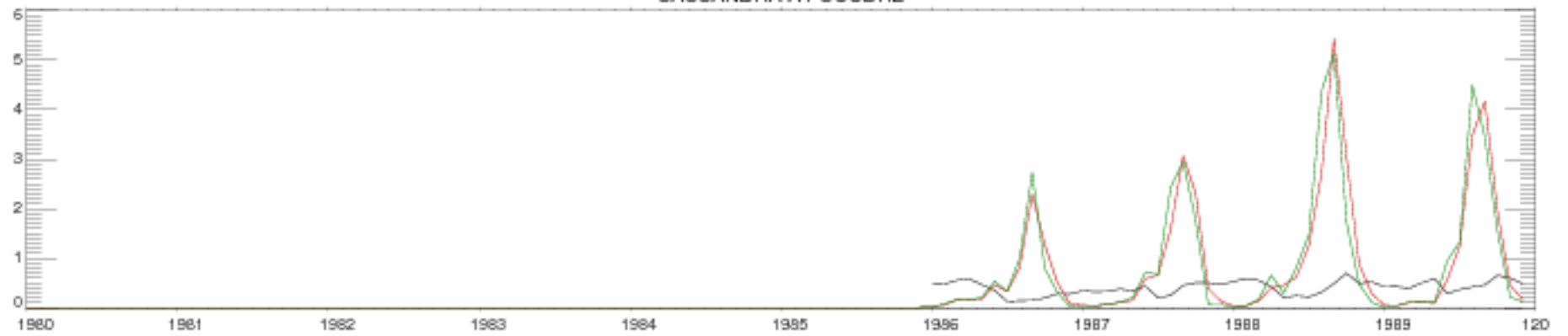
SASSANDRA AT SOUBRE
