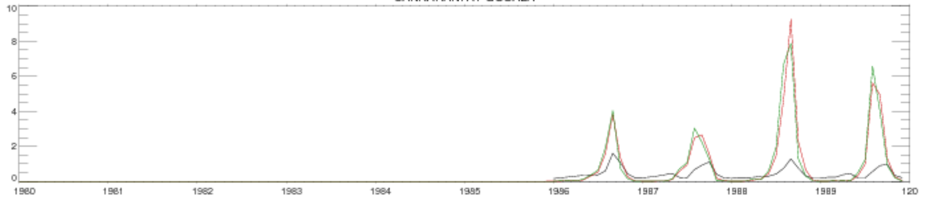
SANKARANI AT GOJALA
