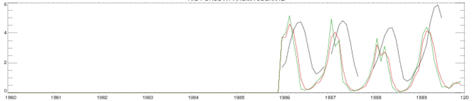
RIO PURUS AT ARUMA-JUSANTE
