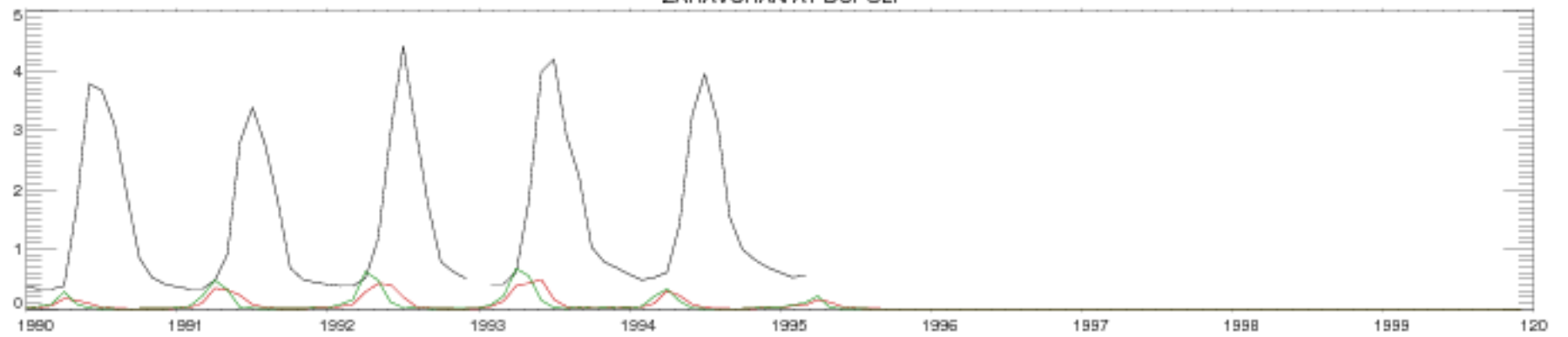
ZARAVCHAN AT DUPULI
