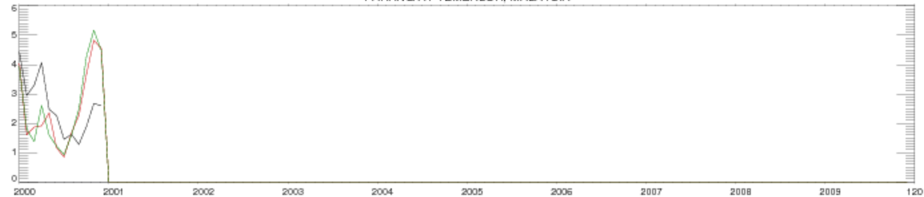
PAHANG AT TEMERLOH, MALAYSIA
