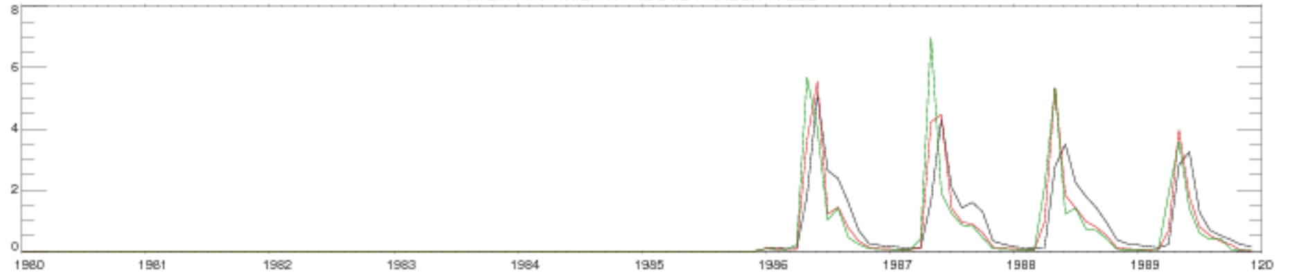
STEWART RIVER AT ABOVE FRASER FALLS
