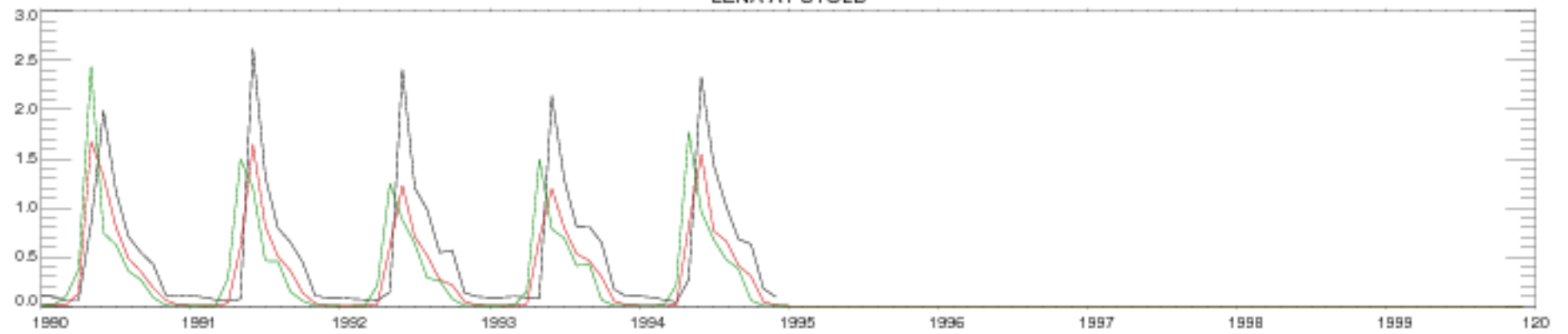
LENA AT STOLB
