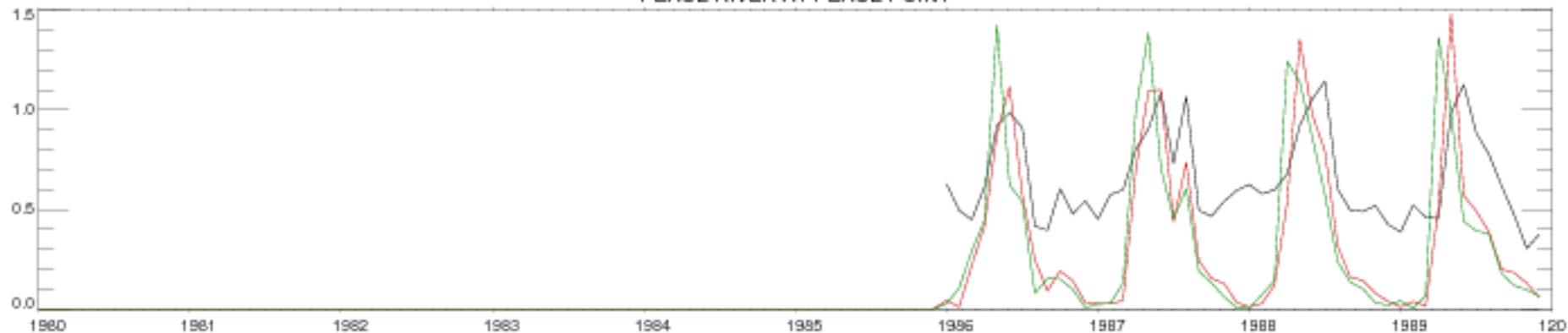
PEACE RIVER AT PEACE POINT
