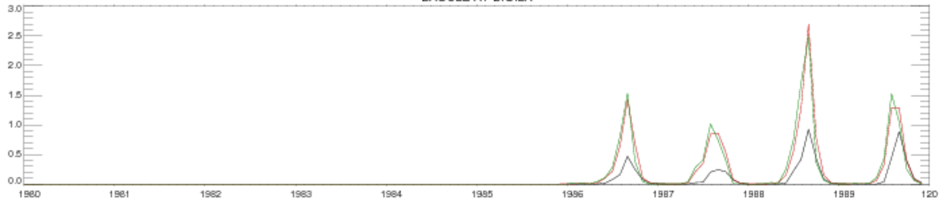
BAOULE AT DIOILA
