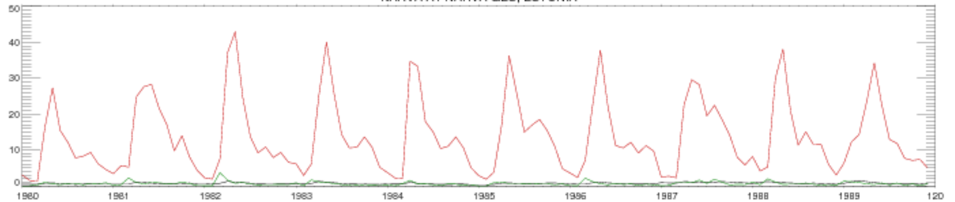
NARVA AT NARVA GES, ESTONIA
