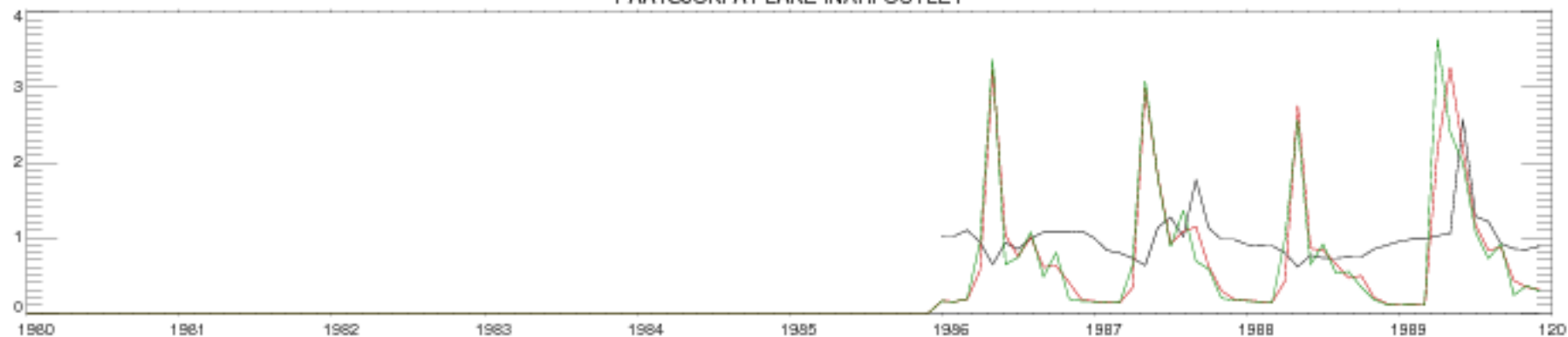
PAATSJOKI AT LAKE INARI OUTLET
