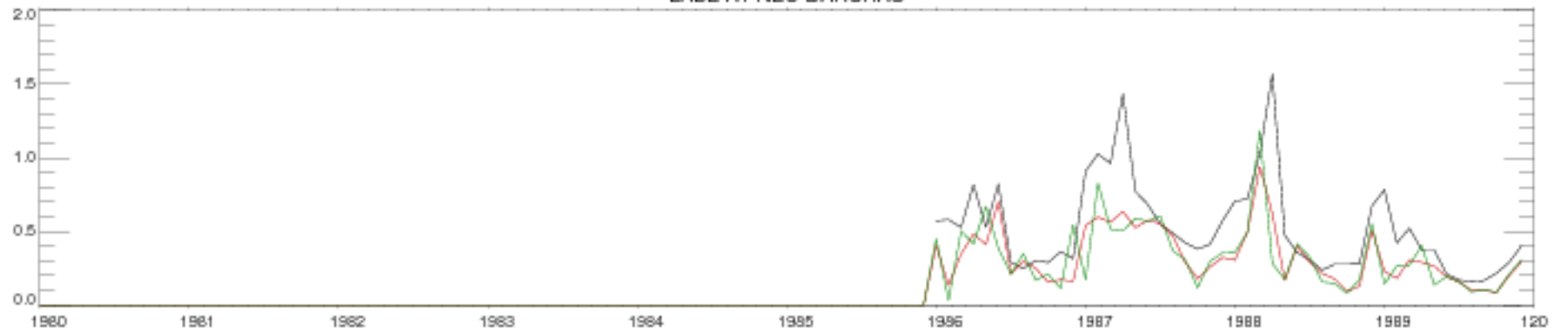
LABE AT NEU-DARCHAU
