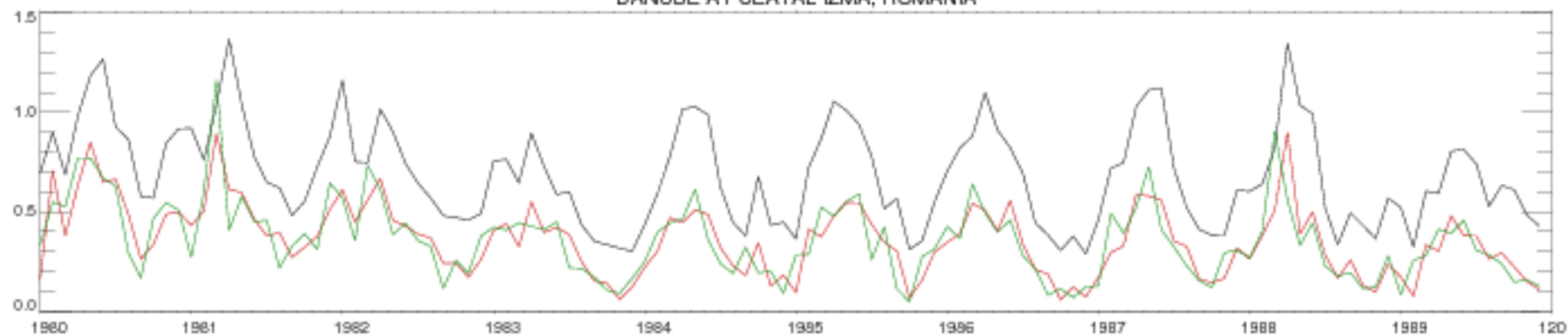
DANUBE AT CEATAL IZMA, ROMANIA
