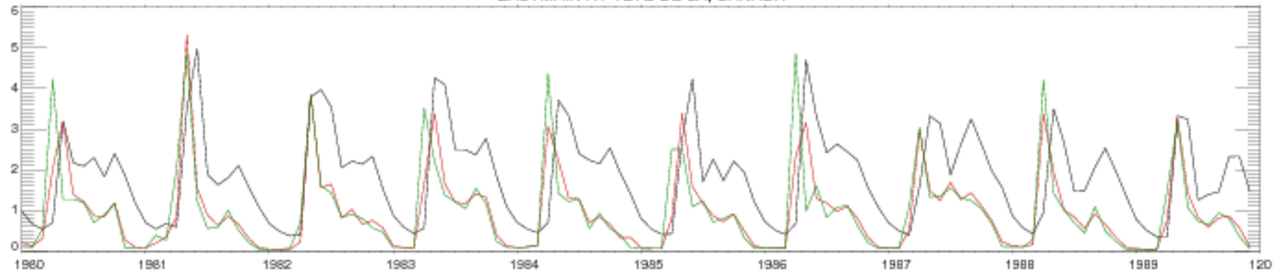
EASTMAIN AT TETE DE LA, CANADA
