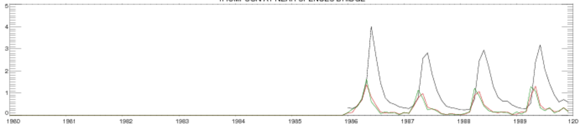
THOMPSON AT NEAR SPENCES BRIDGE
