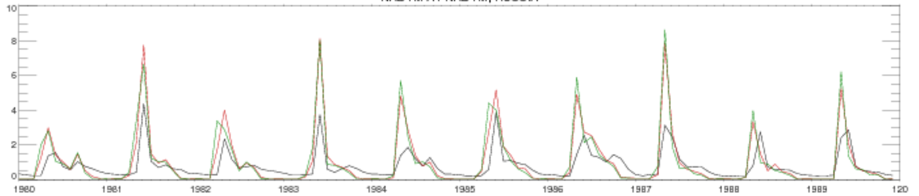
NADYM AT NADYM, RUSSIA
