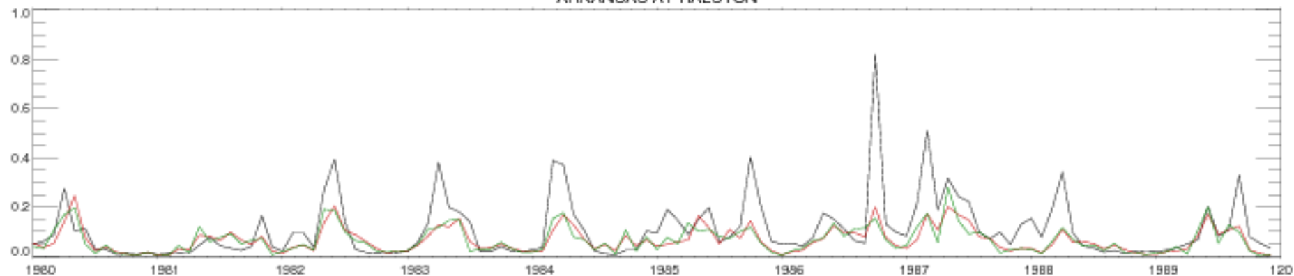
ARKANSAS AT RALSTON
