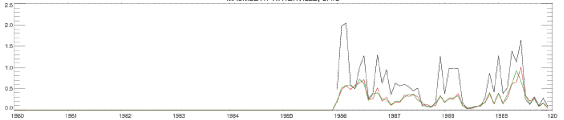
MAUMEE AT WATERVILLE, OHIO
