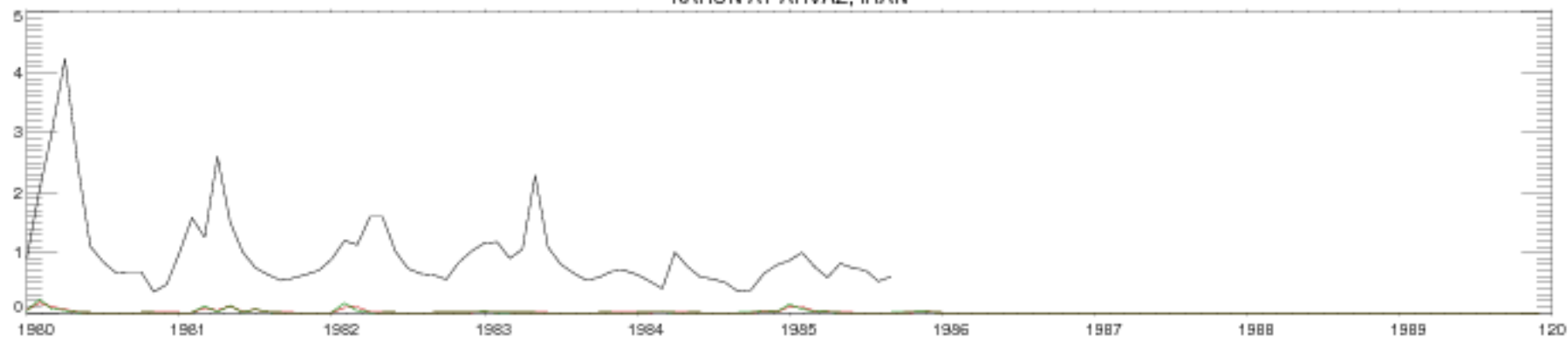
KARUN AT AHVAZ, IRAN
