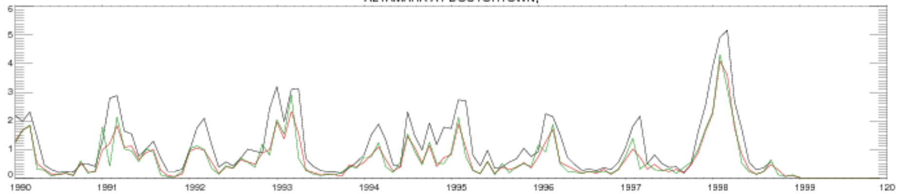
ALTAMAHA AT DOCTORTOWN,
