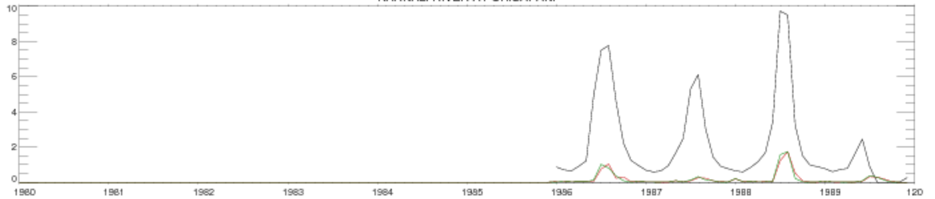
KARNALI RIVER AT CHISAPANI
