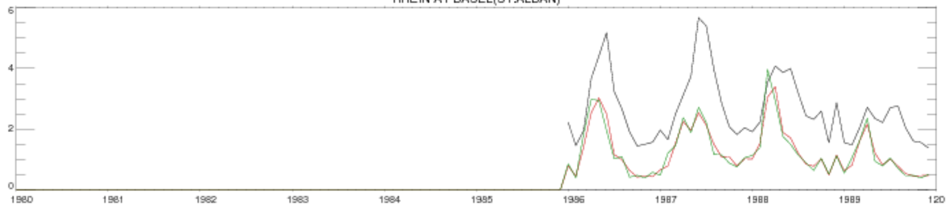
RHEIN AT BASEL(ST.ALBAN)
