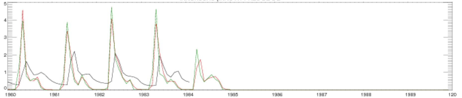
INNUKSUAC (INNU AT PRES DE L'E
