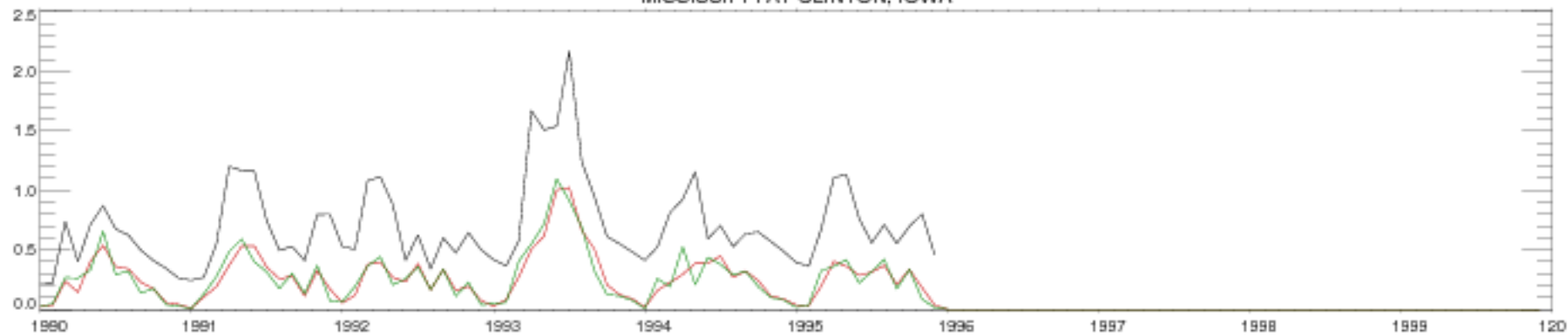
MISSISSIPPI AT CLINTON, IOWA
