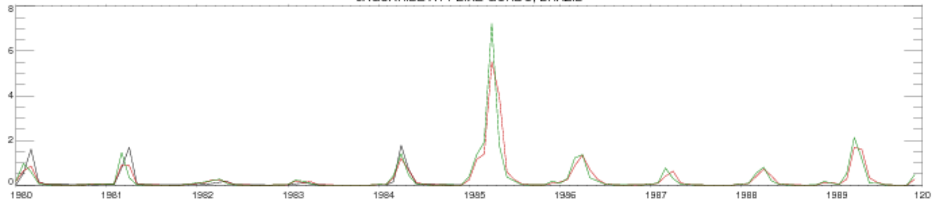
JAGUARIBE AT PEIXE GORDO, BRAZIL
