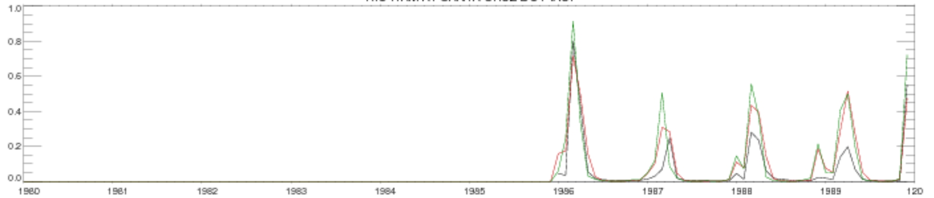
RIO ITAM AT SANTA CRUZ DO PIAUI
