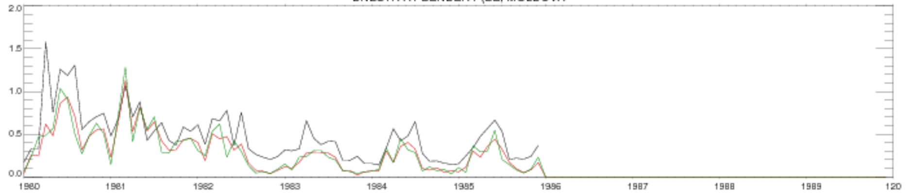
DNESTR AT BENDERY (BE, MOLDOVA)
