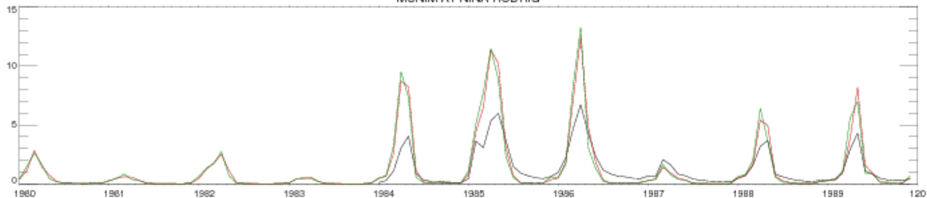
MUNIM AT NINA RODRIG
