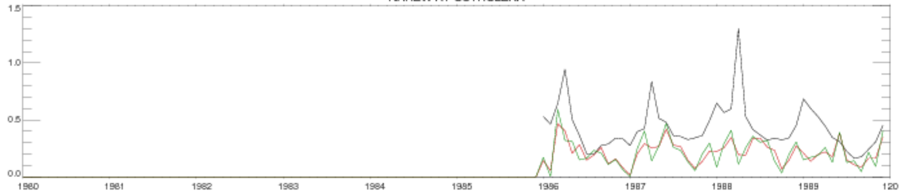
NAREW AT OSTROLEKA
