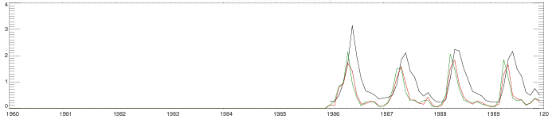
FRASER RIVER AT MARGUERITE
