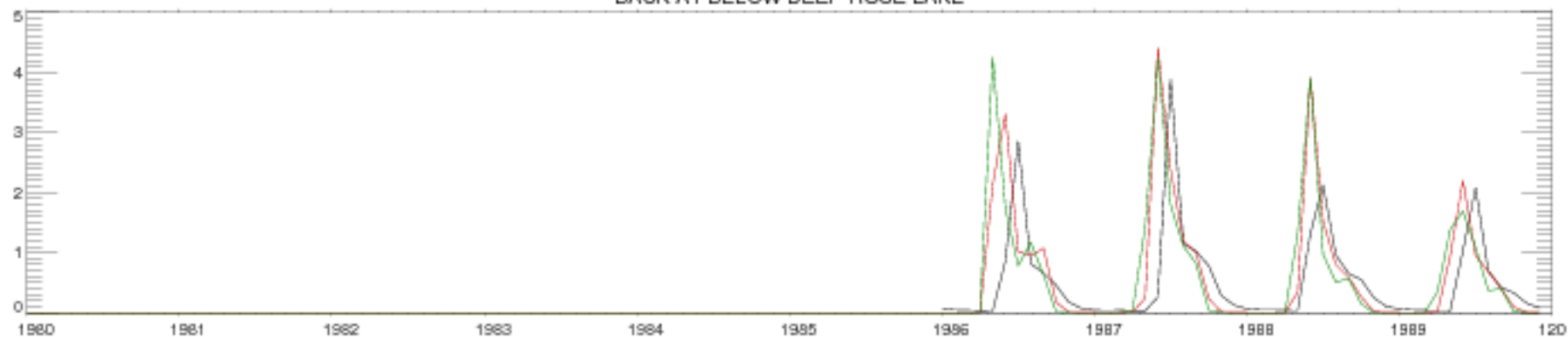
BACK AT BELOW DEEP ROSE LAKE
