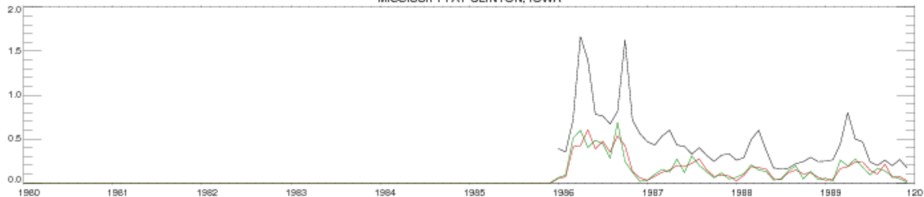
MISSISSIPPI AT CLINTON, IOWA
