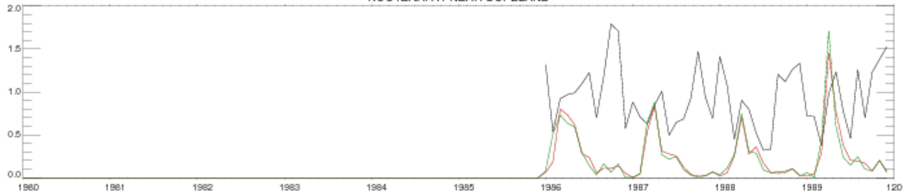
KOOTENAI AT NEAR COPELAND
