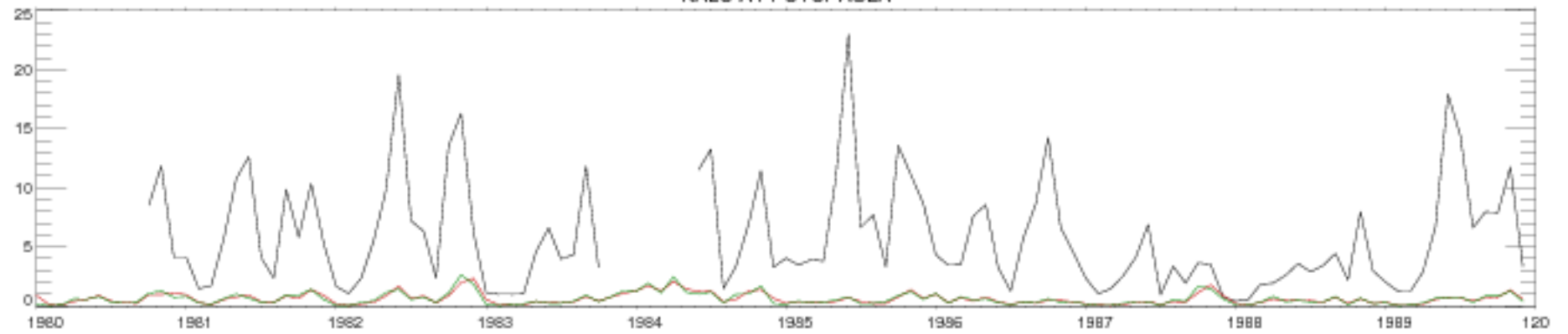
KALU AT PUTUPAULA
