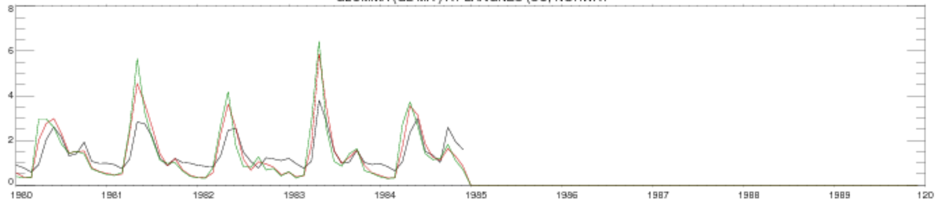
GLOMMA (GL MA ) AT LANGNES (SO, NORWAY
