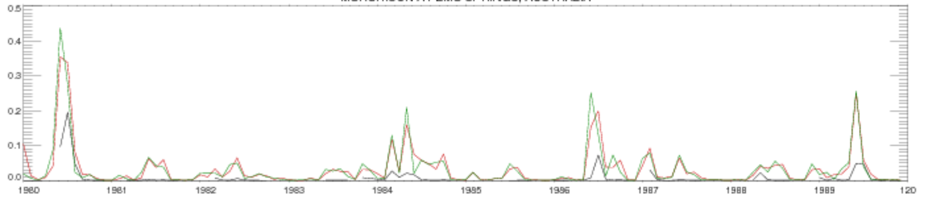
MURCHISON AT EMU SPRINGS, AUSTRALIA
