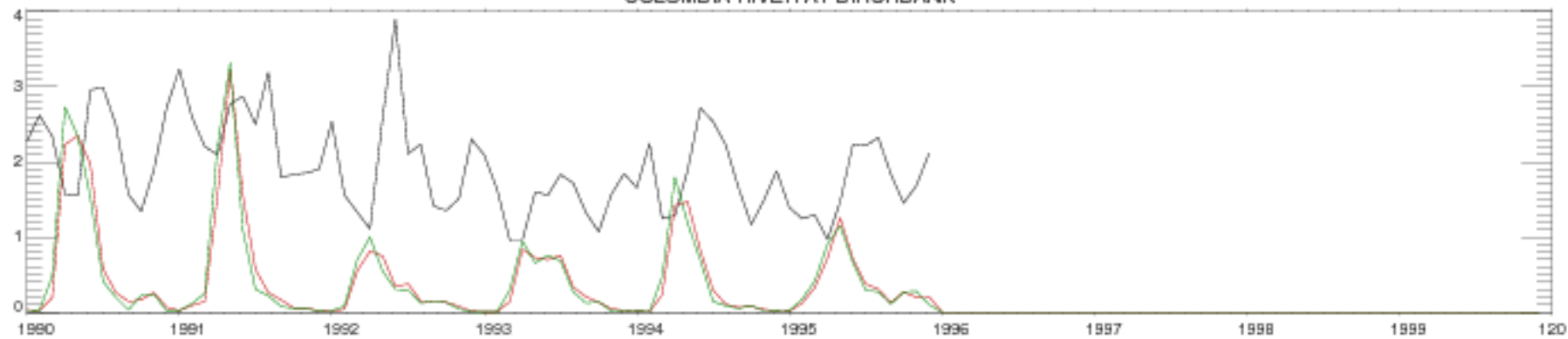
COLUMBIA RIVER AT BIRCHBANK
