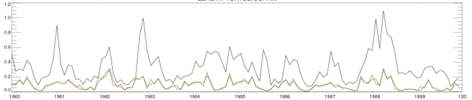
EBRO AT TORTOSA, SPAIN
