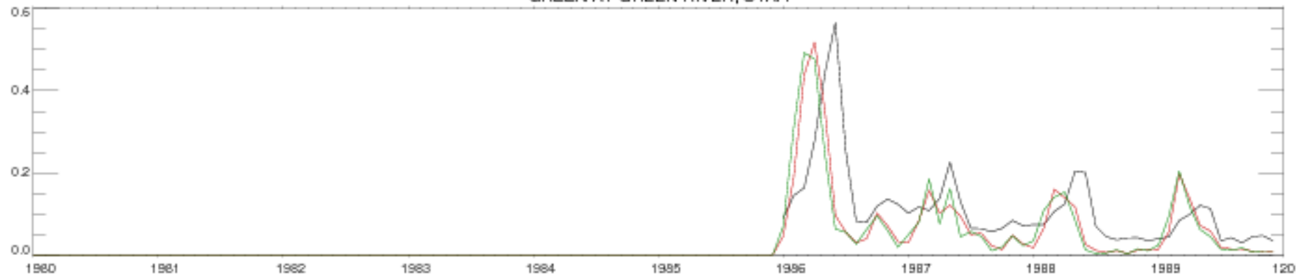
GREEN AT GREEN RIVER, UTAH
