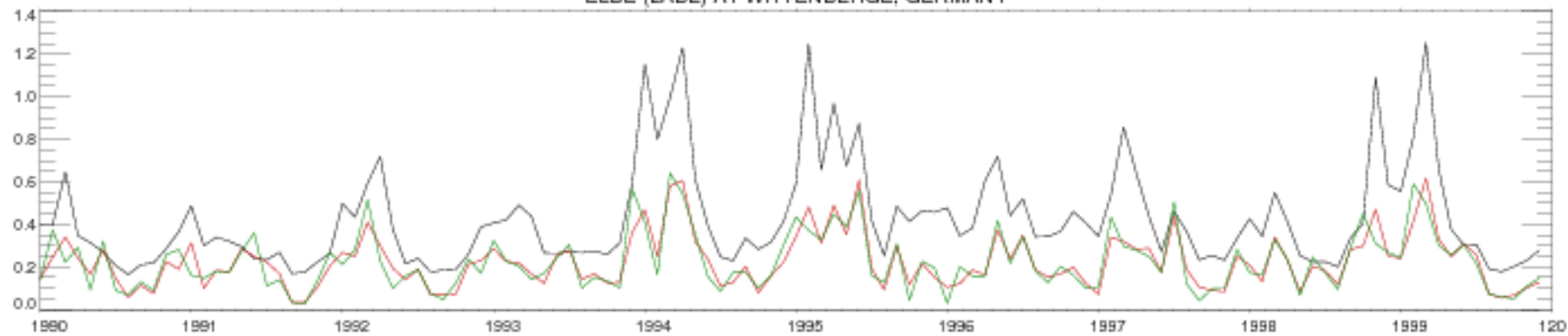
ELBE (LAE) AT WITTENBERGE, GERMANY
