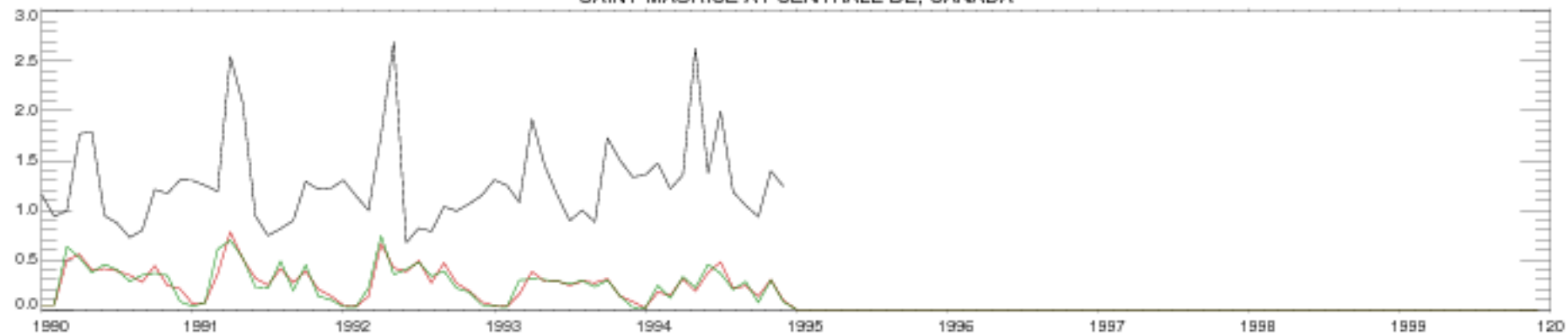
SAINT-MAURICE AT CENTRALE DE, CANADA
