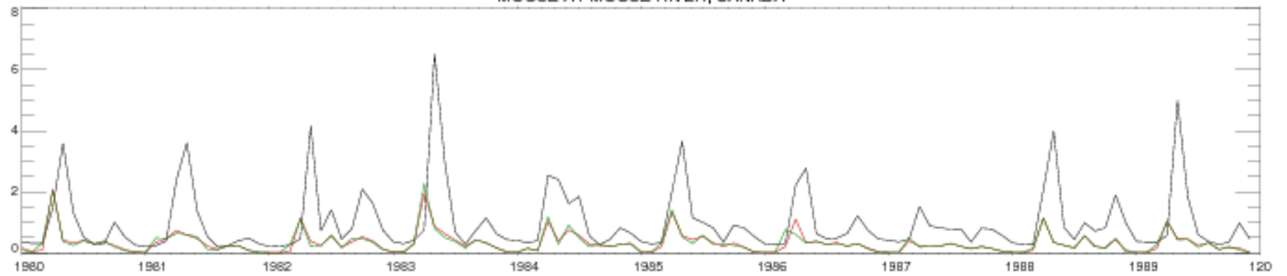
MOOSE AT MOOSE RIVER, CANADA
