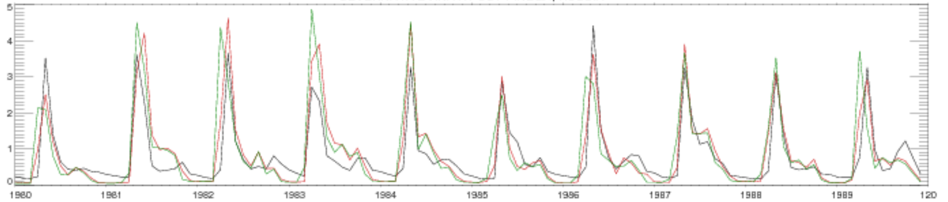
SEVERNAYA DVINA AT UST PINEGA, RUSSIA
