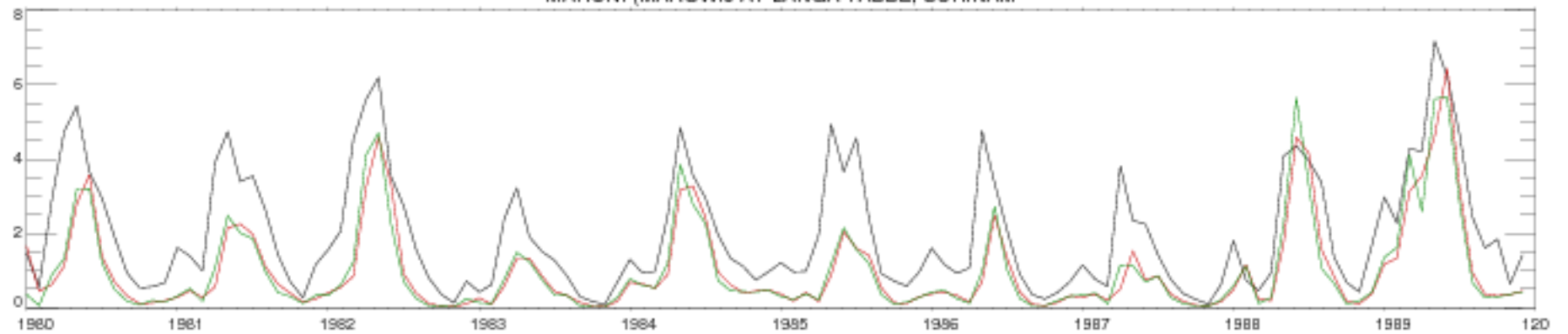
MARONI (MAROWIJ AT LANGA TABBE, SURINAM)
