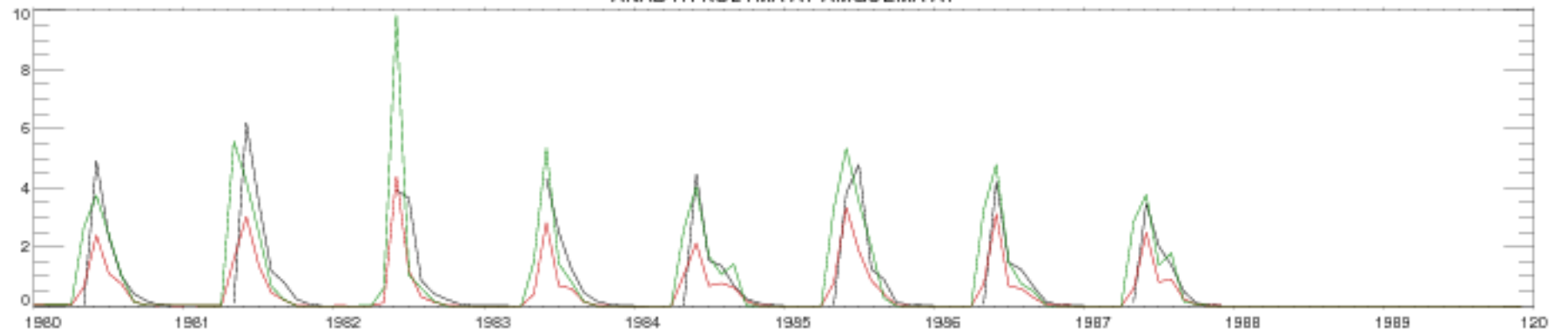
ANADYR KOLYMA AT AMGUEMA AT
