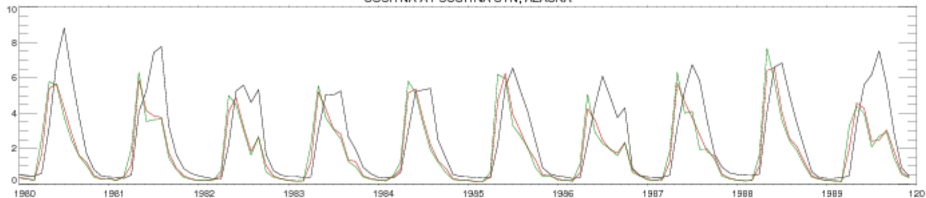
SUSITNA AT SUSITNA STN, ALASKA
