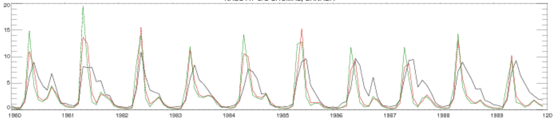
NASS AT U/S SHUMAL, CANADA
