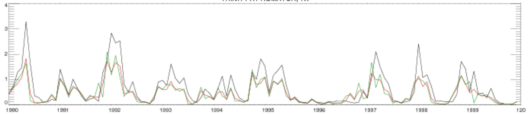
TRINITY AT ROMAYOR, TX
