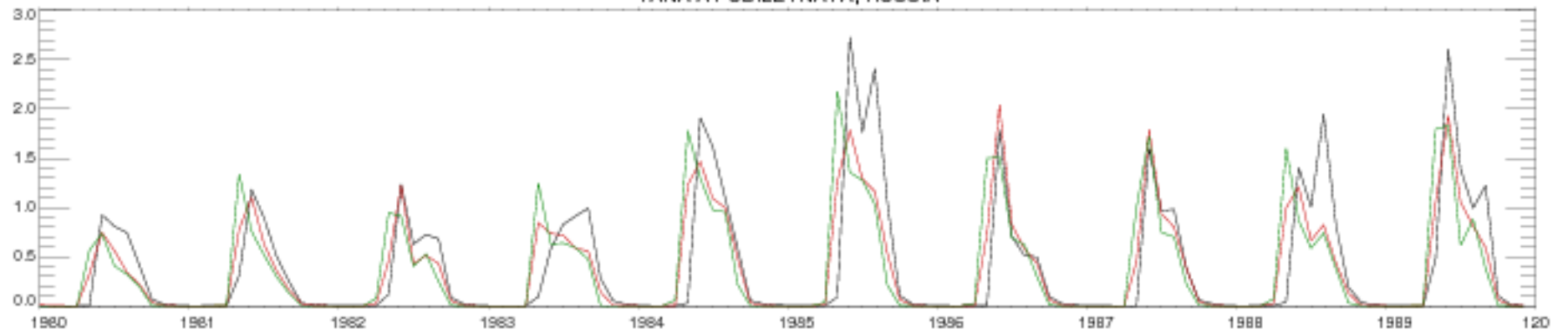
YANA AT UBILEYNAYA, RUSSIA
