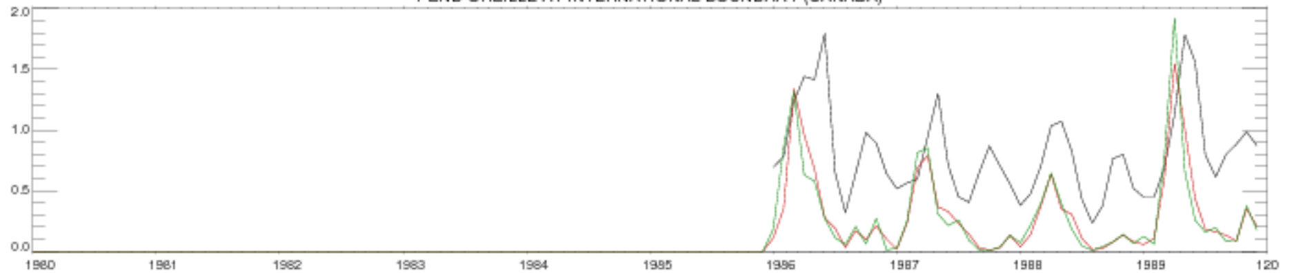
PEND OREILLE AT INTERNATIONAL BOUNDARY (CANADA)
