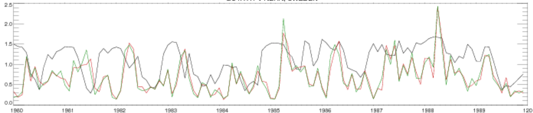
GOTA AT V NERN, SWEDEN
