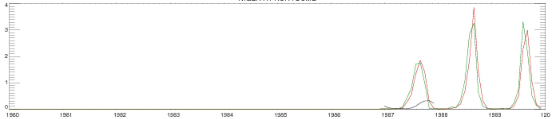
NIGER AT KORYOUME
