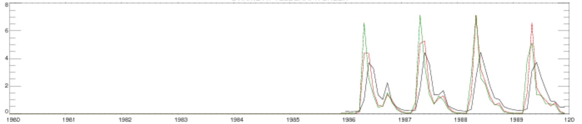
STIKINE AT TELEGRAPH CREEK
