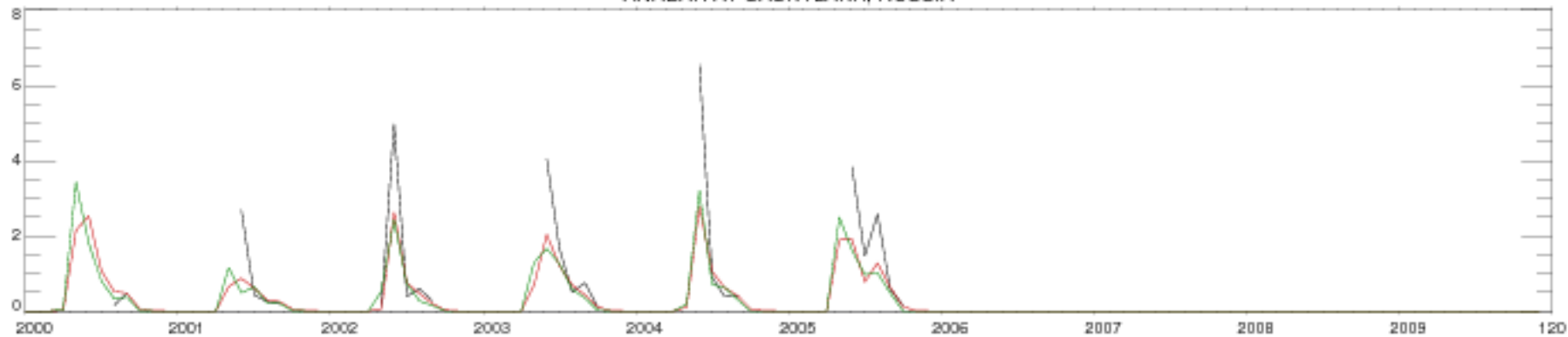
ANABAR AT SASKYLAKH, RUSSIA
