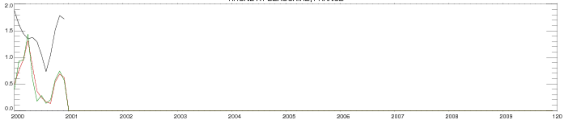
RHONE AT BEAUCAIRE, FRANCE
