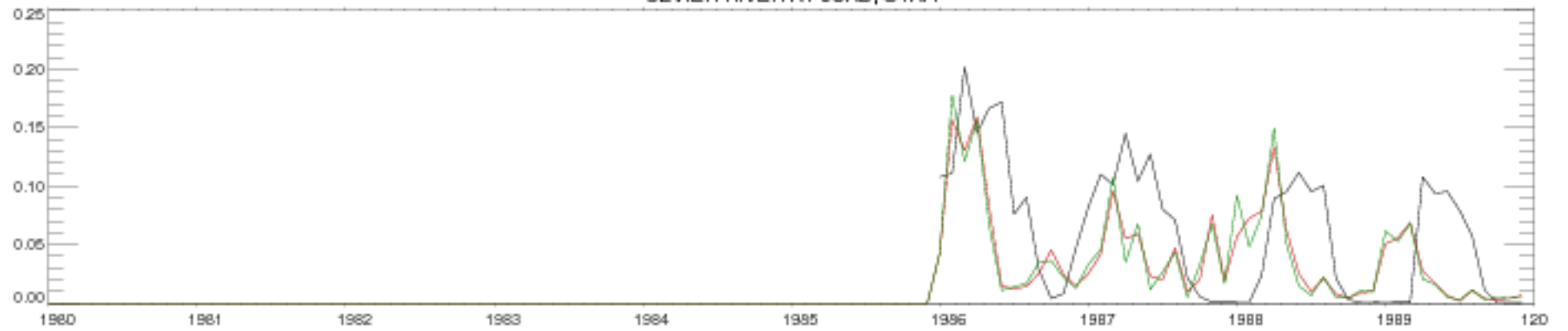
SEVIER RIVER AT JUAB, UTAH
