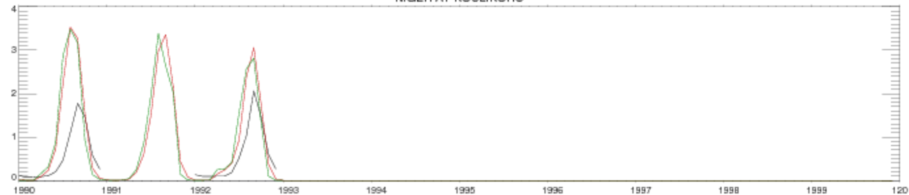
NIGER AT KOULIKORO
