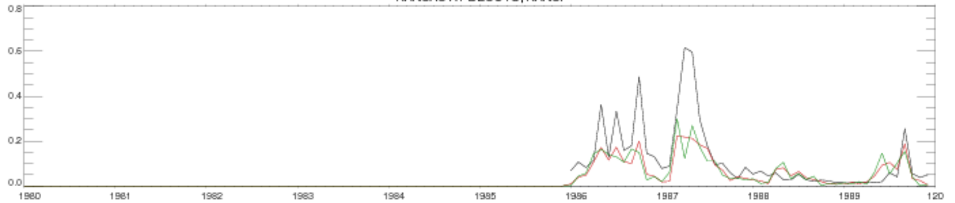
KANSAS AT DESOTO, KANS.
