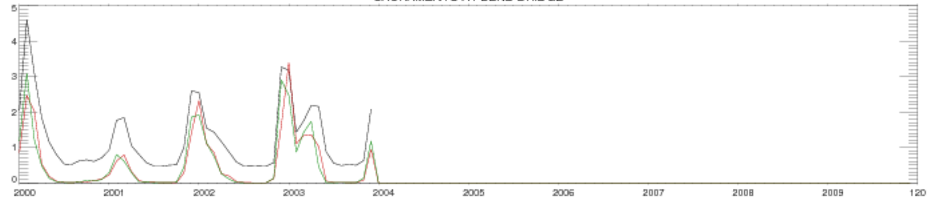
SACRAMENTO AT BEND BRIDGE
