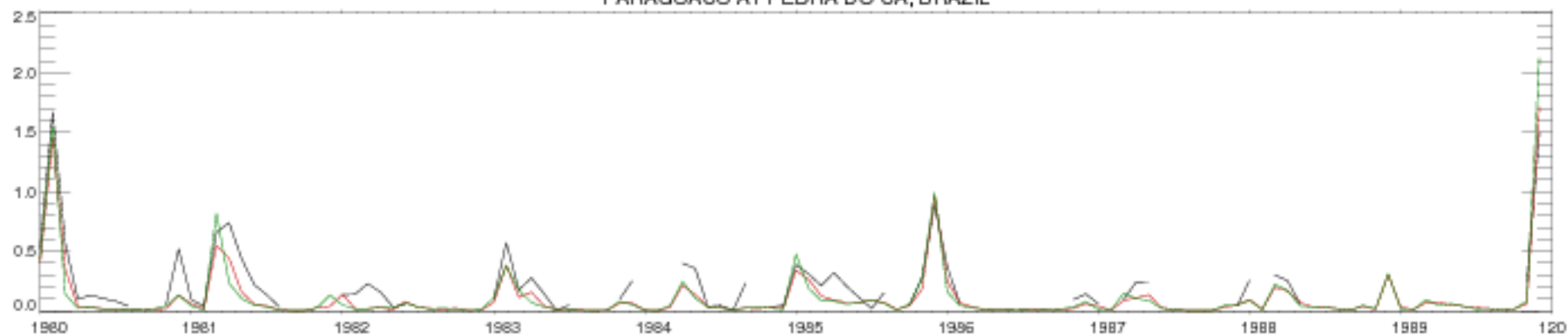
PARAGUACU AT PEDRA DO CA, BRAZIL
