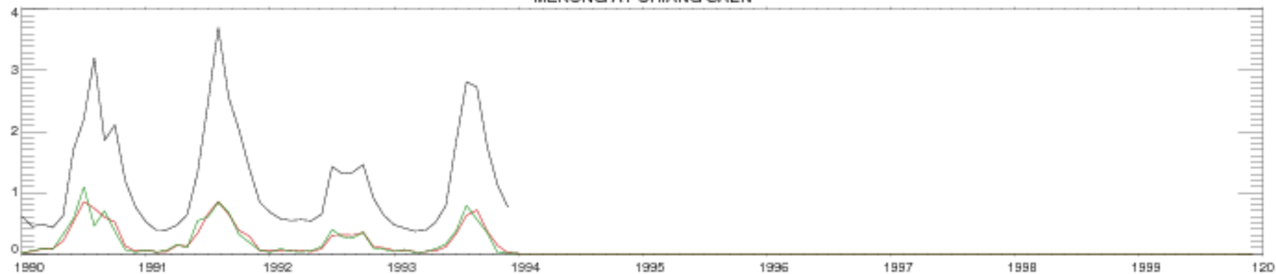
MEKONG AT CHIANG SAEN
