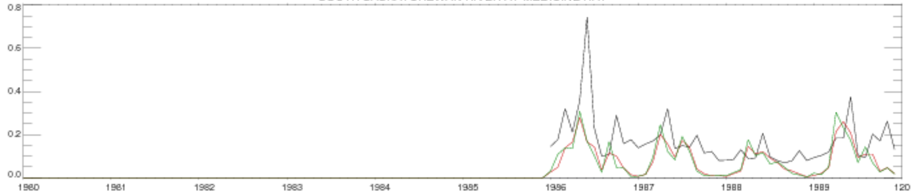
SOUTH SASKATCHEWAN RIVER AT MEDICINE HAT
