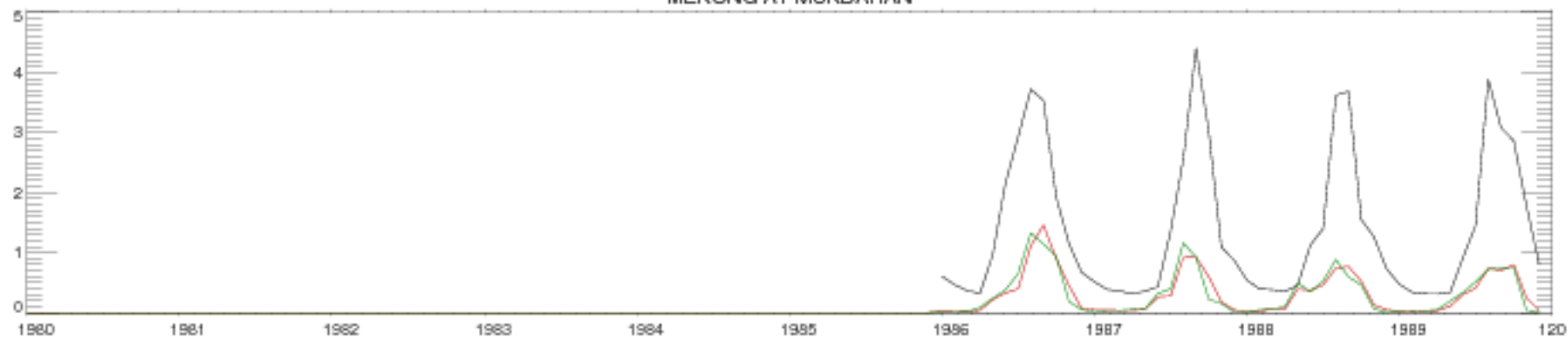
MEKONG AT MUKDAHAN
