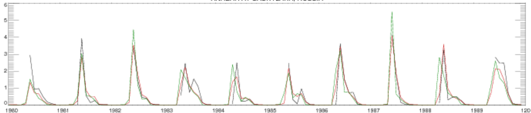
ANABAR AT SASKYLAKH, RUSSIA
