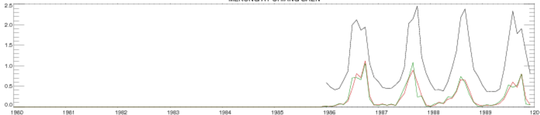
MEKONG AT CHIANG SAEN
