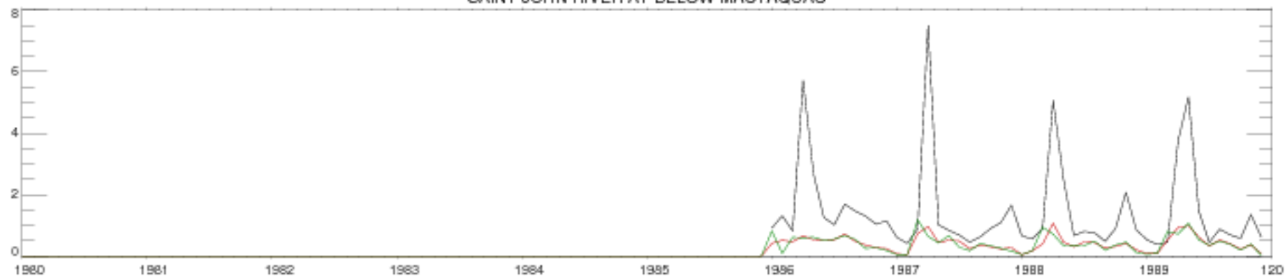
SAINT JOHN RIVER AT BELOW MACTAQUAC
