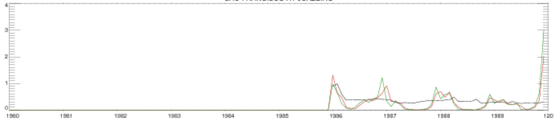
SAO FRANCISCO AT JUAZEIRO
