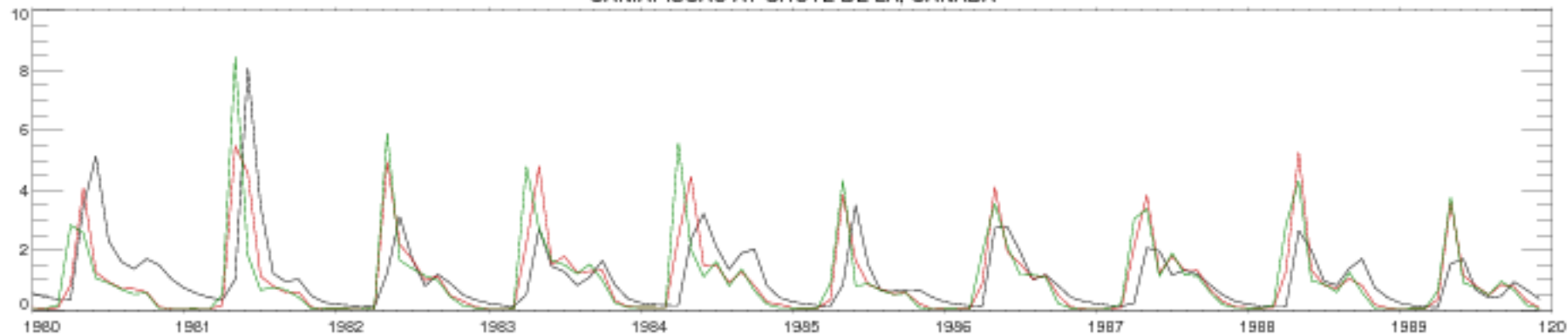
CANIAPISCAU AT CHUTE DE LA, CANADA
