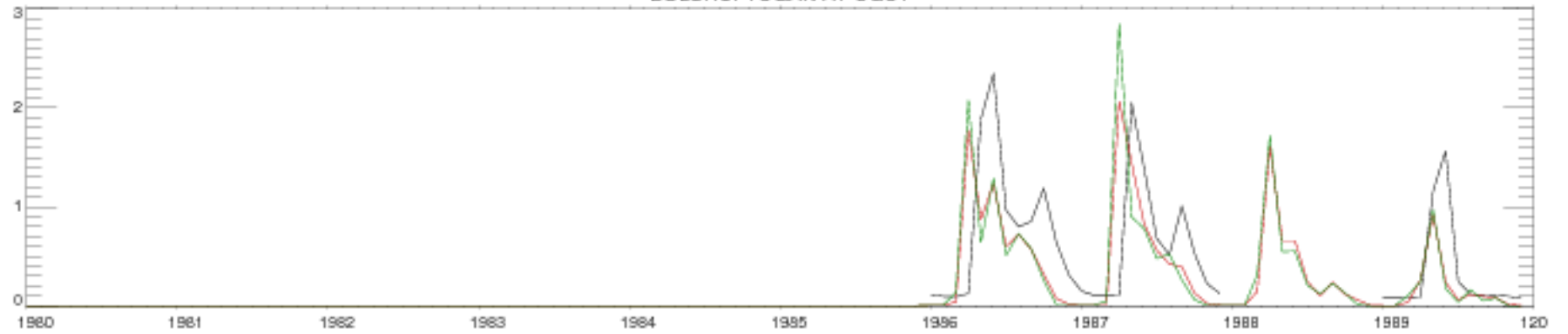
BOLSHOI YUGAN AT UGUT
