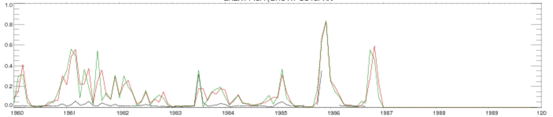
GREAT FISH (GRO AT OUTSPAN)
