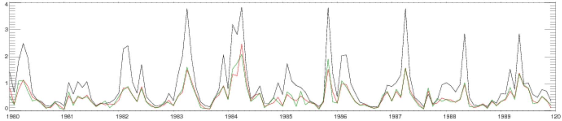
POTOMAC AT AT POINT OF ROCKS
