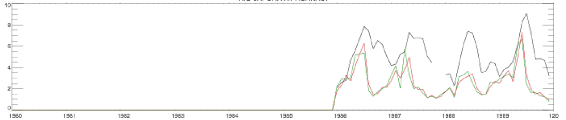
RIO JAPURA AT ACANAU
