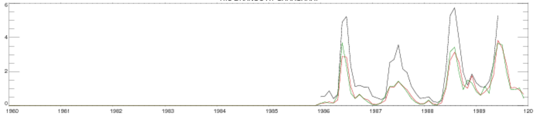
RIO BRANCO AT CARACARAI
