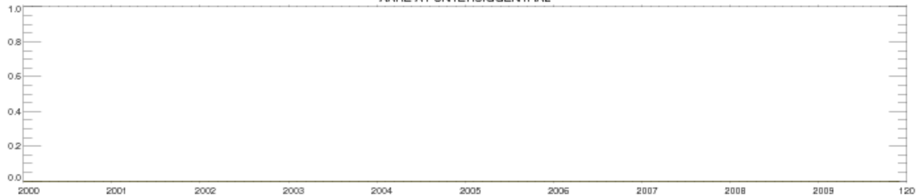
AARE AT UNTERSIGGENTHAL
