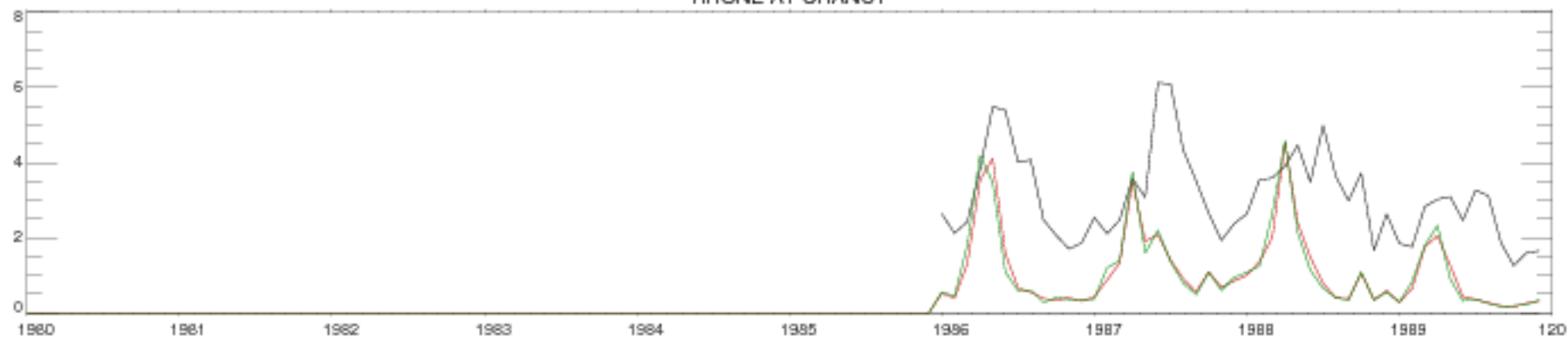
RHONE AT CHANCY
