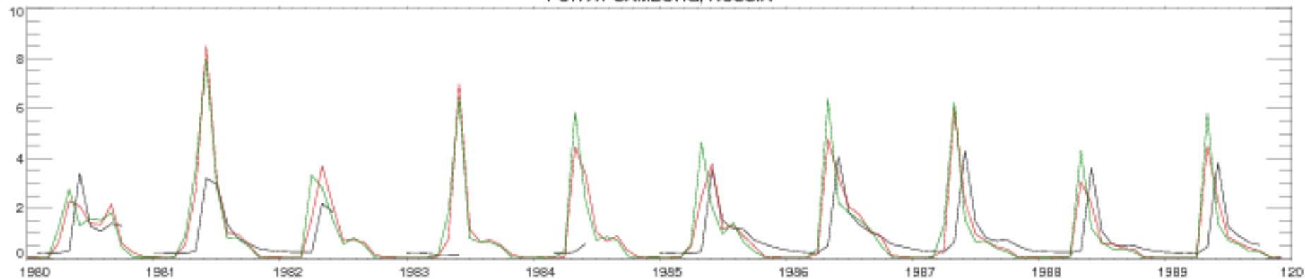
PUR AT SAMBURG, RUSSIA
