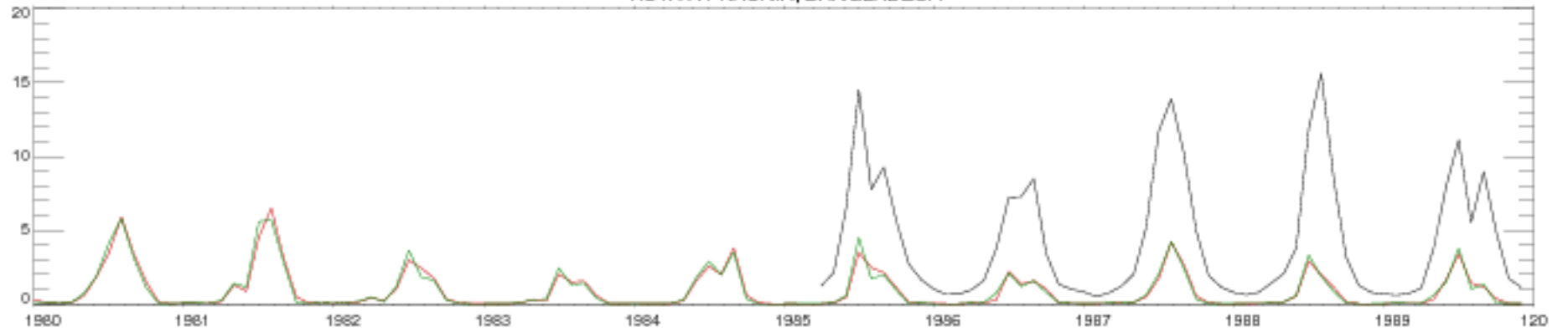
TISTA AT KAUNIA, BANGLADESH
