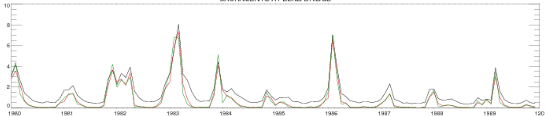
SACRAMENTO AT BEND BRIDGE
