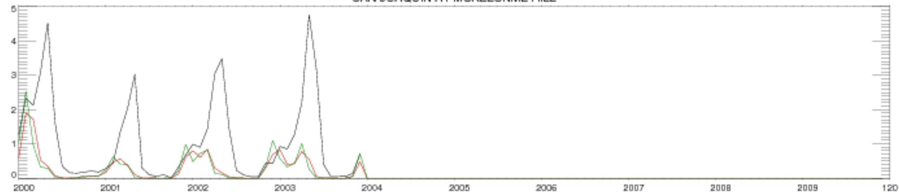
SAN JOAQUIN AT MOKELUNME HILL
