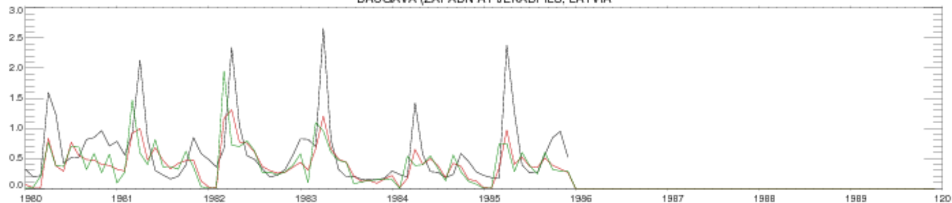
DAUGAVA (ZAPADN AT JEKABPILS, LATVIA)
