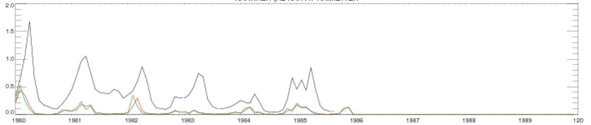
KARKHEH (AL KAR AT HAMIDIYEH)
