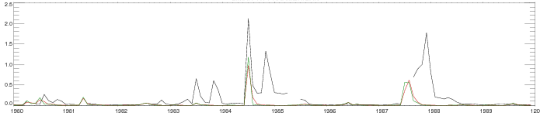
LIMAR AT PANAMERICAN
