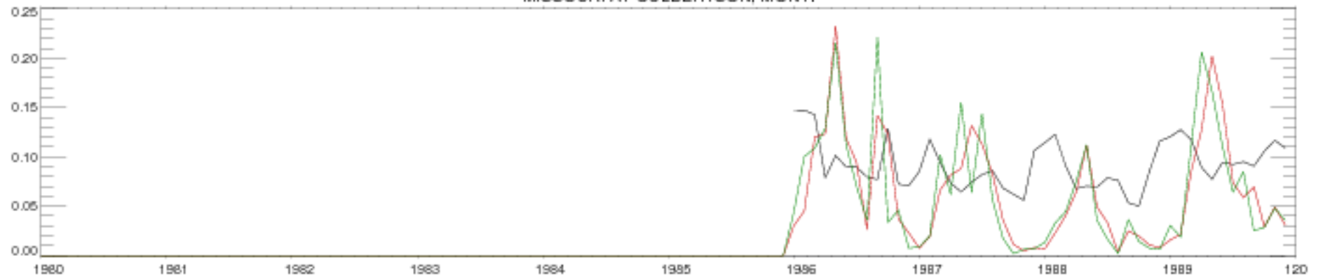
MISSOURI AT CULBERTSON, MONT.
