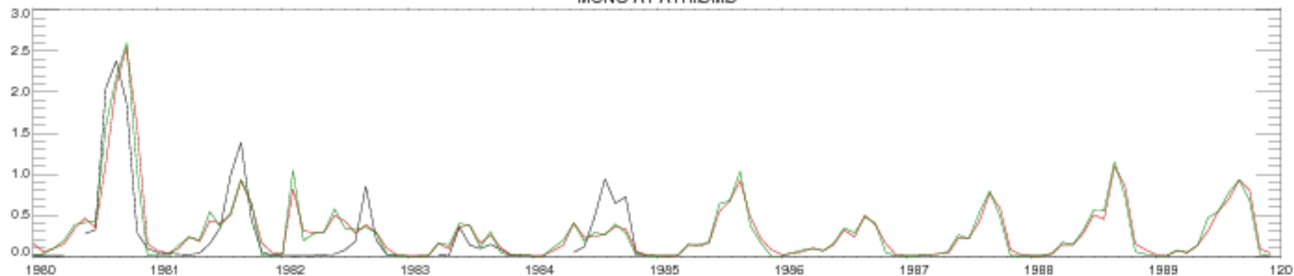
MONO AT ATHIØMØ
