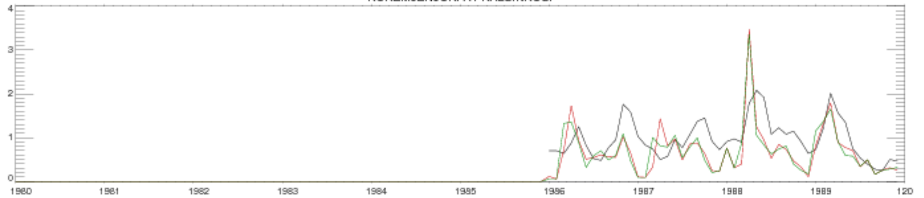
KOKEMJENJOKI AT KALSINKOSI
