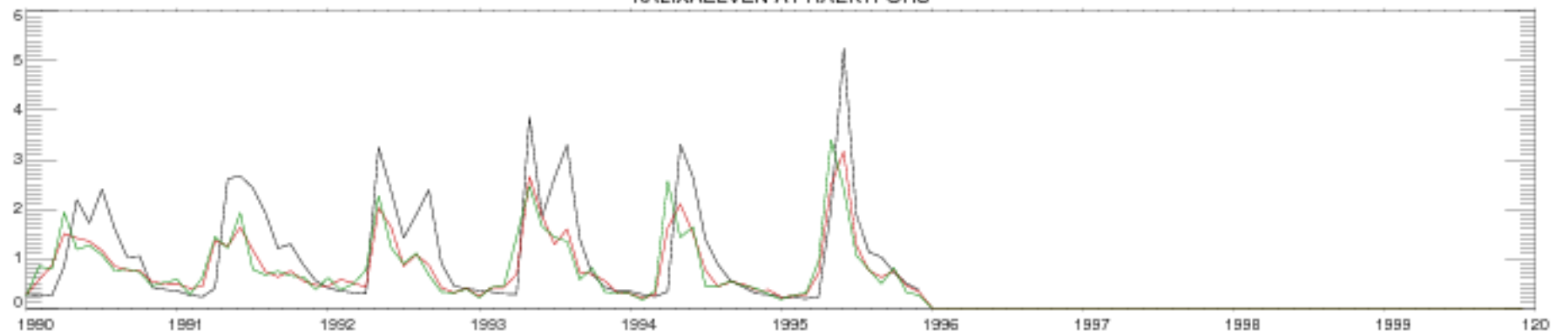
KALIXAELVEN AT RAEKTFORS
