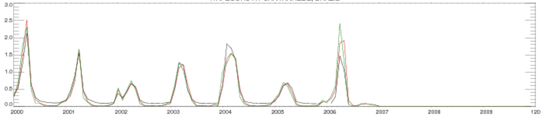
ITAPECURU AT CANTANHEDE, BRAZIL
