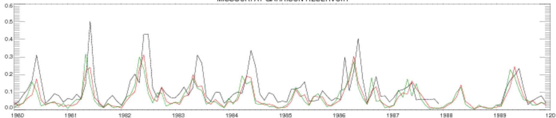
MISSOURI AT GARRISON RESERVOIR
