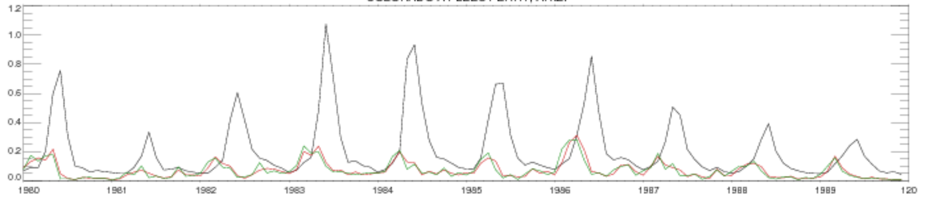
COLORADO AT LEES FERRY, ARIZ.
