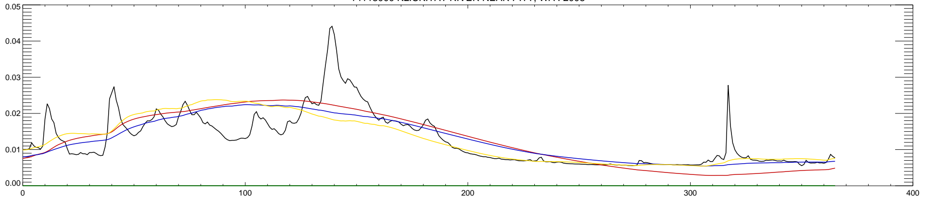
14113000 KLUICKITAT RIVER NEAR PITT, WA : 2009
