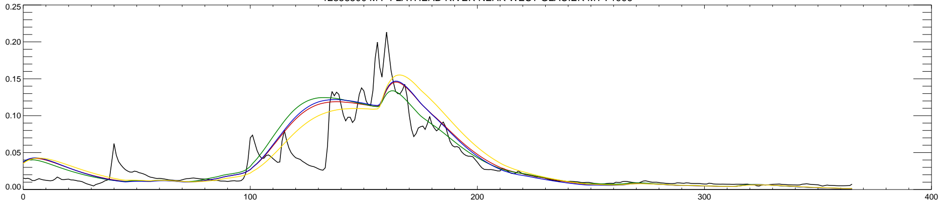
12358500 M F FLATHEAD RIVER NEAR WEST GLACIER MT : 1997
