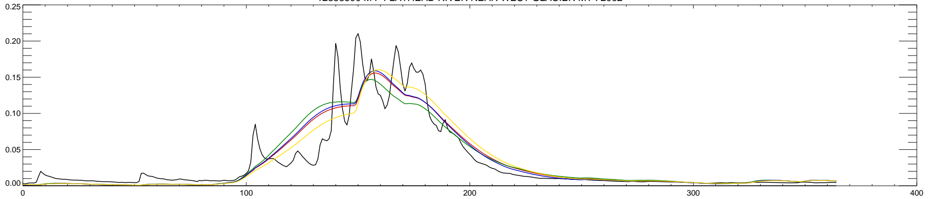
12358500 M F FLATHEAD RIVER NEAR WEST GLACIER MT : 2003
