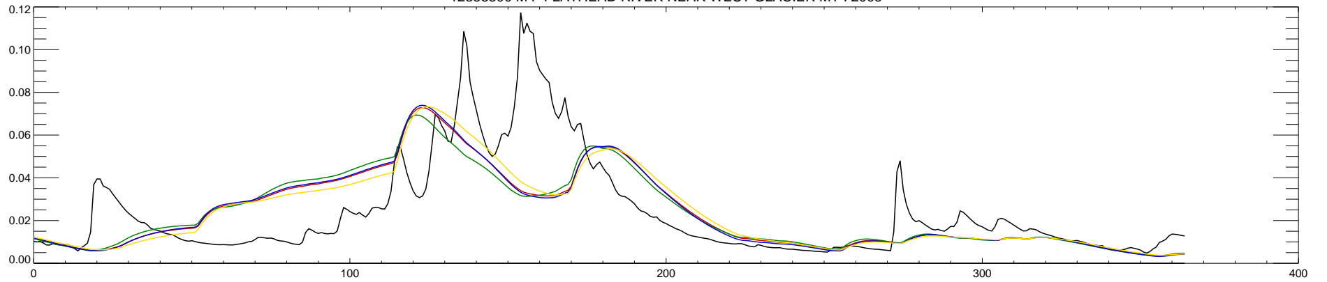
12358500 M F FLATHEAD RIVER NEAR WEST GLACIER MT : 2006
