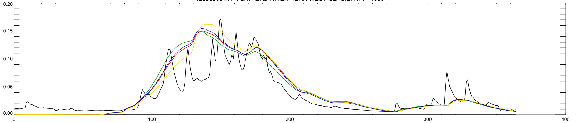
12358500 M F FLATHEAD RIVER NEAR WEST GLACIER MT : 1991
