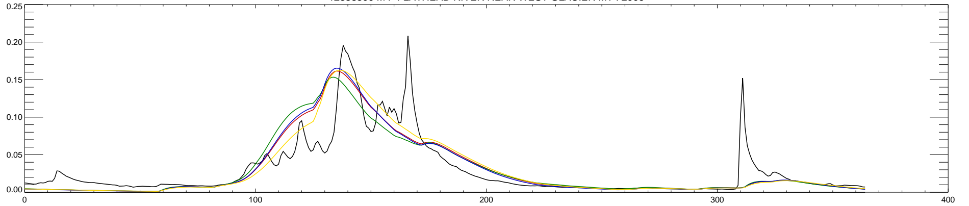
12358500 M F FLATHEAD RIVER NEAR WEST GLACIER MT : 2007
