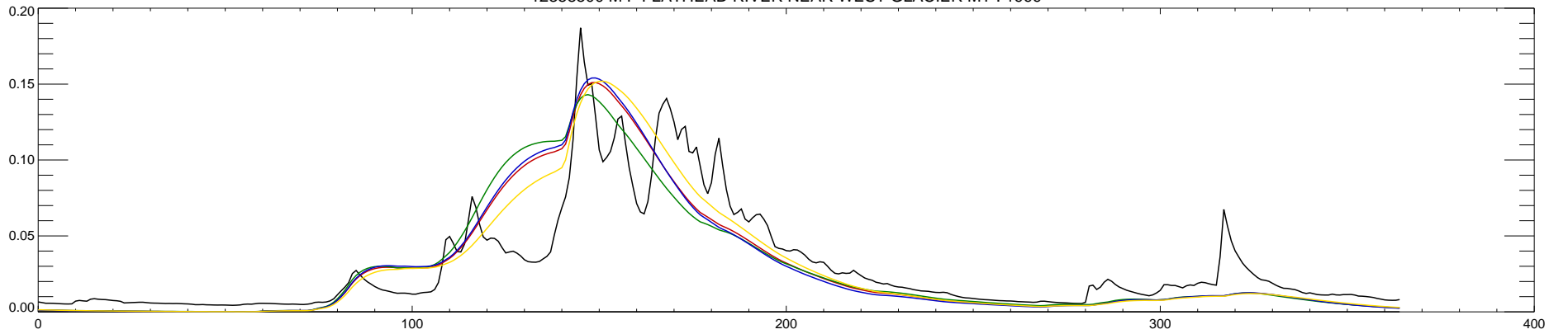
12358500 M F FLATHEAD RIVER NEAR WEST GLACIER MT : 2000
