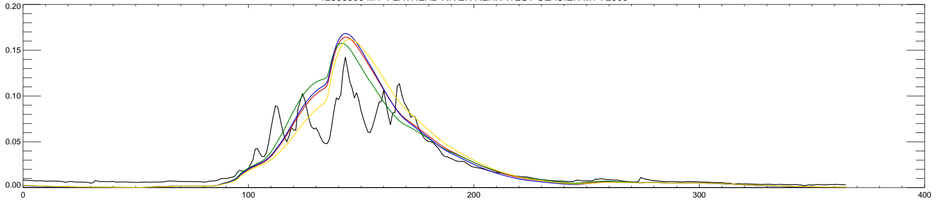
12358500 M F FLATHEAD RIVER NEAR WEST GLACIER MT : 2001
