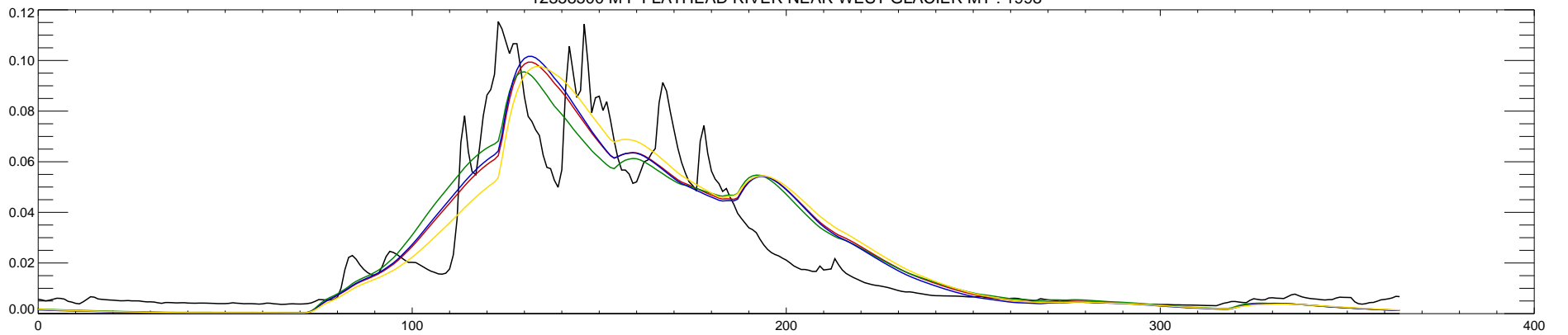
12358500 M F FLATHEAD RIVER NEAR WEST GLACIER MT : 1998
