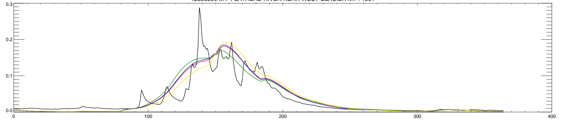
12358500 M F FLATHEAD RIVER NEAR WEST GLACIER MT : 1992
