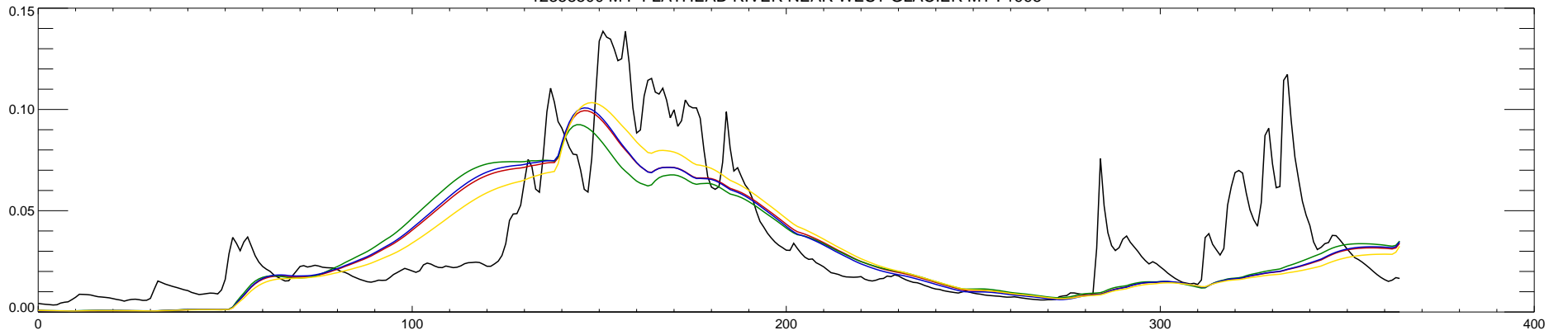
12358500 M F FLATHEAD RIVER NEAR WEST GLACIER MT : 1995
