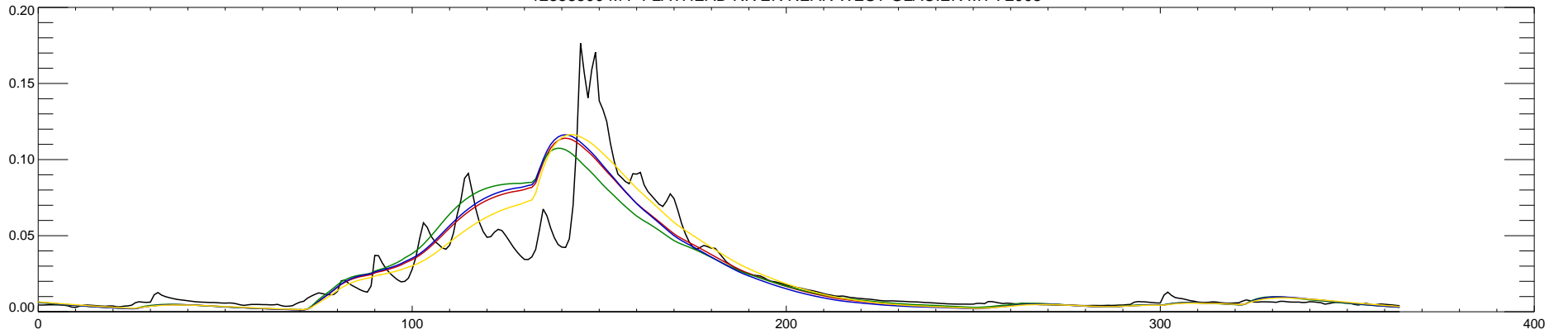
12358500 M F FLATHEAD RIVER NEAR WEST GLACIER MT : 2004
