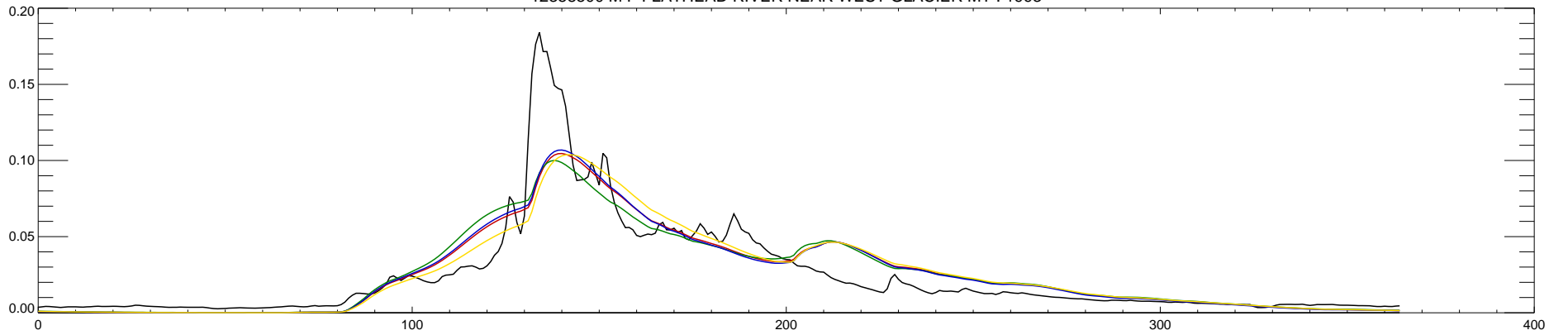
12358500 M F FLATHEAD RIVER NEAR WEST GLACIER MT : 1994
