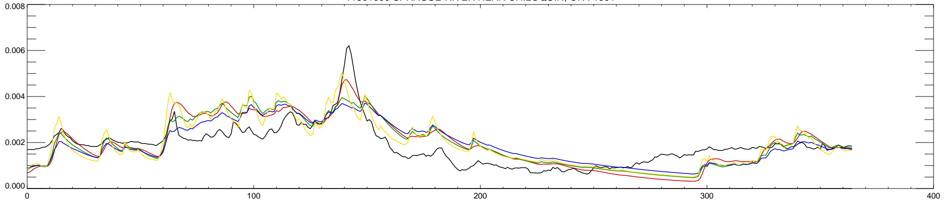
11501000 SPRAGUE RIVER NEAR CHILOQUIN, OR : 1992
