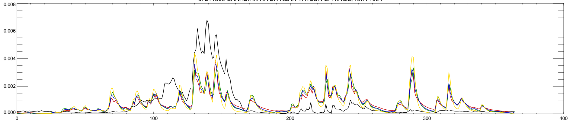
07211500 CANADIAN RIVER NEAR TAYLOR SPRINGS, NM : 1995
