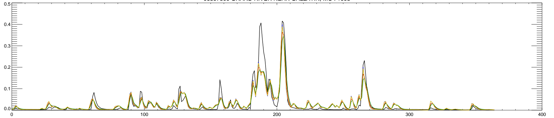
06897500 GRAND RIVER NEAR GALLATIN, MO : 1994
