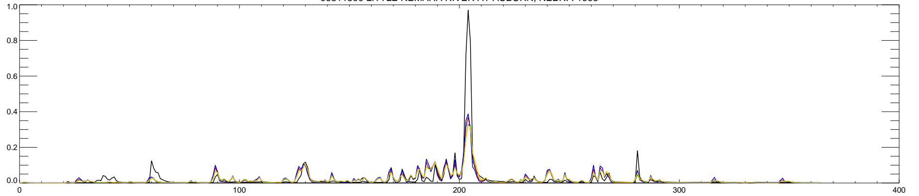
06811500 LITTLE NEMAHA RIVER AT AUBURN, NEBR. : 1994
