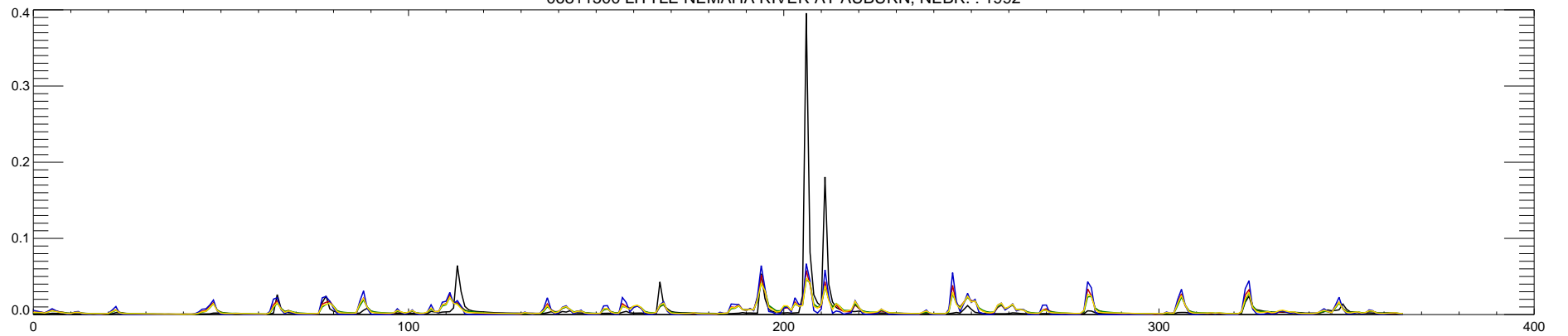
06811500 LITTLE NEMAHA RIVER AT AUBURN, NEBR. : 1992
