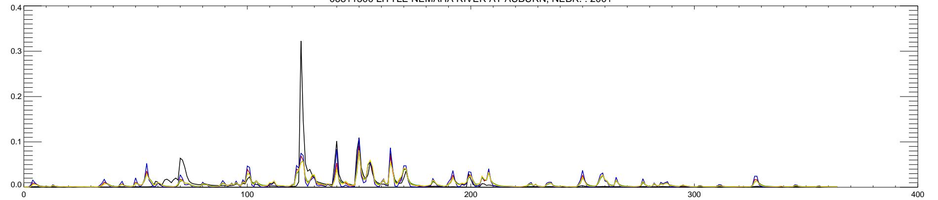
06811500 LITTLE NEMAHA RIVER AT AUBURN, NEBR. : 2001
