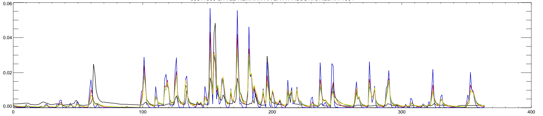
06811500 LITTLE NEMAHA RIVER AT AUBURN, NEBR. : 1995
