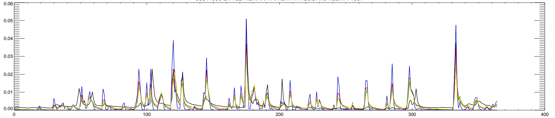
06811500 LITTLE NEMAHA RIVER AT AUBURN, NEBR. : 1998
