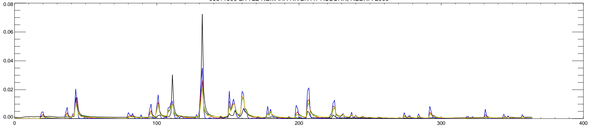
06811500 LITTLE NEMAHA RIVER AT AUBURN, NEBR. : 2006
