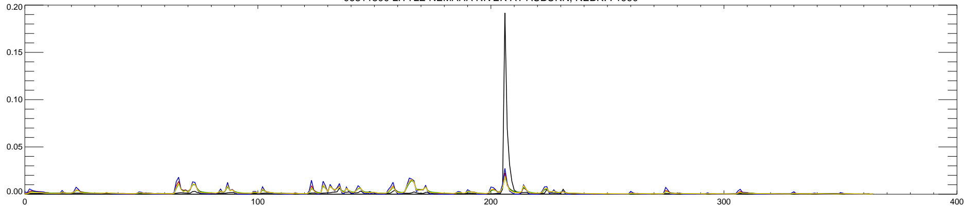
06811500 LITTLE NEMAHA RIVER AT AUBURN, NEBR. : 1991
