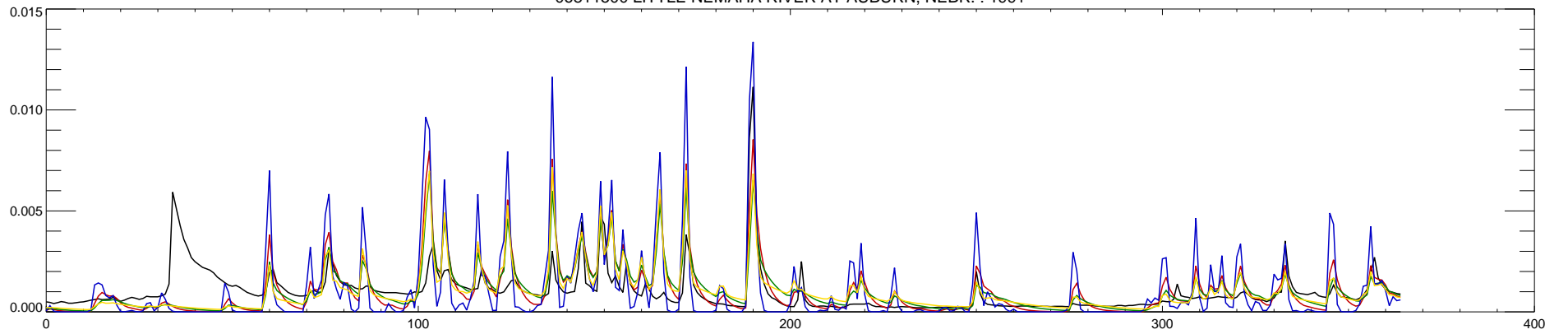
06811500 LITTLE NEMAHA RIVER AT AUBURN, NEBR. : 1992
