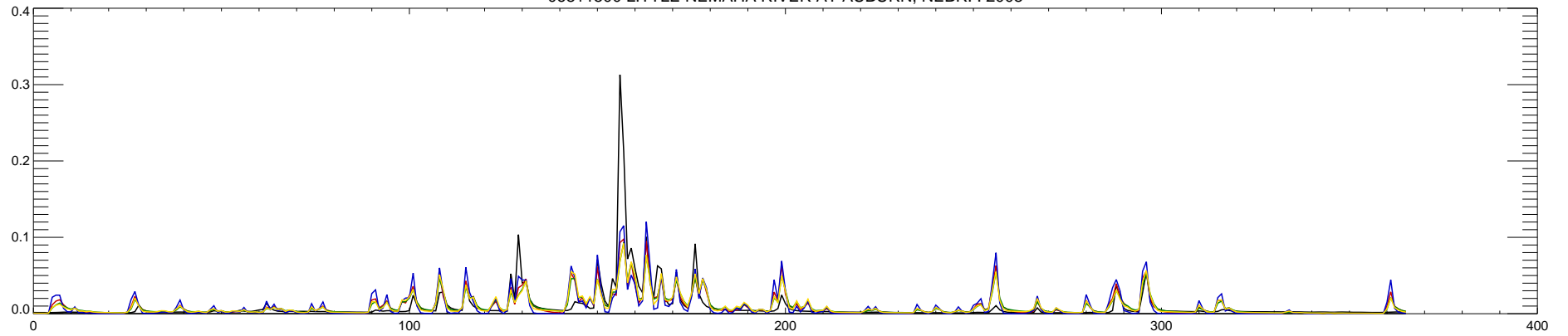
06811500 LITTLE NEMAHA RIVER AT AUBURN, NEBR. : 2009
