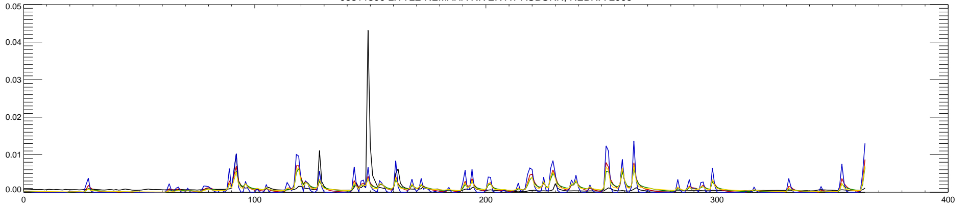
06811500 LITTLE NEMAHA RIVER AT AUBURN, NEBR. : 2007
