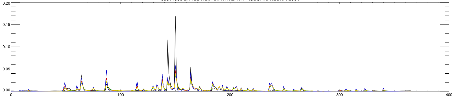
06811500 LITTLE NEMAHA RIVER AT AUBURN, NEBR. : 2004
