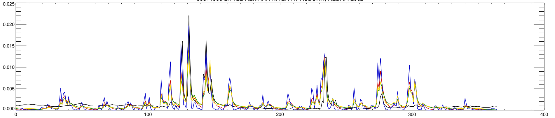
06811500 LITTLE NEMAHA RIVER AT AUBURN, NEBR. : 2003
