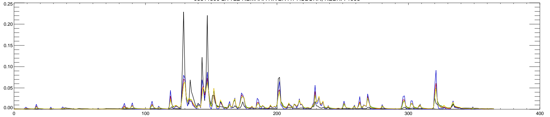
06811500 LITTLE NEMAHA RIVER AT AUBURN, NEBR. : 1997
