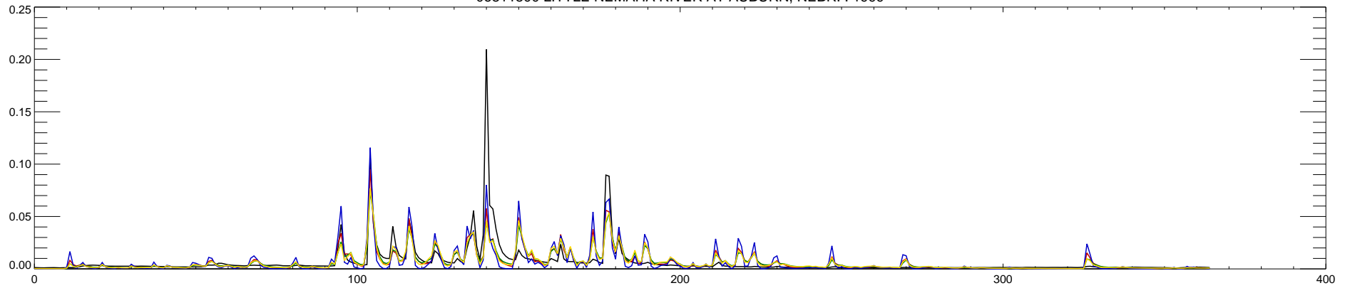
06811500 LITTLE NEMAHA RIVER AT AUBURN, NEBR. : 2000
