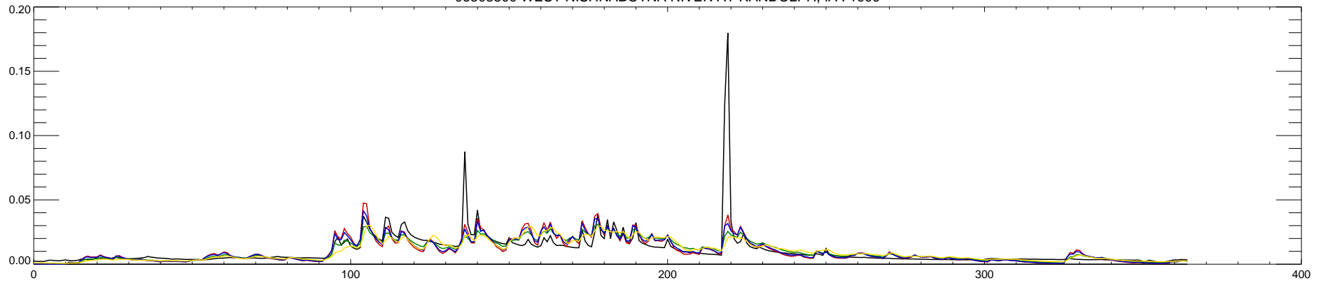
06808500 WEST NISHNABOTNA RIVER AT RANDOLPH, IA : 2000
