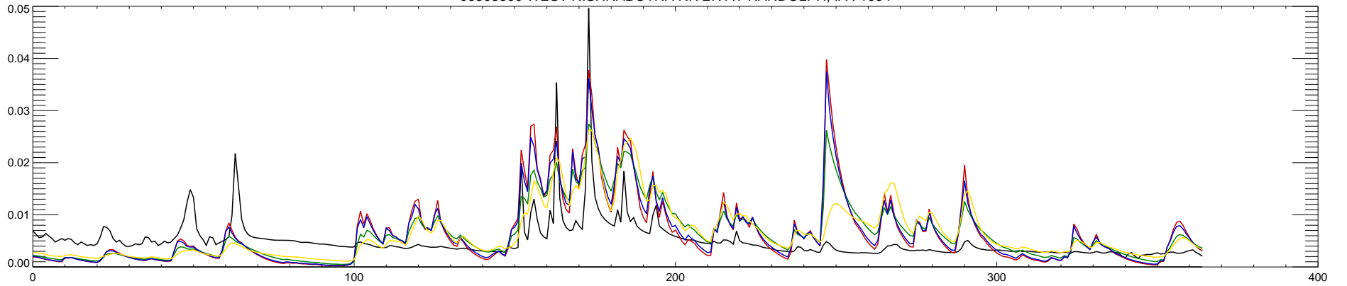
06808500 WEST NISHNABOTNA RIVER AT RANDOLPH, IA : 1995
