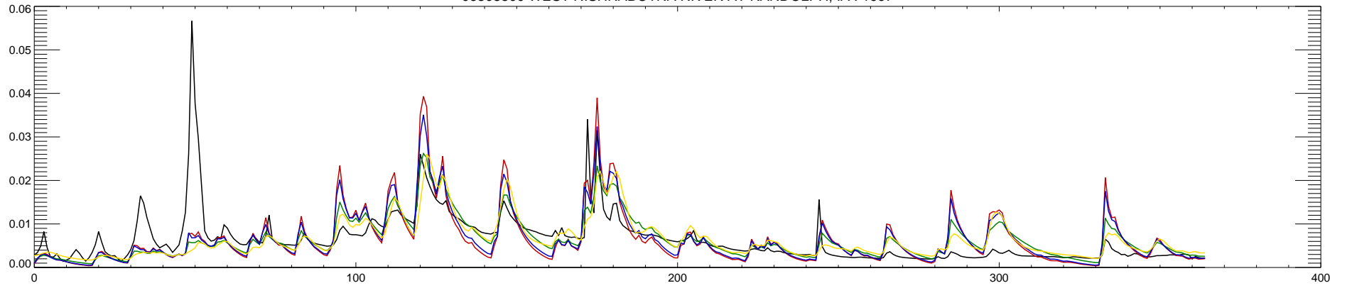
06808500 WEST NISHNABOTNA RIVER AT RANDOLPH, IA : 1998
