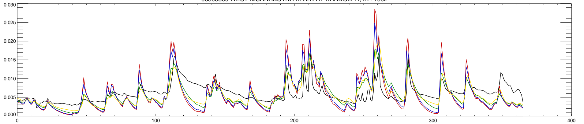
06808500 WEST NISHNABOTNA RIVER AT RANDOLPH, IA : 1992
