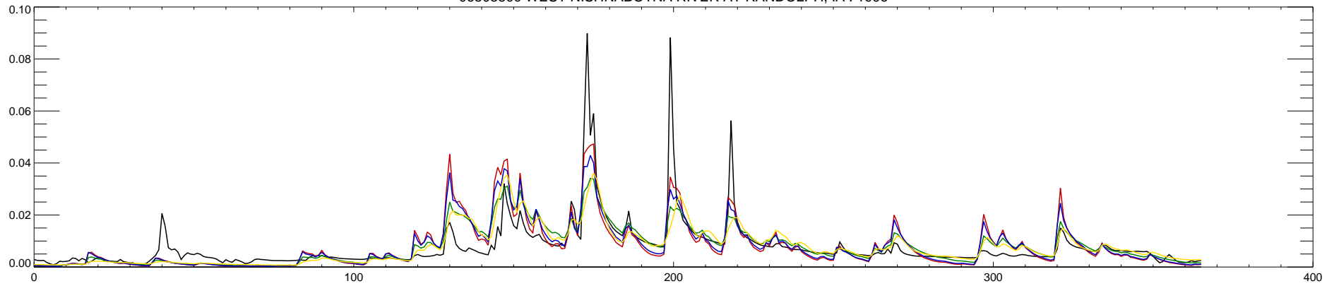
06808500 WEST NISHNABOTNA RIVER AT RANDOLPH, IA : 1997
