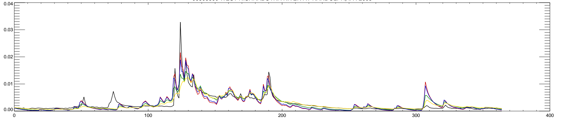
06808500 WEST NISHNABOTNA RIVER AT RANDOLPH, IA : 2004
