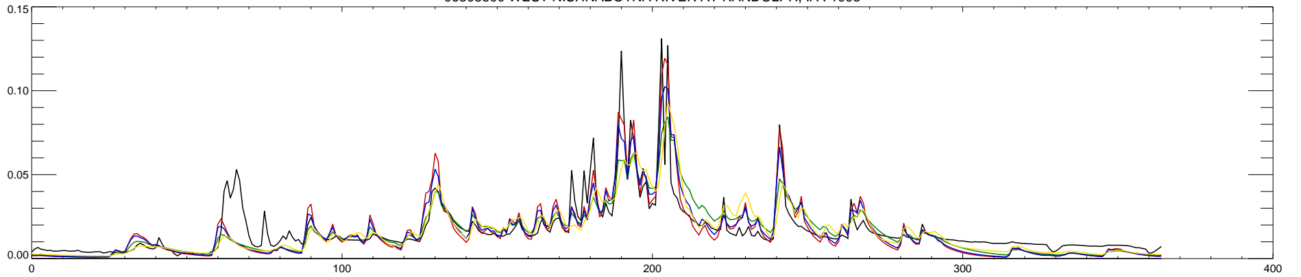
06808500 WEST NISHNABOTNA RIVER AT RANDOLPH, IA : 1994
