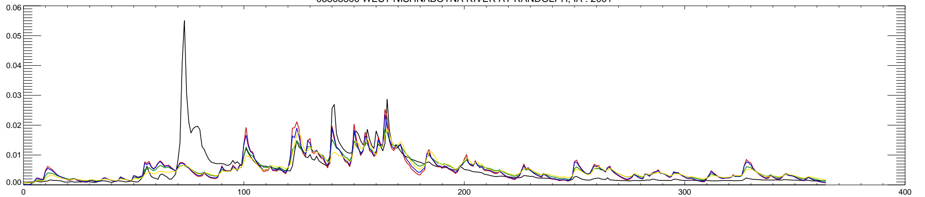
06808500 WEST NISHNABOTNA RIVER AT RANDOLPH, IA : 2001
