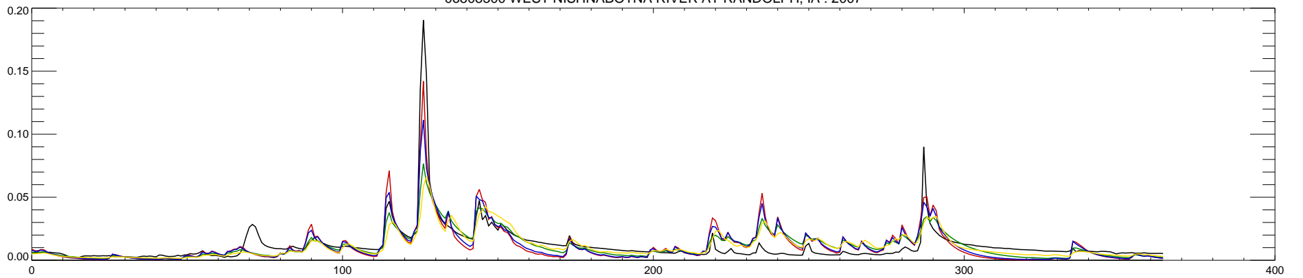
06808500 WEST NISHNABOTNA RIVER AT RANDOLPH, IA : 2007
