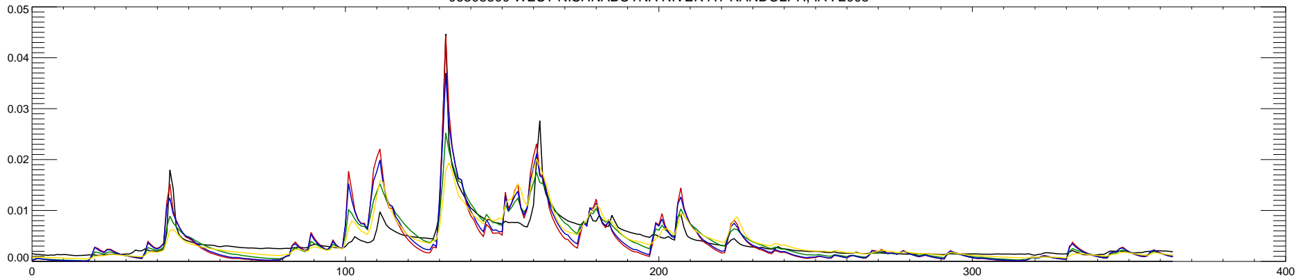
06808500 WEST NISHNABOTNA RIVER AT RANDOLPH, IA : 2006
