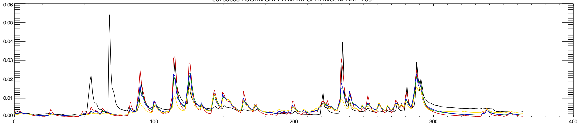
06799500 LOGAN CREEK NEAR UEHLING, NEBR. : 2007
