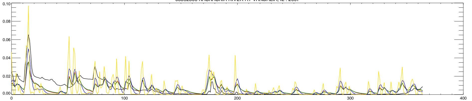
05592500 KASKASKIA RIVER AT VANDALIA, IL : 2007
