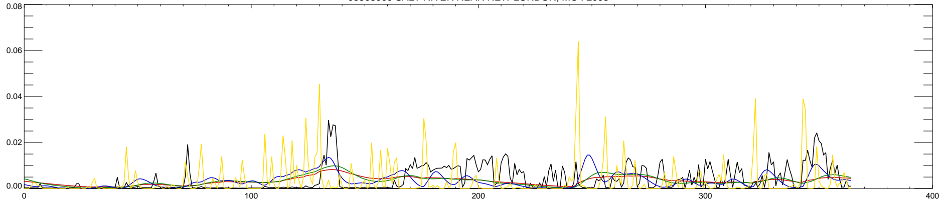
05508000 SALT RIVER NEAR NEW LONDON, MO : 2004
