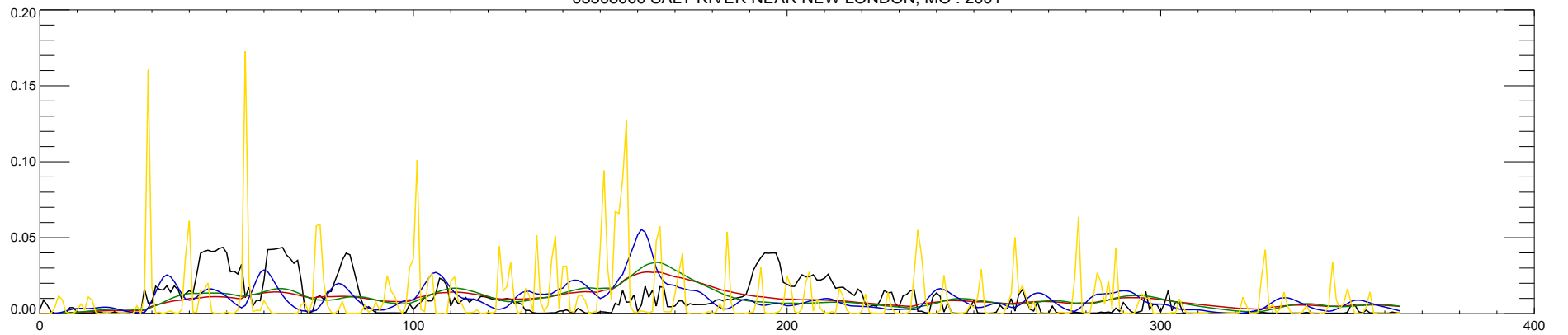
05508000 SALT RIVER NEAR NEW LONDON, MO : 2001
