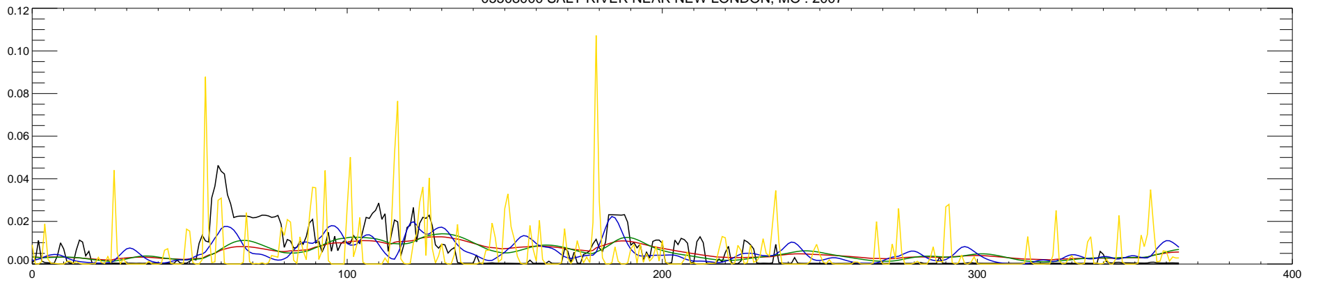
05508000 SALT RIVER NEAR NEW LONDON, MO : 2007
