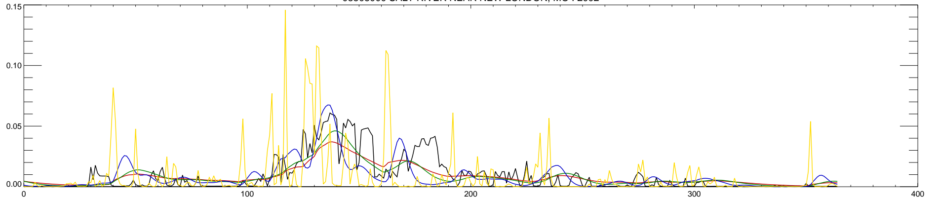
05508000 SALT RIVER NEAR NEW LONDON, MO : 2003
