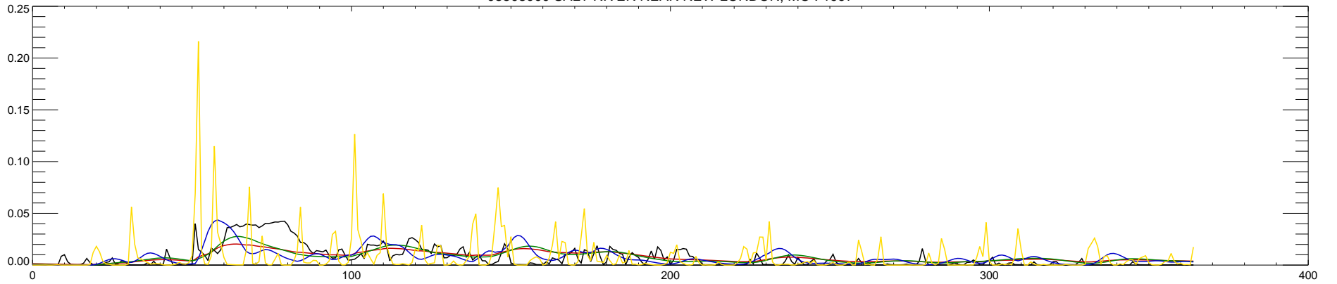
05508000 SALT RIVER NEAR NEW LONDON, MO : 1998
