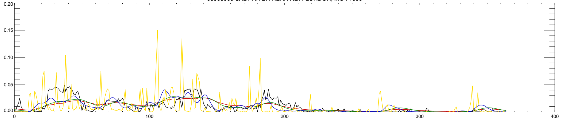
05508000 SALT RIVER NEAR NEW LONDON, MO : 2000
