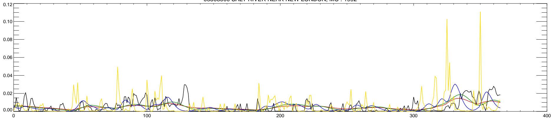
05508000 SALT RIVER NEAR NEW LONDON, MO : 1992
