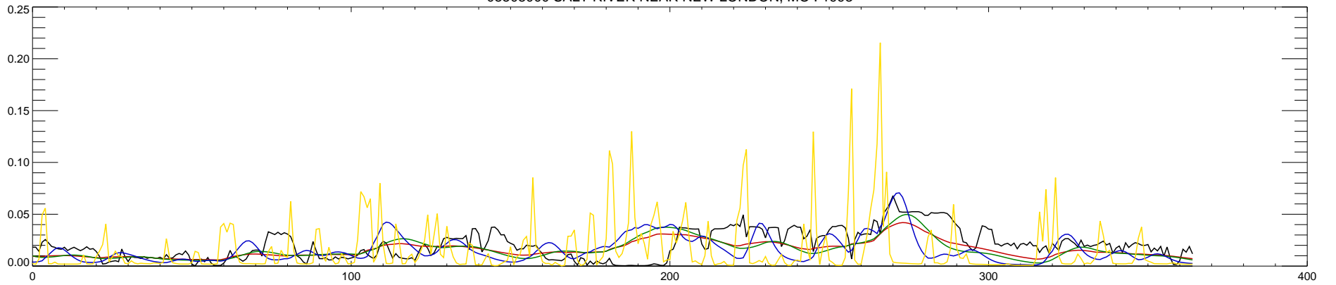
05508000 SALT RIVER NEAR NEW LONDON, MO : 1994
