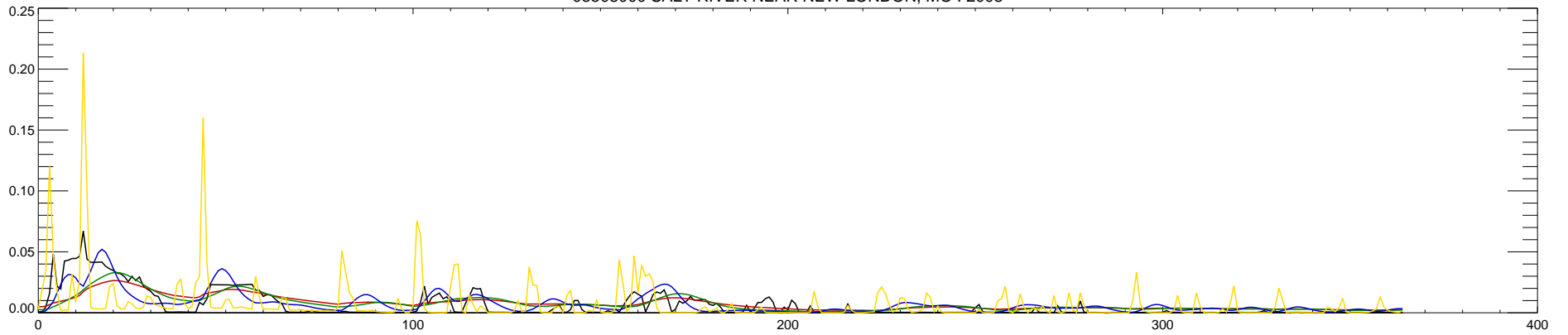
05508000 SALT RIVER NEAR NEW LONDON, MO : 2006
