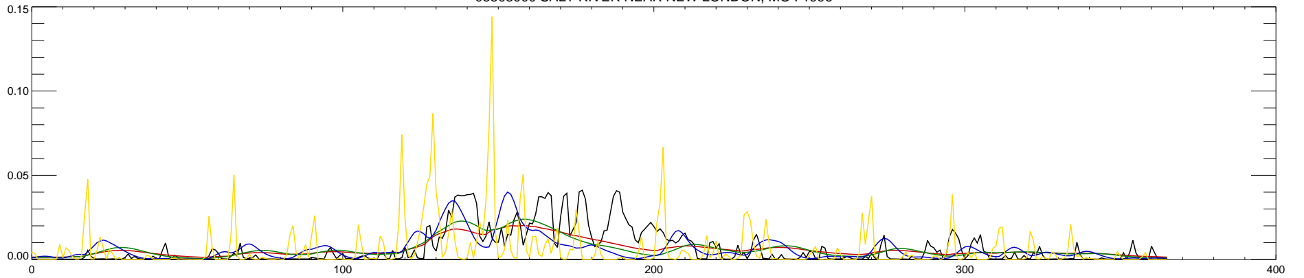
05508000 SALT RIVER NEAR NEW LONDON, MO : 1997
