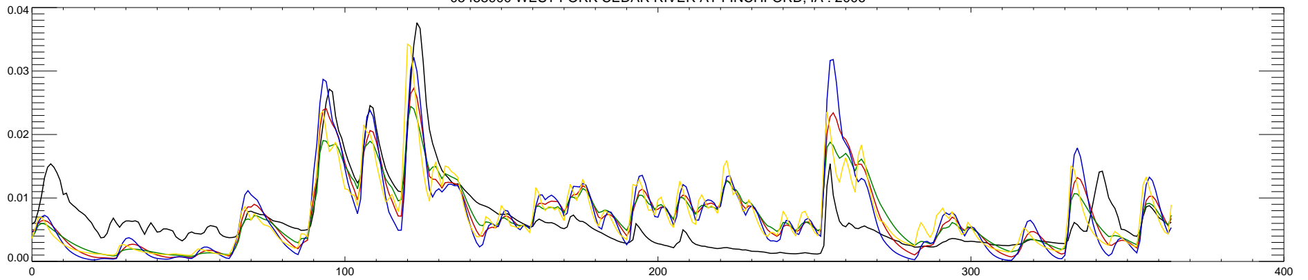
05458900 WEST FORK CEDAR RIVER AT FINCHFORD, IA : 2007
