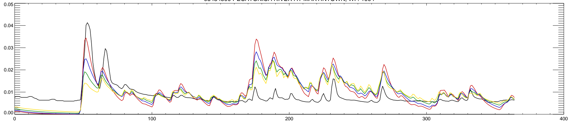
05434500 PECATONICA RIVER AT MARTINTOWN, WI : 1995
