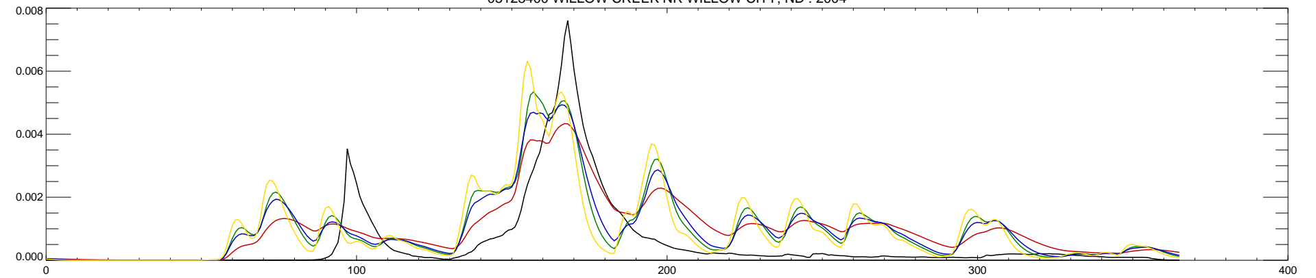
05123400 WILLOW CREEK NR WILLOW CITY, ND : 2004
