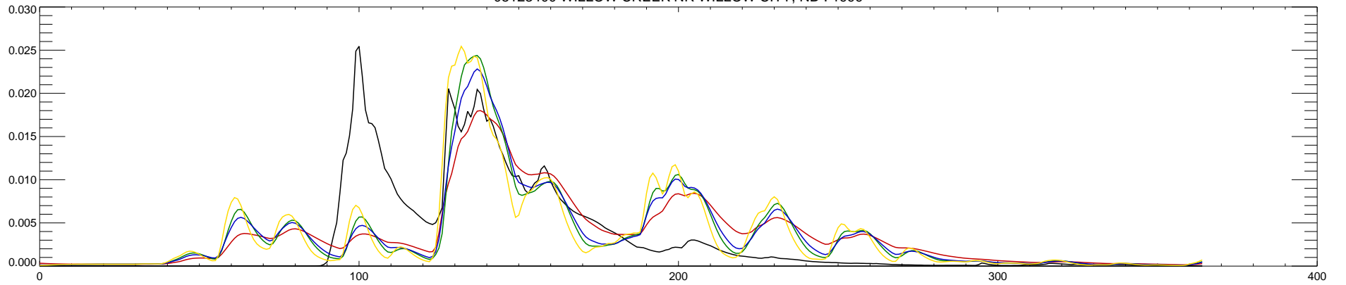
05123400 WILLOW CREEK NR WILLOW CITY, ND : 2000
