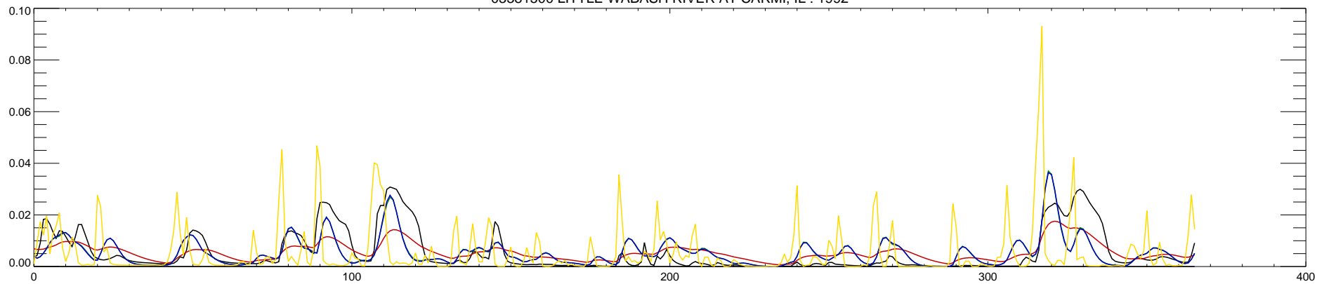
03381500 LITTLE WABASH RIVER AT CARM, IL : 1992
