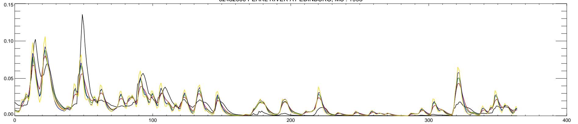
02482000 PEARL RIVER AT EDINBURG, MS : 1994
