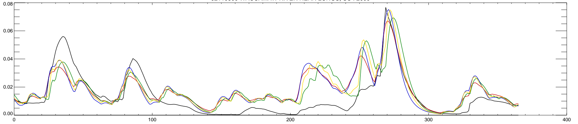
02110500 WACCAMAW RIVER NEAR LONGS, SC : 2001
