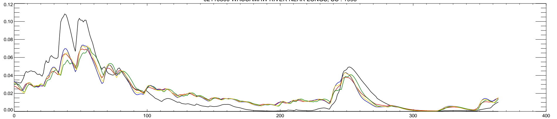
02110500 WACCAMAW RIVER NEAR LONGS, SC : 1998
