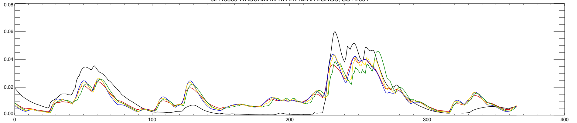
02110500 WACCAMAW RIVER NEAR LONGS, SC : 2004
