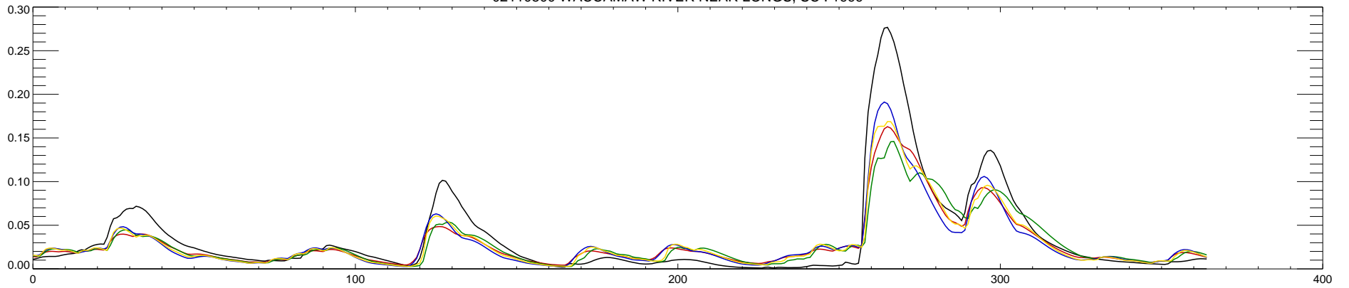
02110500 WACCAMAW RIVER NEAR LONGS, SC : 2000
