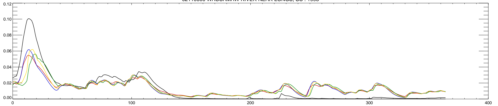
02110500 WACCAMAW RIVER NEAR LONGS, SC : 1994
