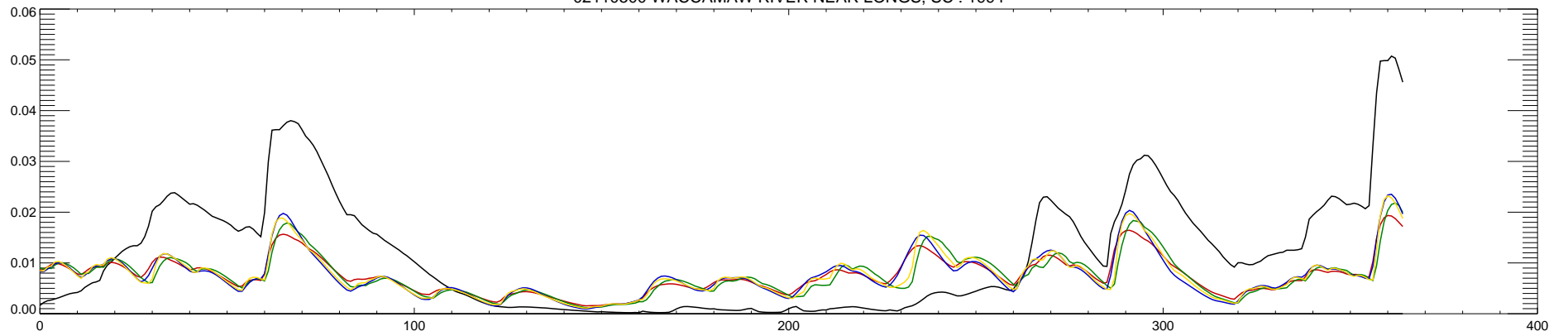
02110500 WACCAMAW RIVER NEAR LONGS, SC : 1995
