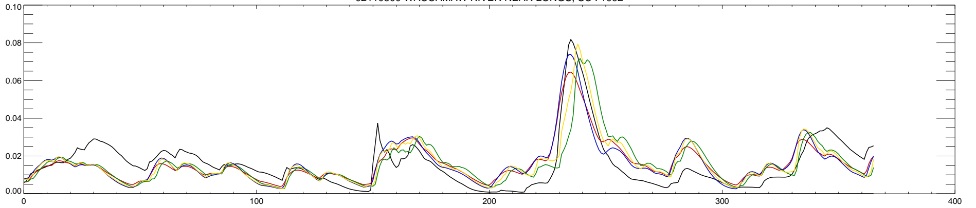
02110500 WACCAMAW RIVER NEAR LONGS, SC : 1992
