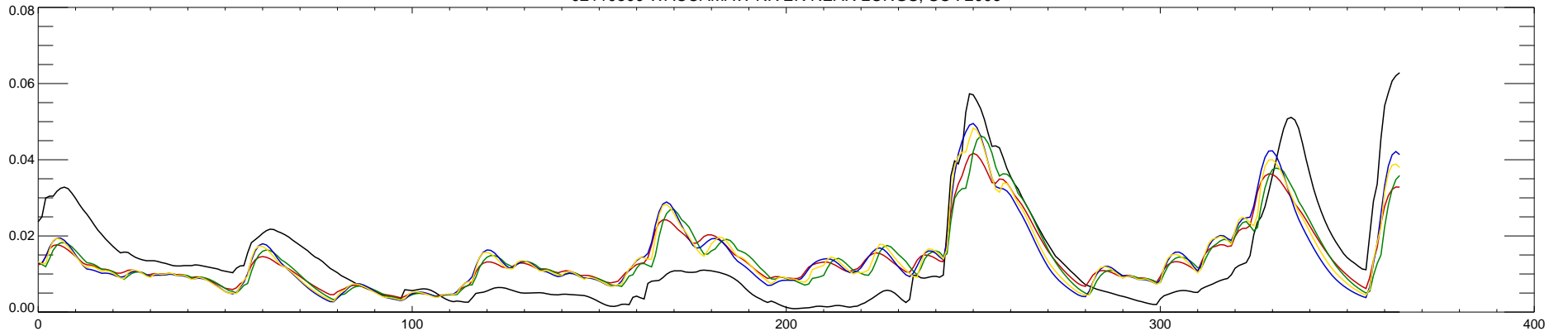
02110500 WACCAMAW RIVER NEAR LONGS, SC : 2007
