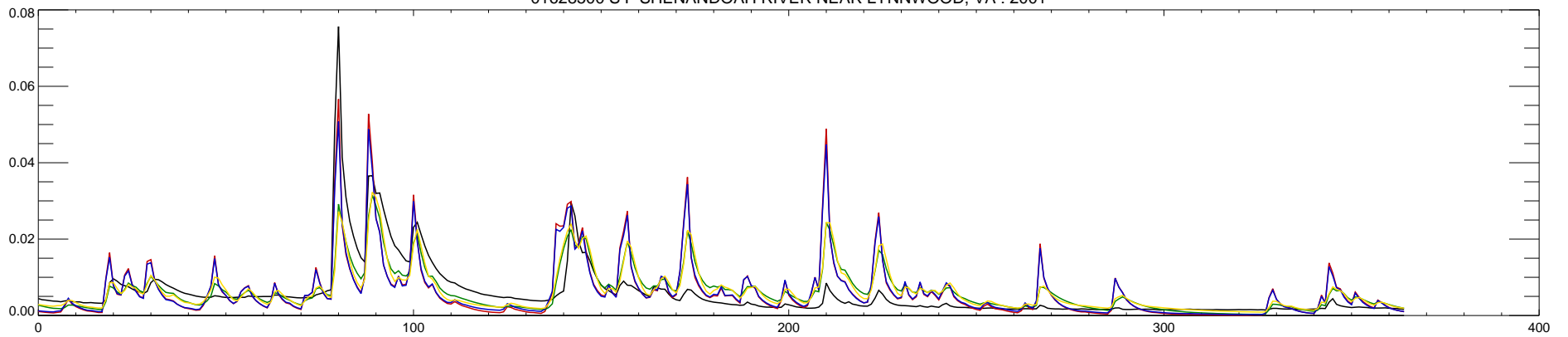
01628500 S F SHENANDOAH RIVER NEAR LYNNWOOD, VA : 2001
