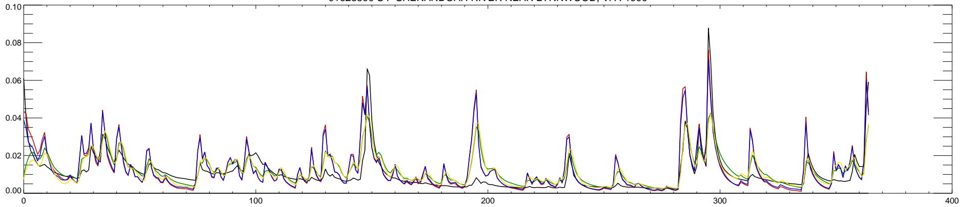
01628500 S F SHENANDOAH RIVER NEAR LYNNWOOD, VA : 1991
