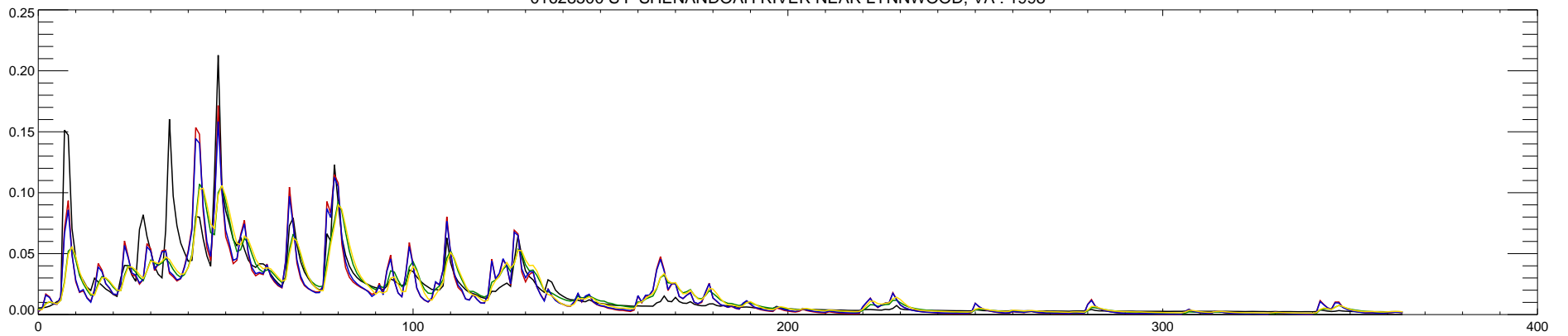
01628500 S F SHENANDOAH RIVER NEAR LYNNWOOD, VA : 1998
