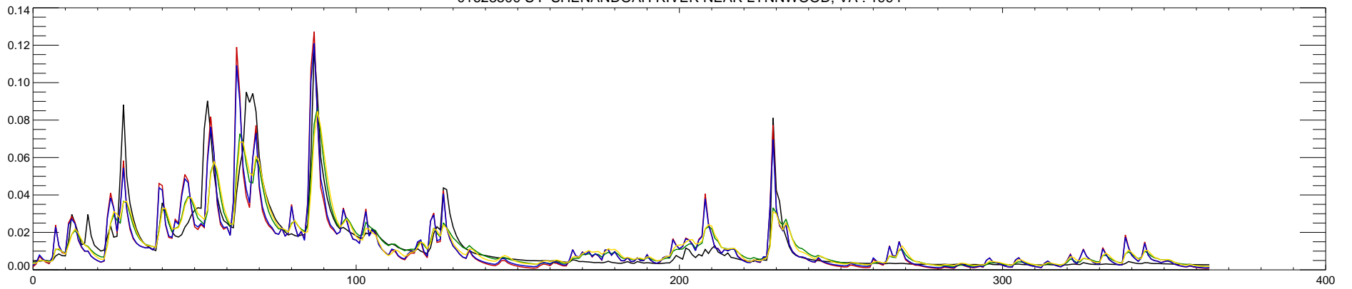
01628500 S F SHENANDOAH RIVER NEAR LYNNWOOD, VA : 1995
