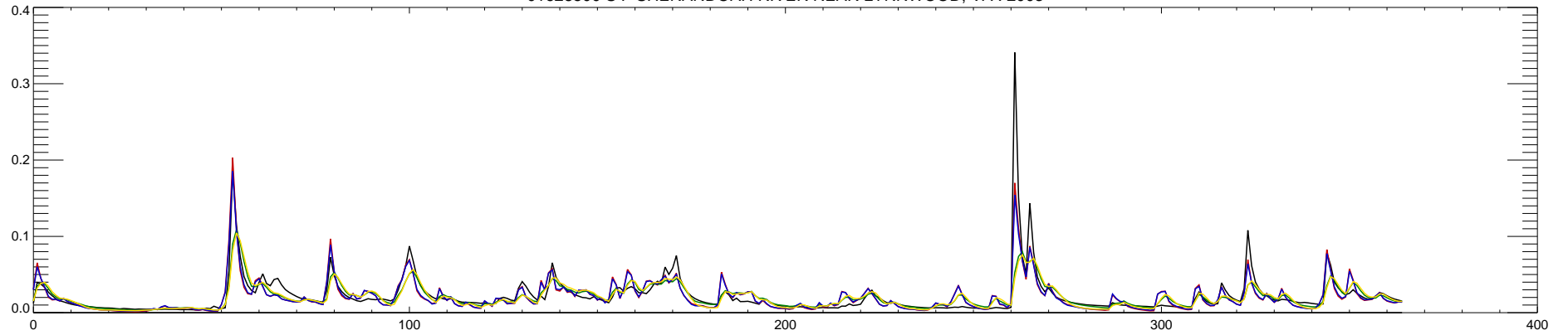
01628500 S F SHENANDOAH RIVER NEAR LYNNWOOD, VA : 2004
