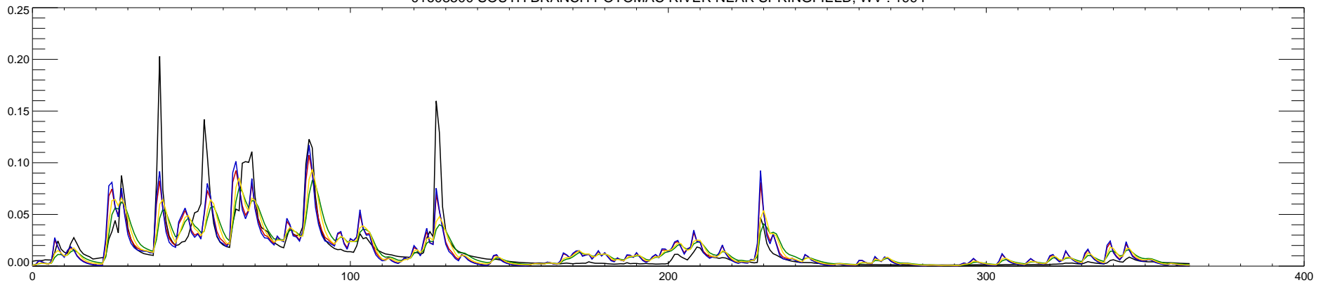
01608500 SOUTH BRANCH POTOMAC RIVER NEAR SPRINGFIELD, WV : 1995
