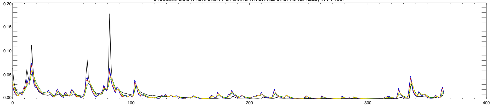
01608500 SOUTH BRANCH POTOMAC RIVER NEAR SPRINGFIELD, WV : 1992
