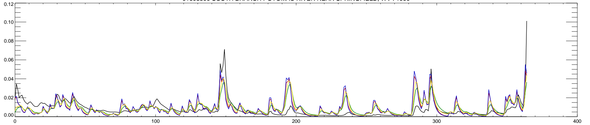
01608500 SOUTH BRANCH POTOMAC RIVER NEAR SPRINGFIELD, WV : 1991
