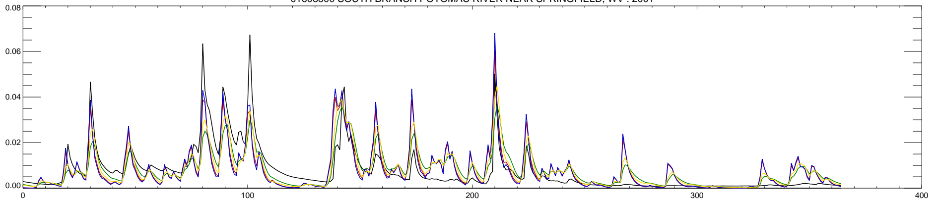
01608500 SOUTH BRANCH POTOMAC RIVER NEAR SPRINGFIELD, WV : 2001
